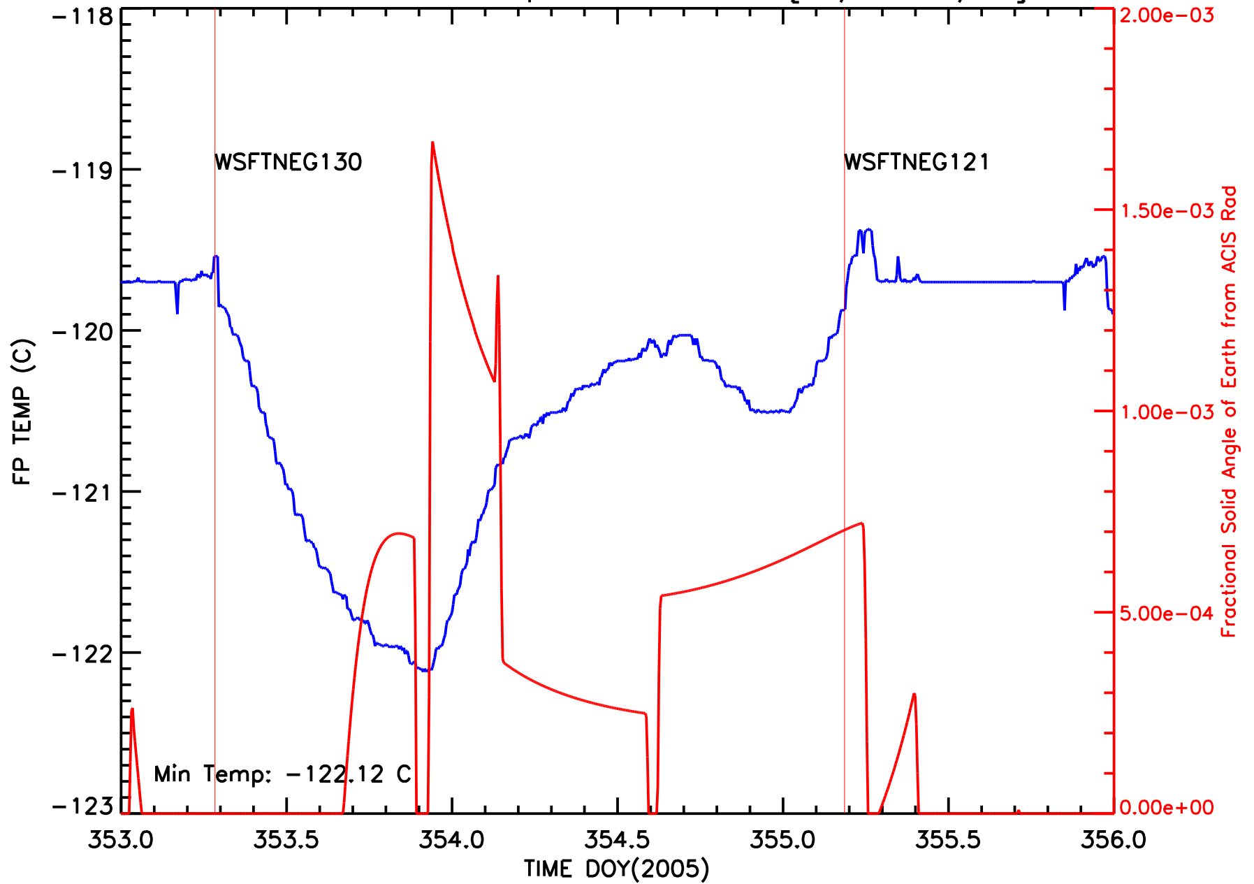
ACIS Focal Plane Temperature vs Time [12/18-22/05]
