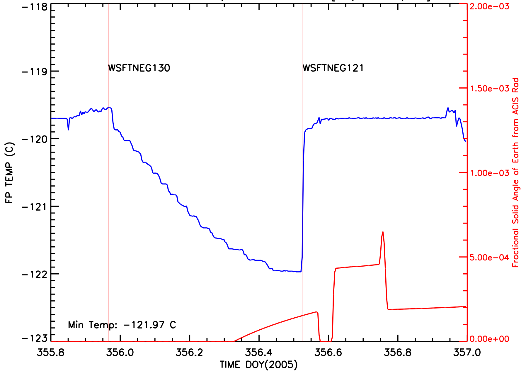
ACIS Focal Plane Temperature vs Time [12/21-23/05]
