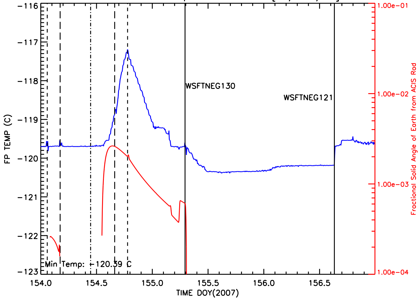
ACIS Focal Plane Temperature vs Time [06/3-7/07]
