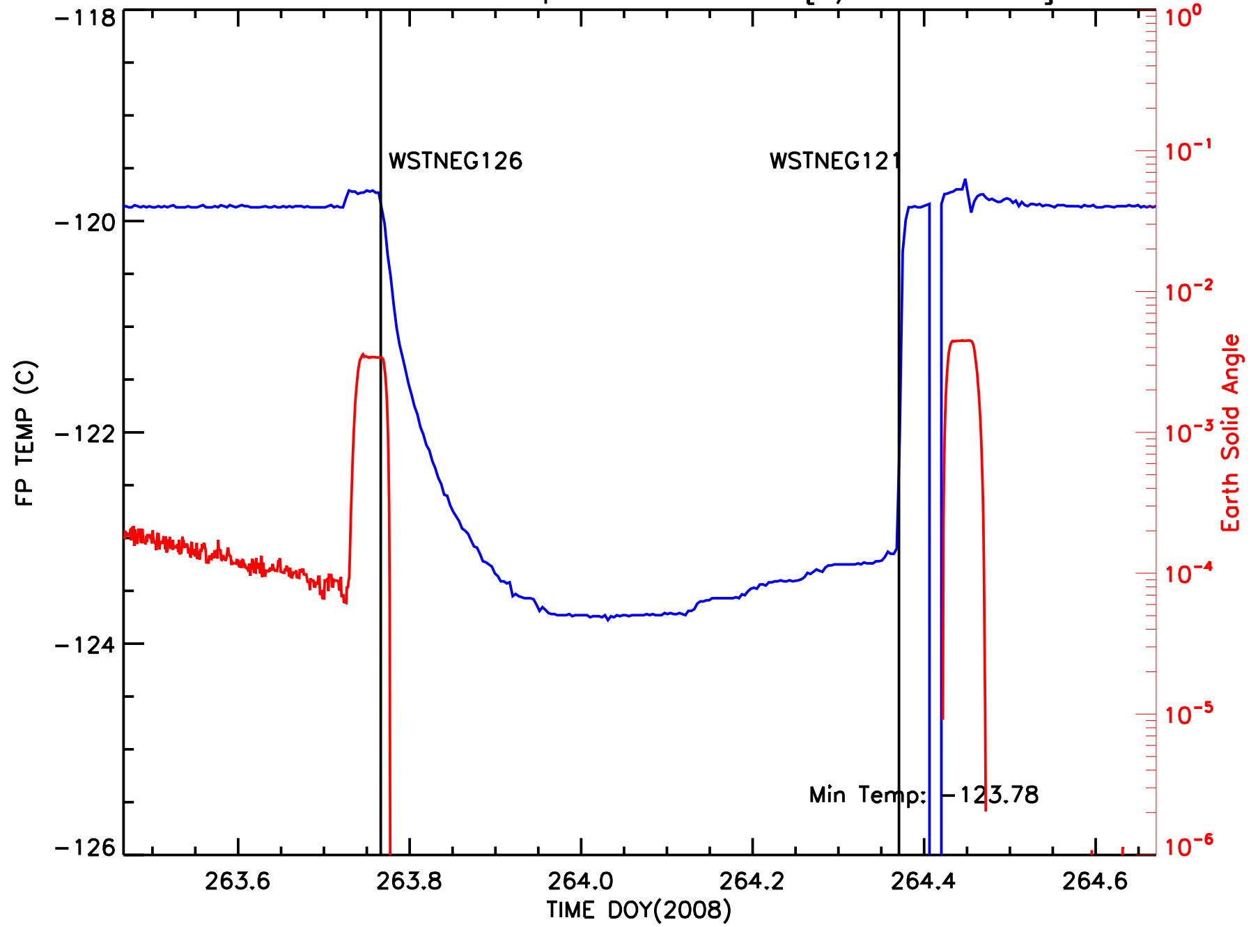
ACIS Focal Plane Temperature vs Time [9/20-21 2008]
