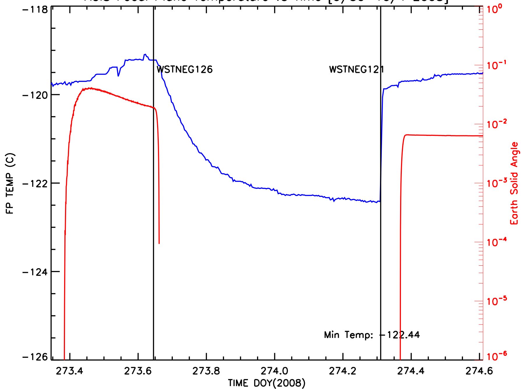
ACIS Focal Plane Temperature vs Time [9/30-10/1 2008]
