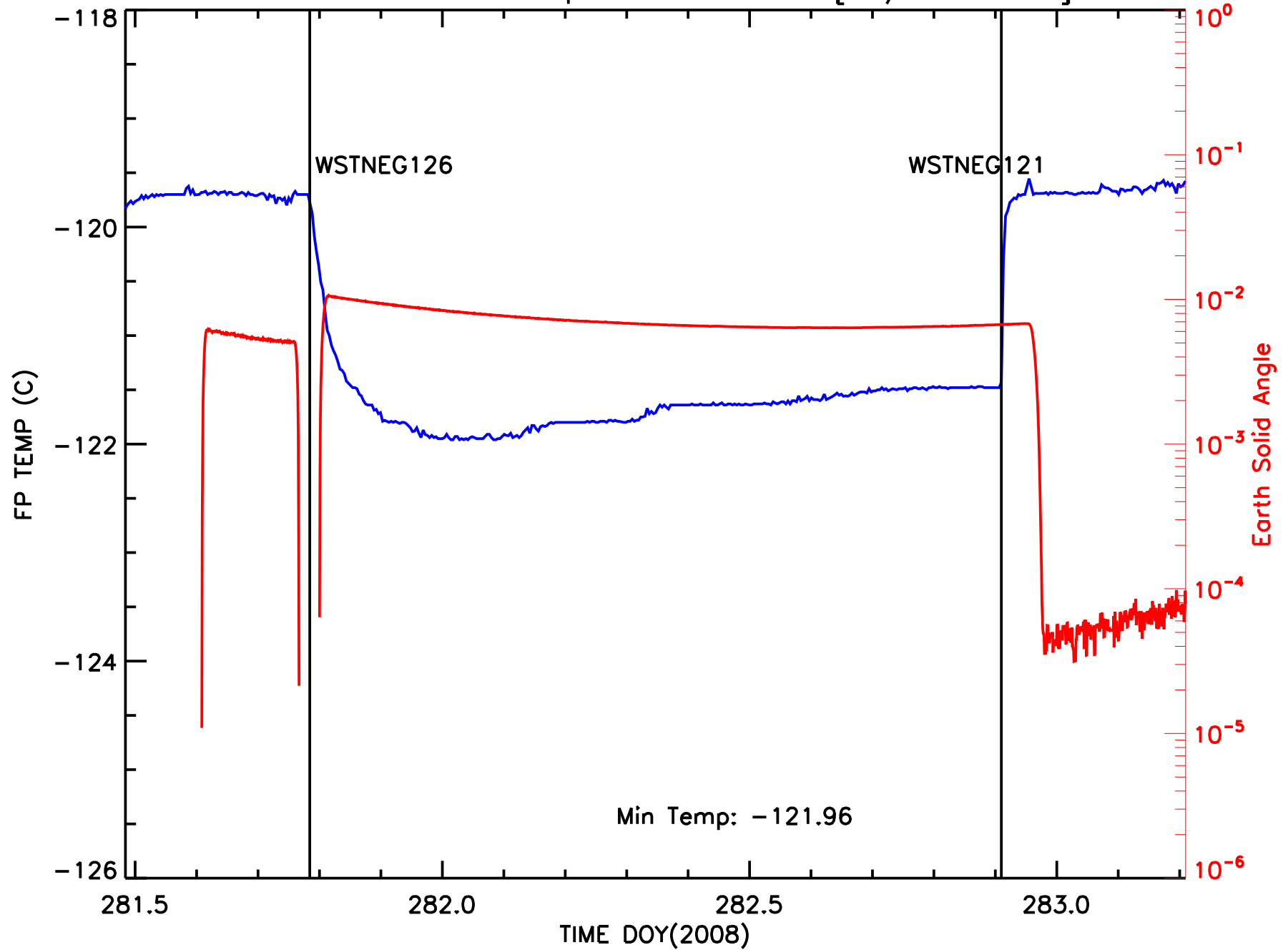
ACIS Focal Plane Temperature vs Time [10/8-9 2008]
