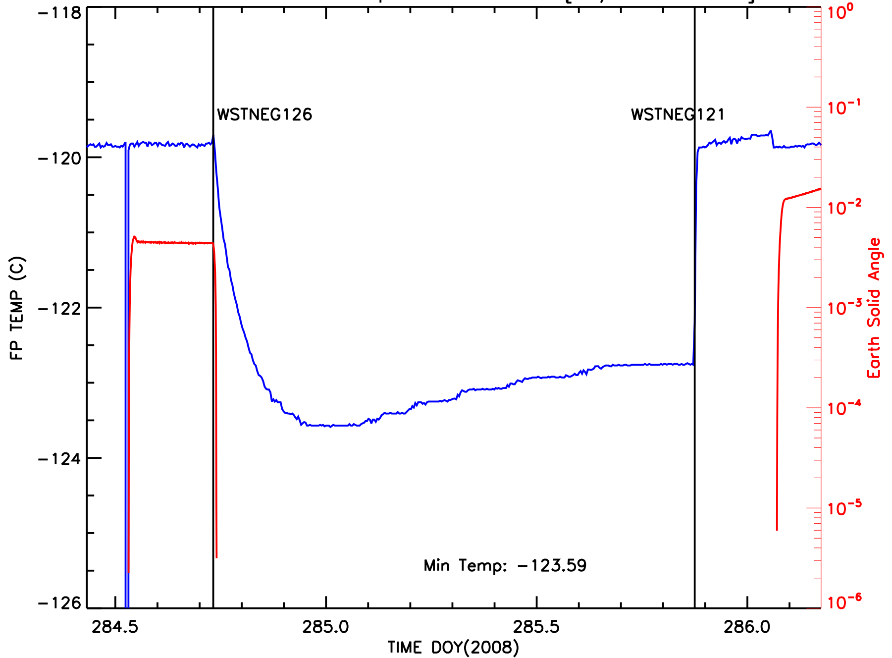
ACIS Focal Plane Temperature vs Time [10/11-12 2008]
