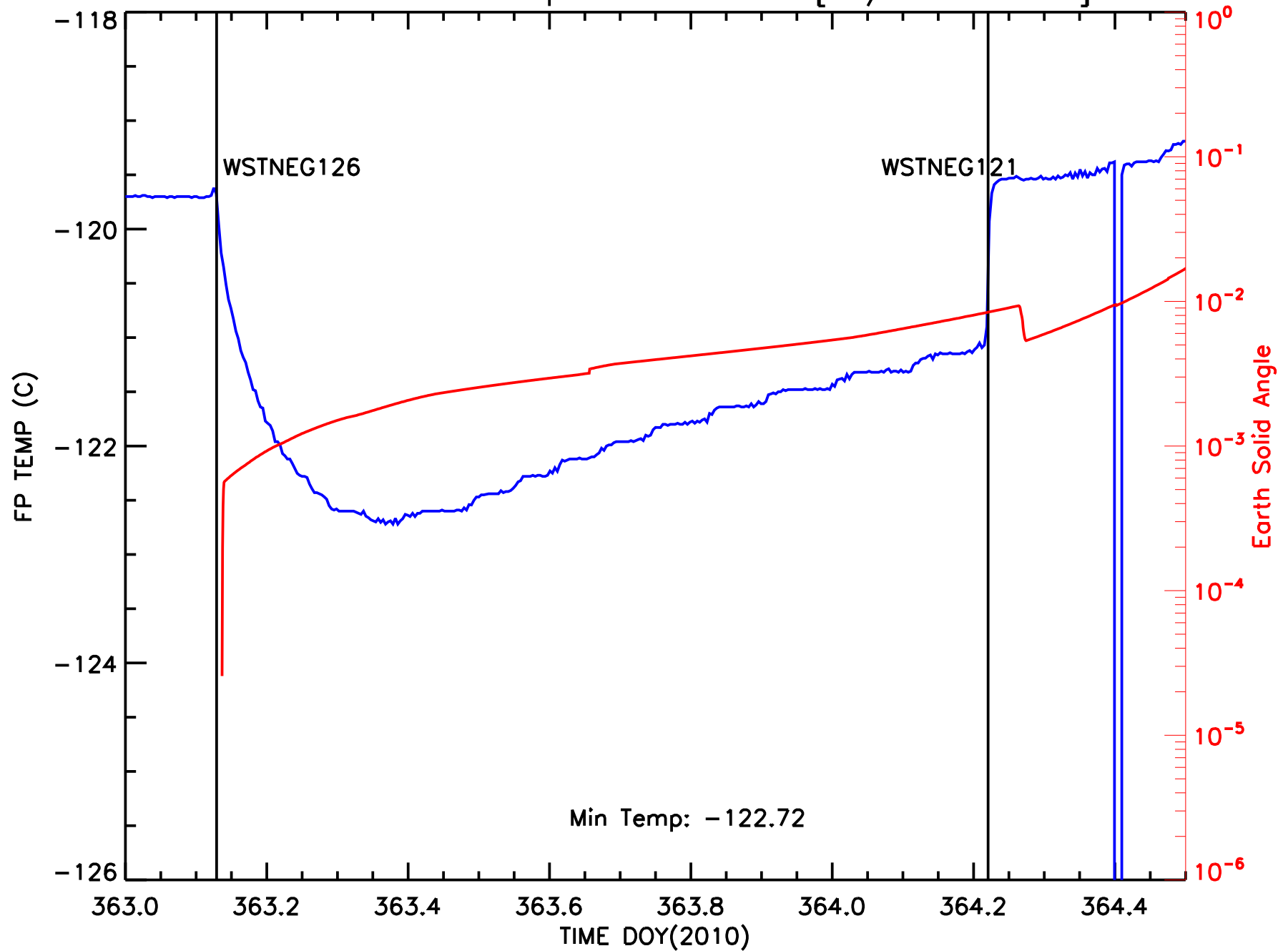
ACIS Focal Plane Temperature vs Time [12/23-24 2010]
