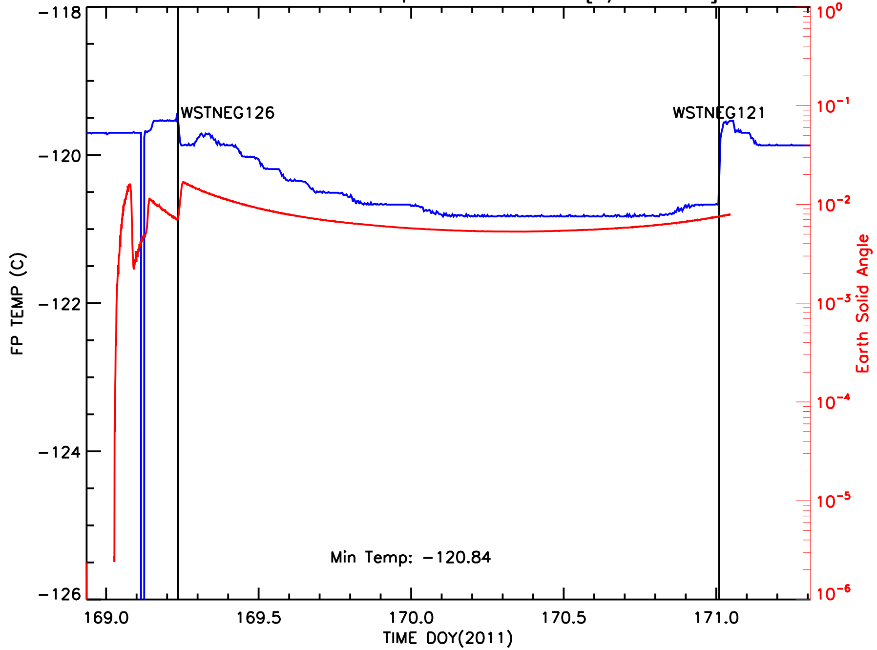
ACIS Focal Plane Temperature vs Time [6/18 2011]
