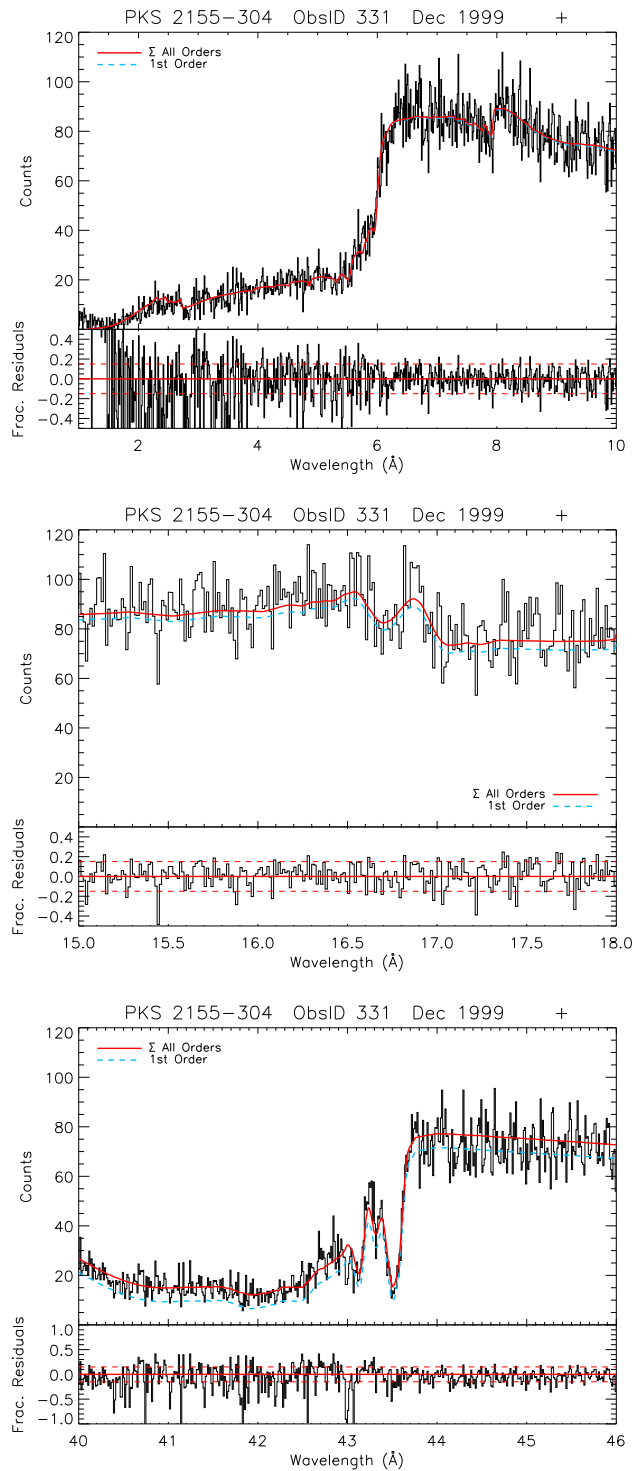
Figure 4. Details of the energy regimes of interest. The top plot shows the repaired higher energy mismatch over \sim 1 - 6 keV ( 2 - 12 Å). The middle plot shows the inclusion of the Cs-M IV,V edges near \sim 0.74 keV ( 16.8 Å). The bottom plot shows the improved alignment of the C-K edge \sim 0.28 keV ( 44 Å). Note the remaining mismatch at \sim 43 Å. Dashed lines on residuals plots are 15% error lines. Data have been binned by CIAO pixel size ( 0.0125 Å). Only data from positive dispersion are shown. Negative dispersion corrections display similar results.
