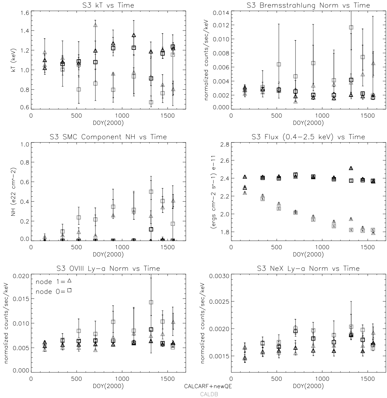
Figure 5. This figure contains 6 panels of E0102 ACIS-S3 fitted spectral parameters plotted versus time. Each panel, however, depicts a different parameter with the default and calcarf/rmf response results plotted in the same panel. The top left panel shows the fitted kT value versus time, while the top right shows the bremsstrahlung normalization versus time. The middle panels show the SMC component absorption versus time on the left and the flux from 0.4 to 2.5 keV versus time on the right. The bottom two panels show the fitted line normalizations versus time of OVIII Ly \alpha (left) and Ne X Ly \alpha (right). Two symbols are used to represent the nodal locations of these observations; node 0 is represented by a square, while node 1 is represented by a triangle. Grayscale is used to show the two types of response products used with black denoting the calcarf/rmf results and light gray denoting the CALDB default results.
