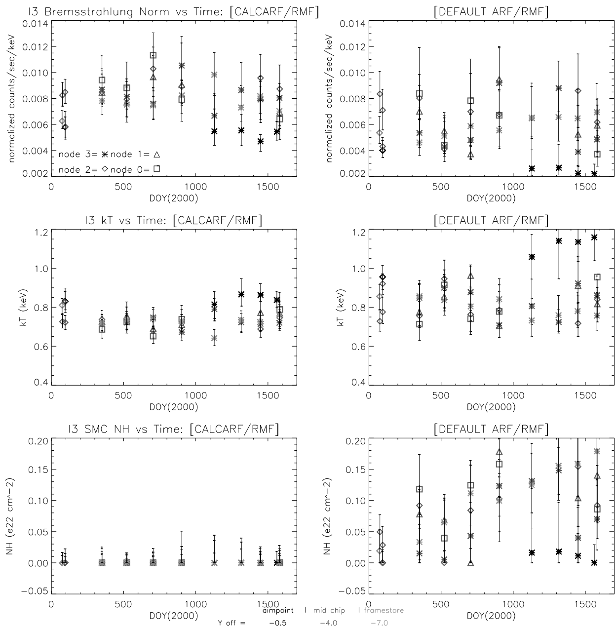
Figure 3. This figure contains 6 panels of E0102 ACIS-I3 fitted spectral parameters plotted versus time. Each set of two panels compares the calcarf/rmf results (left) to the default response results (right). The top two panels depict the bremsstrahlung normalization versus time, while the middle two show the kT value and the bottom two contain the SMC component absorption versus time. Symbols are used here to represent different nodes; node 0 is represented by a square, node 1 by a triangle, node 2 by a diamond and node 3 an asterisk. Grayscale is used to denote approximate chip location with black denoting near aim point observations, medium gray denoting mid-chip observations and light gray denoting observations near the framestore.
