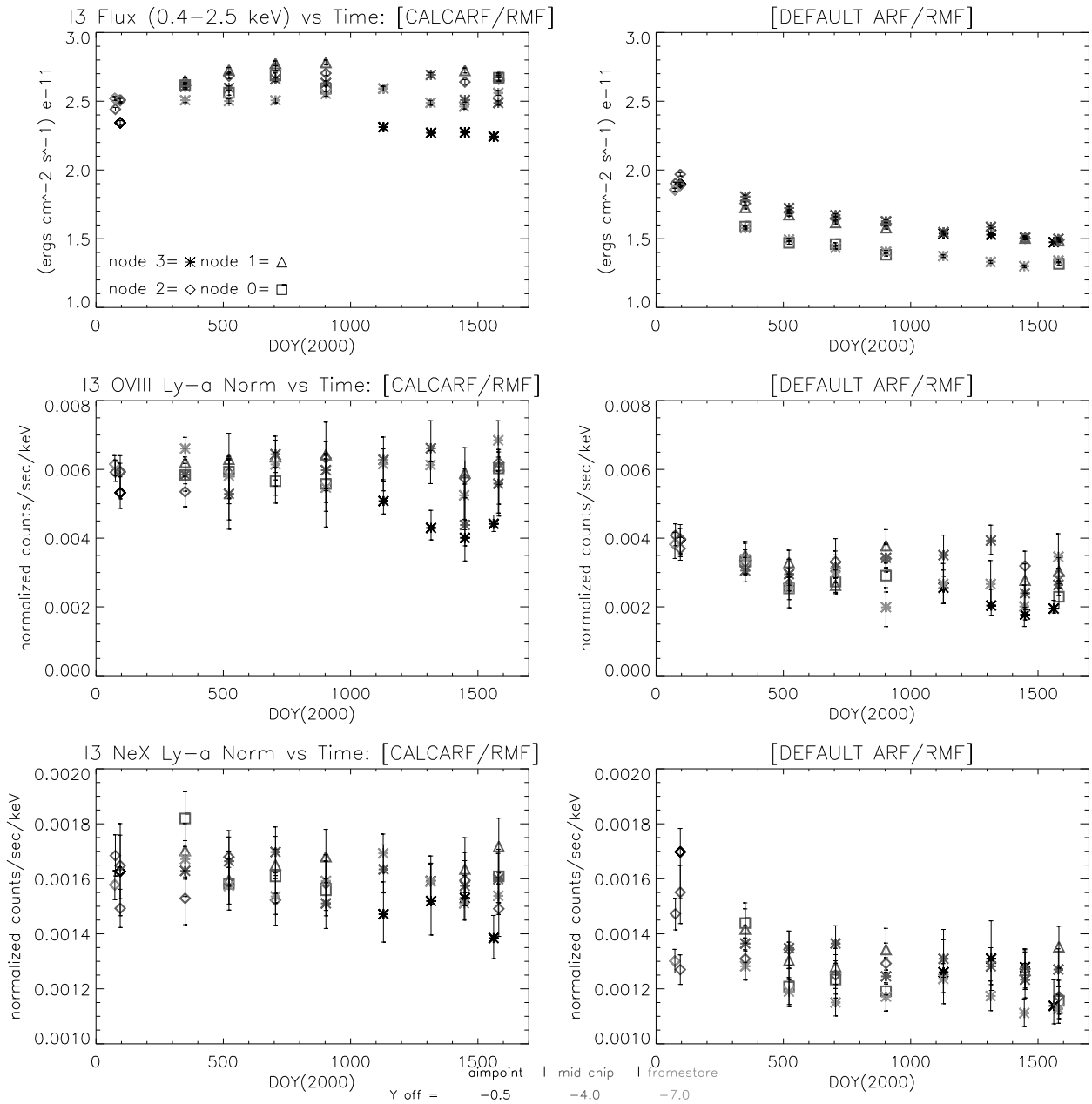
Figure 4. This figure contains 6 panels of E0102 ACIS-I3 fitted spectral parameters plotted versus time. Each set of two panels compares the calcarf/rmf results (left) to the default response results (right). The top two panels depict the the model flux from 0.4 to 2.5 keV versus time, while the middle two show the OVIII Ly \alpha normalization versus time and the bottom two contain the Ne X Ly \alpha normalization versus time. Symbols are used here to represent different nodes; node 0 is represented by a square, node 1 by a triangle, node 2 by a diamond and node 3 an asterisk. Grayscale is used to denote approximate chip location with black denoting near aim point observations, medium gray denoting mid-chip observations and light gray denoting observations near the framestore.
