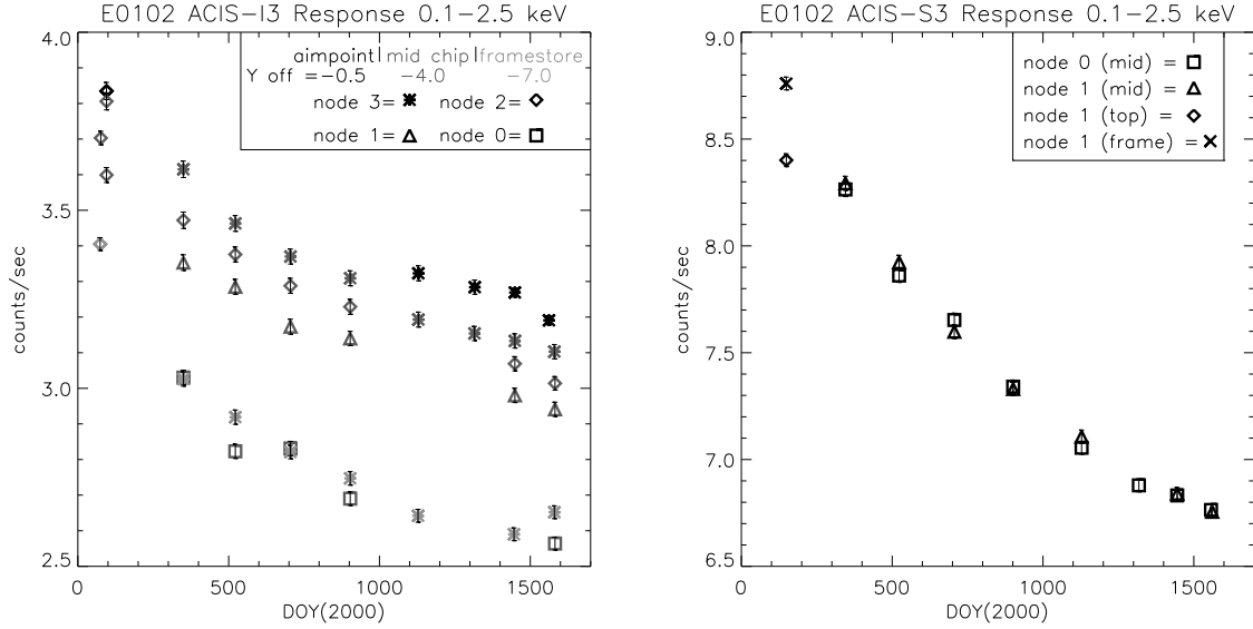
Figure 1. The left panel shows the E0102 count rate (0.1 - 2.5 keV) at each observation on I3; the same plot is shown on the right panel for S3 E0102 observations.
