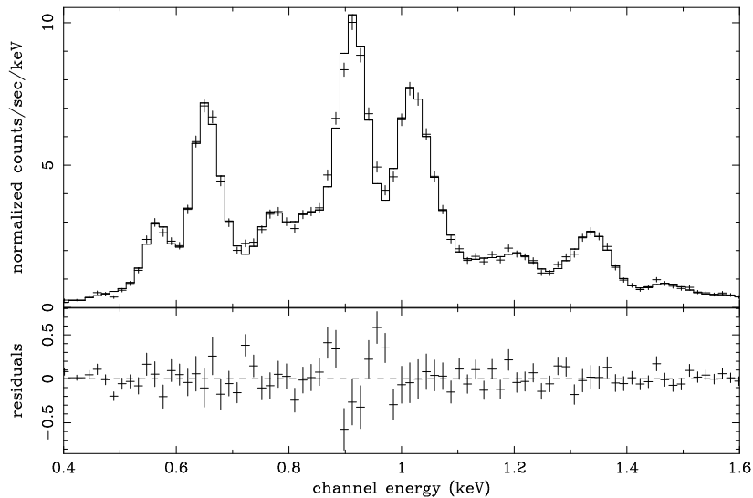
Figure 2. Sample linear plot of a spectral fit of obsid 420 taken 14-03-2000 at -7' off-axis. The data plotted here have had CTI-correction and time-dependent gain applied and were fit using reponse products generated by calcarf and calcrmf2.
