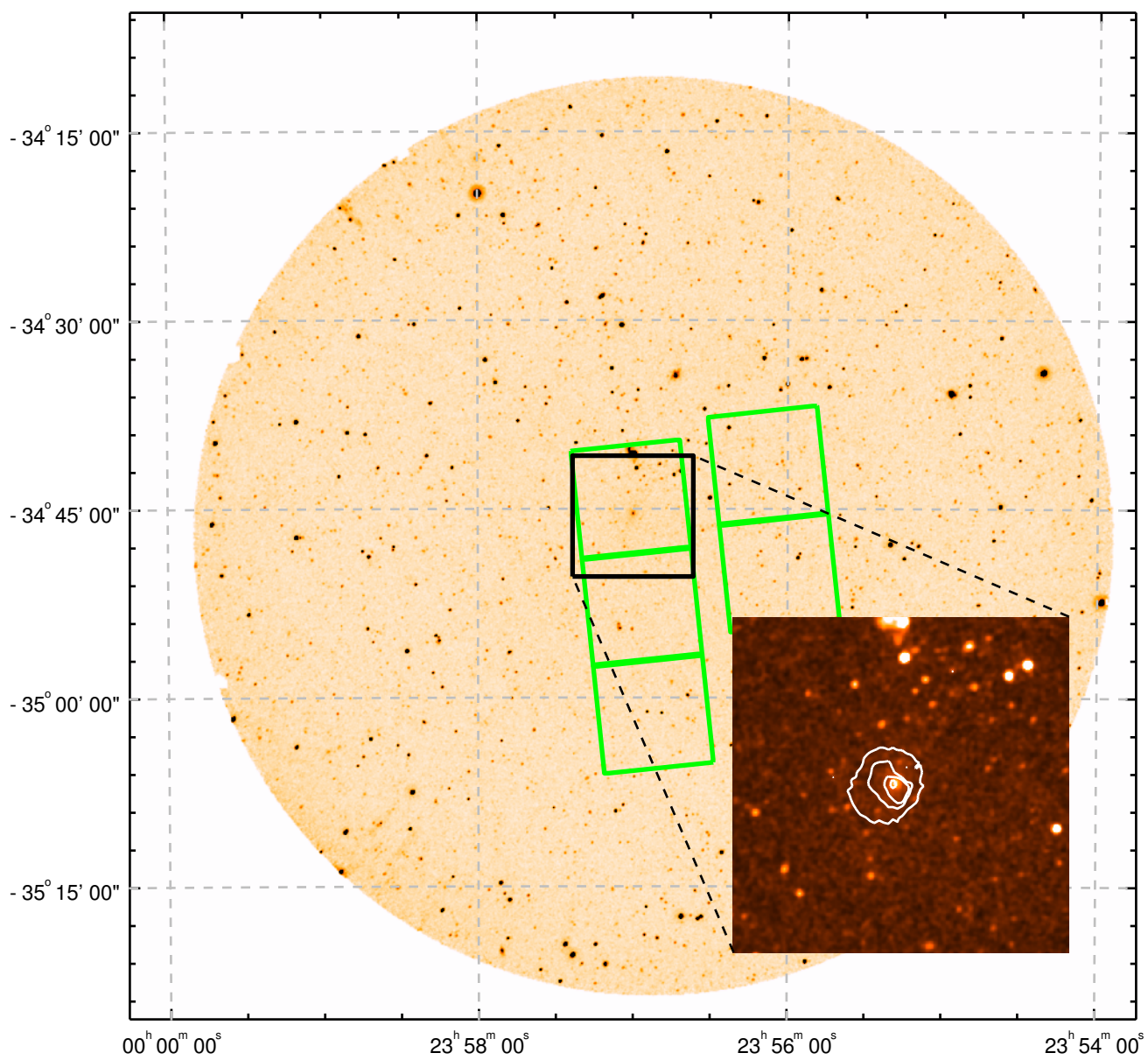
Chandra contours on GALEX image
