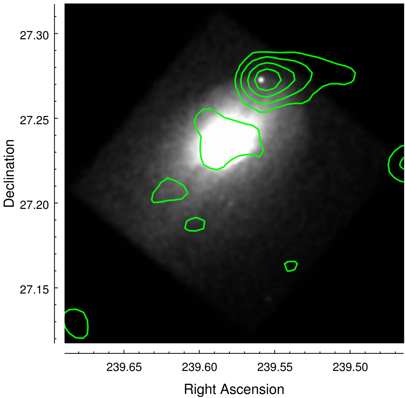
Abell 2142 (NVSS contours on Chandra image)
