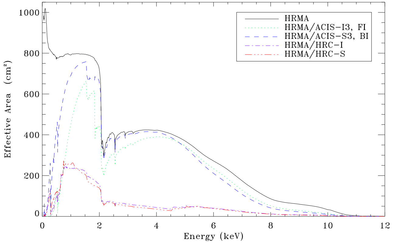
HRMA, HRMA/ACIS & HRMA/HRC On-axis Effective Area
