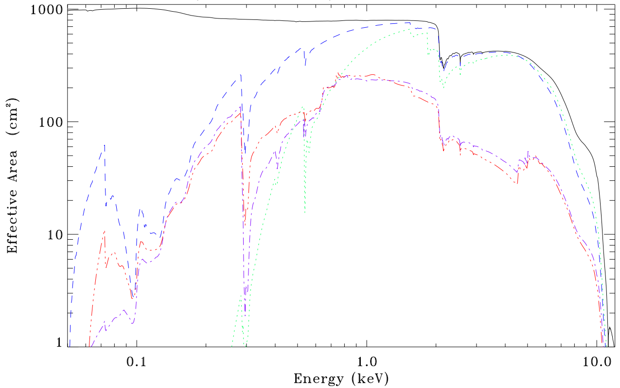
HRMA, HRMA/ACIS & HRMA/HRC On-axis Effective Area
