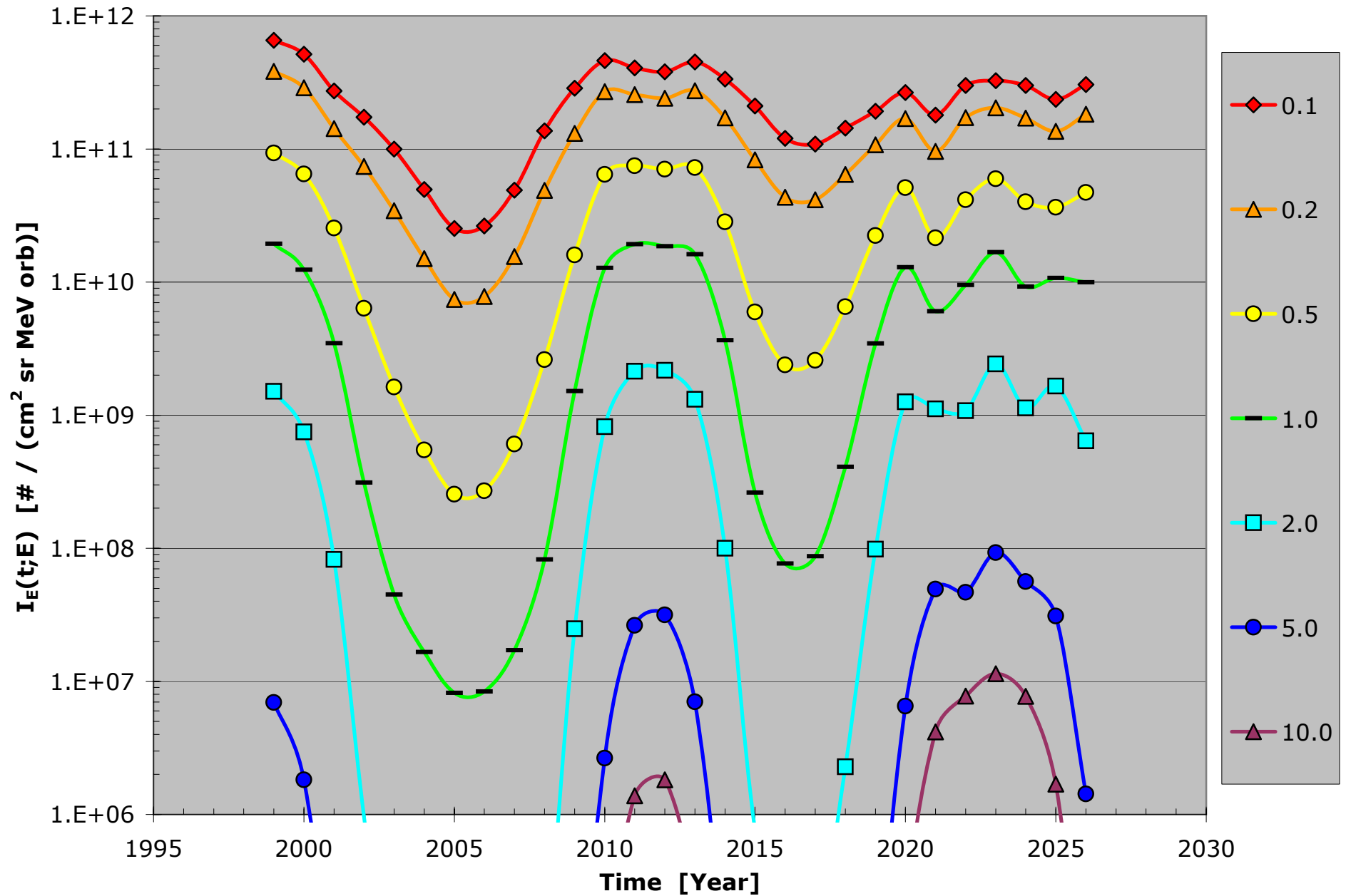
Trapped-proton spectral intensity
