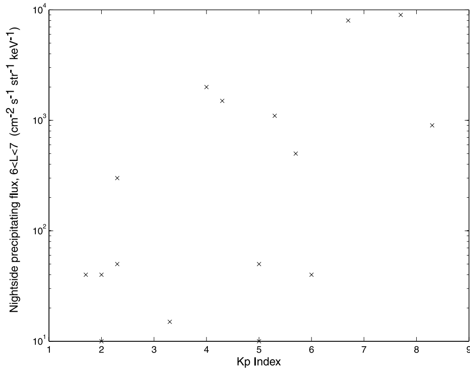
Figure 8. Scatter plot of average nightside precipitation between L = 6 and 7 as a function of K_p for the 3 hour interval inclosing the satellite passage. K_p is a proxy for particle injection into the ring current and the increase in precipitation with K_p indicates that the precipitation accompanies injection.
