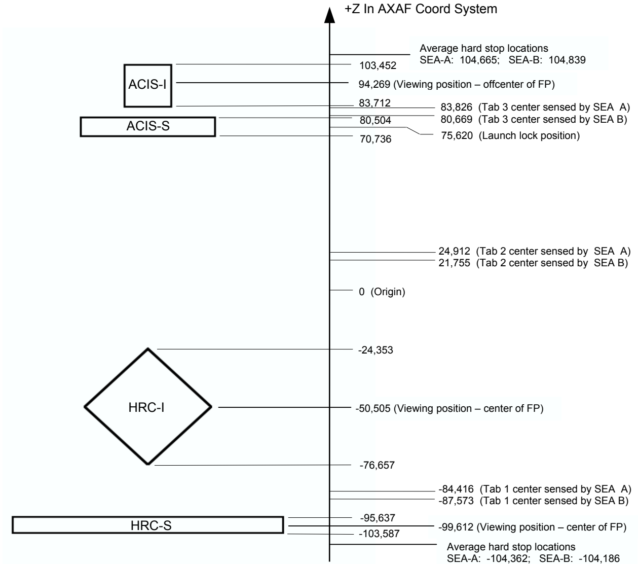
FIGURE 7: Nominal Translating Science Compartment (TSC) Positions (not to scale)
