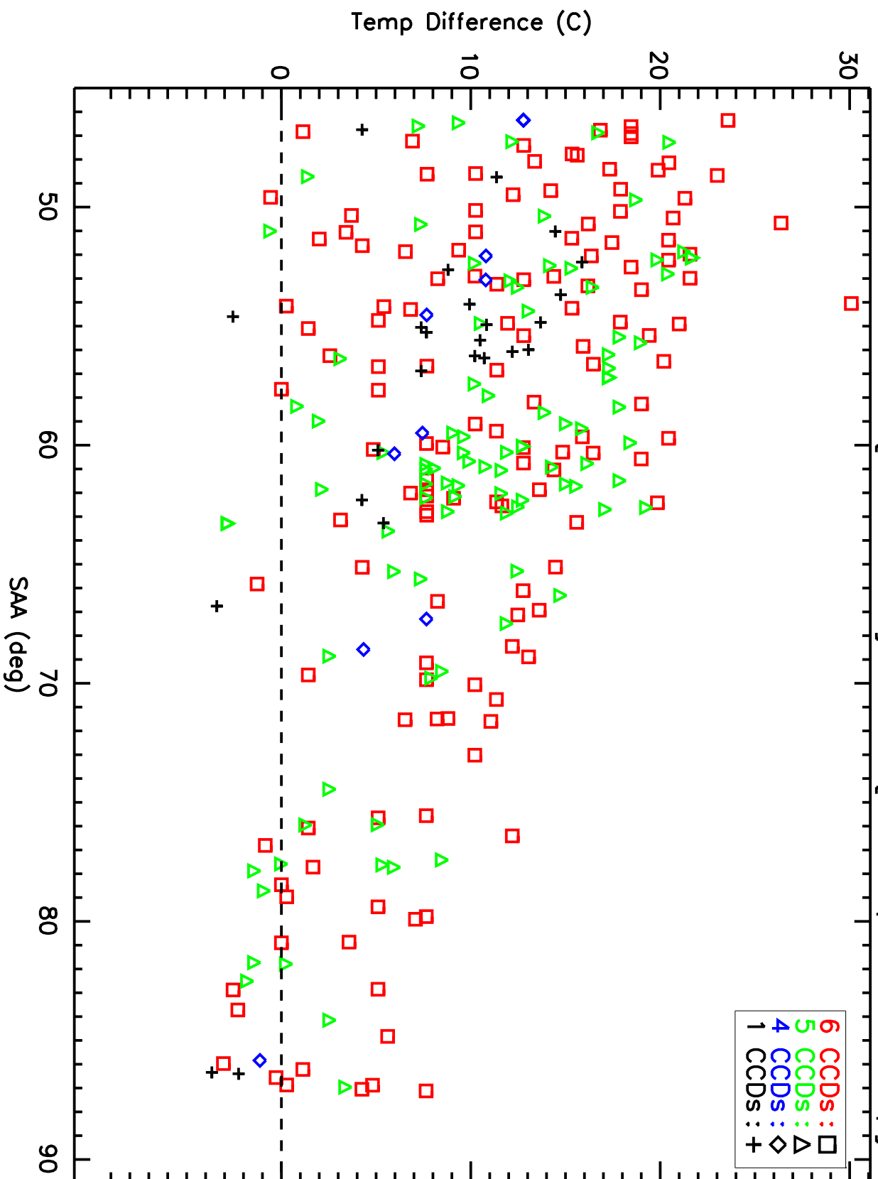
ACIS PSMC THERMAL [2004–2006]: SAA vs [EndTemp – StartTemp]
