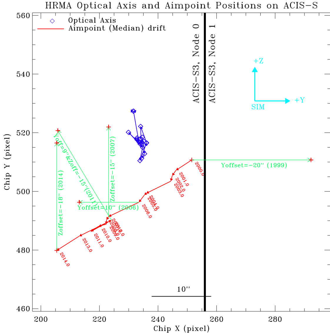
Figure 13: Chandra optical axis (blue) and median aimpoint (red, see Fig. 5) positions on ACIS-S. Each aimpoint position is labeled by the year. The cyan colored arrows show the SIM coordinates. The green arrows show the default offsets implemented over the years (see Section 6 for more details). Due to its accelerated drift in the past two years, now the aimpoint has moved far enough from the node boundary. This memo recommends to apply a fifth default offset of Y-offset = 0'' and Z-offset = -18'' for the Chandra Cycle 16, as shown in this Figure.
