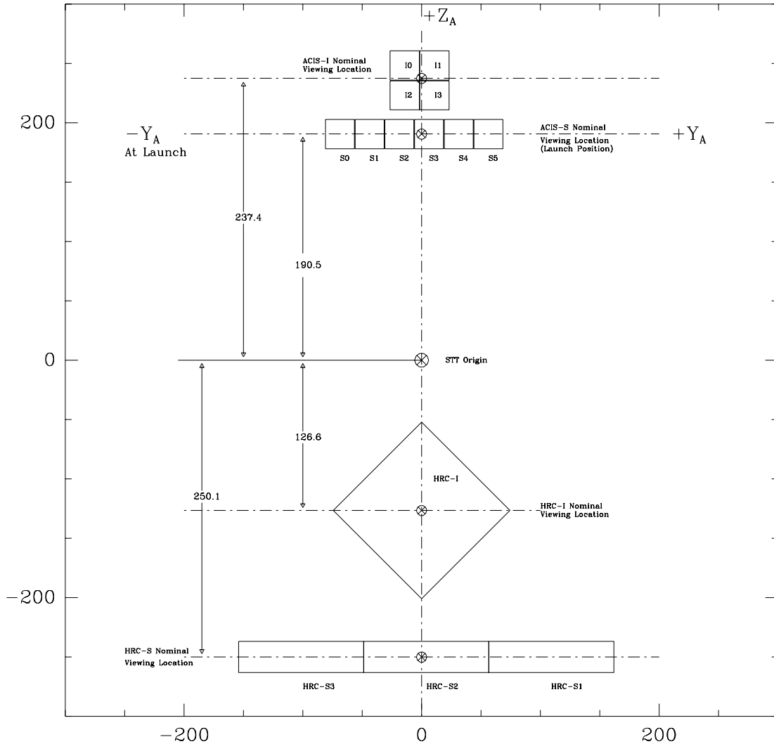
Figure 2: Chandra Detectors Layout: The SIM Translation Table shows the flight focal plane instrument to scale (in mm, coordinate system is AXAF-STT-1.0). SIM +Y is along the x-axis; SIM +Z is along the y-axis. \otimes on each detector marks the aimpoint position with nominal SIM-Z position and zero pointing offset.
