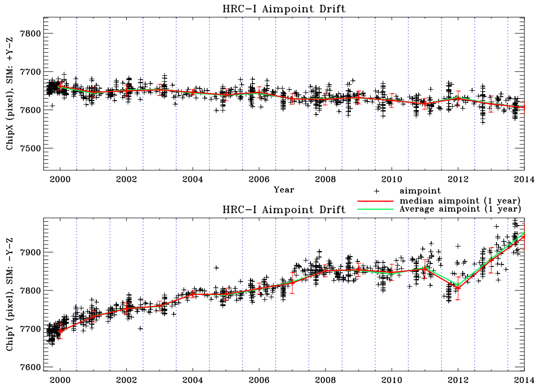
Figure 3: Aimpoint position as a function of time on HRC-I. Solid red (green) lines show the median (average) aimpoint drift in one year bins, separated by vertical dotted blue lines.
