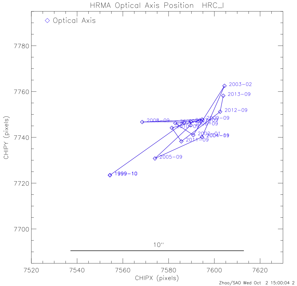
Figure 9: Chandra optical axis positions on HRC-I since launch. Each position is labeled by the year-month. The position is relatively stable and well within a 10'' region.
