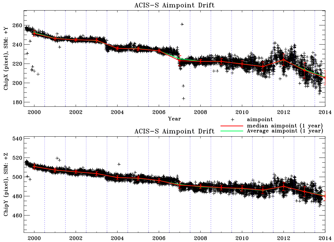
Figure 6: Aimpoint position as a function of time on ACIS-S. Solid red (green) lines show the median (average) aimpoint drift in one year bins, separated by vertical dotted blue lines.
