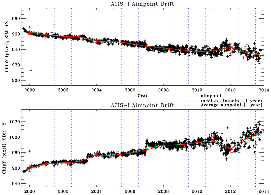
Figure 5: Aimpoint position as a function of time on ACIS-I. Solid red (green) lines show the median (average) aimpoint drift in one year bins, separated by vertical dotted blue lines.
