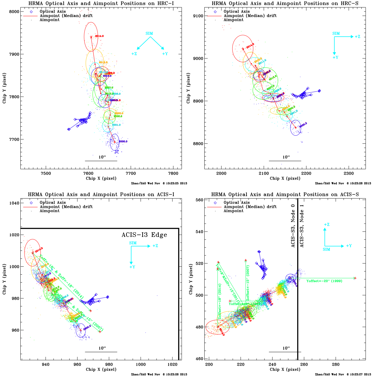
Figure 15: Same as Figures 14 – 13. The dots near the ovals of the same color are the aimpoints of individual observations for that given year.
