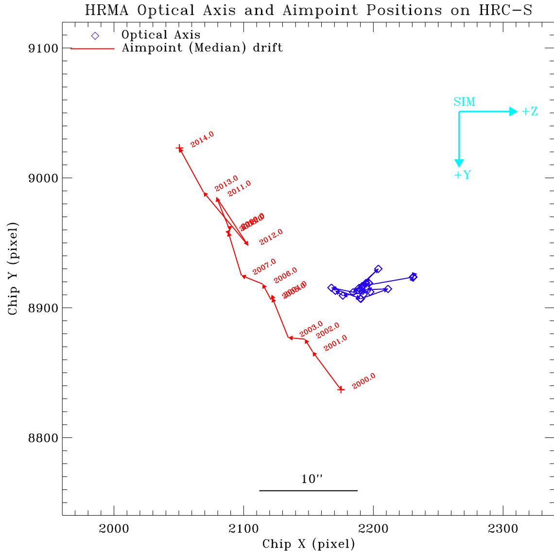
Figure 11: Chandra optical axis (blue) and median aimpoint (red, see Fig. 4) positions on HRC-S. Each aimpoint position is labeled by the year. The cyan colored arrows show the SIM coordinates.
