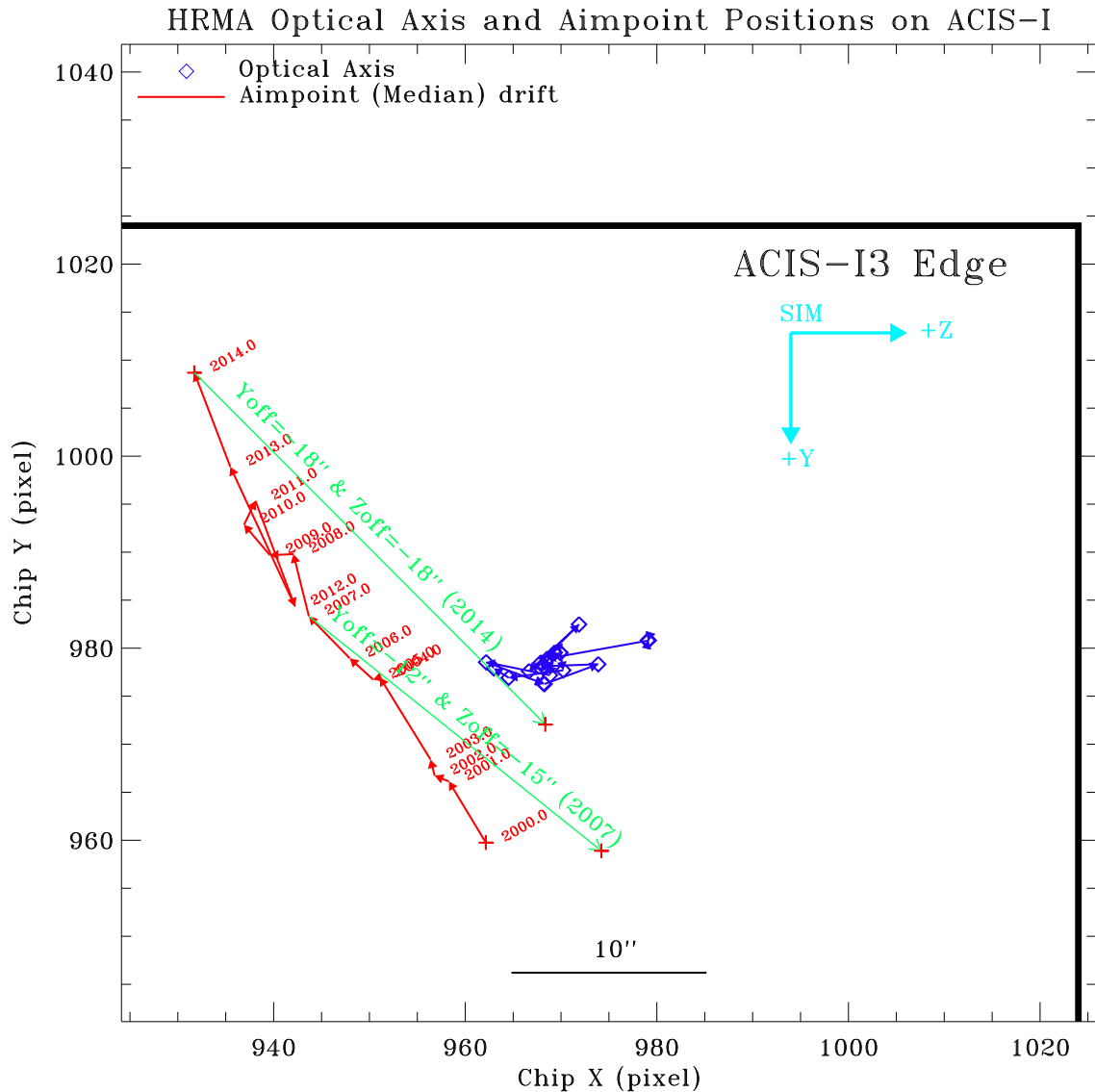
Figure 12: Chandra optical axis (blue) and median aimpoint (red, see Fig. 5) positions on ACIS-I. Each aimpoint position is labeled by the year. The cyan colored arrows show the SIM coordinates. ACIS-I observations were conducted without default offset since the Chandra launch until the end of 2006. In December 2006, the aimpoint had a sudden shift of \sim 10'' due to the ACA primary focal plan CCD cool down from -15^{\circ}\text{C} to -20^{\circ}\text{C} . This sudden shift brought the aimpoint uncomfortably close to the ACIS-I3 chip edge. As it continue to drift towards the edge, the dither pattern ( 16'' peak-to-peak) will soon fall out of the chip. Therefore a default Y-offset = -15'' and Z-offset = -12'' was implemented to move the aimpoint away from the chip edge and also closer to the optical axis. The green arrow shows the magnitude and the direction of this default offset. Since then, all the ACIS-I observations have been conducted with this default offset, unless the observers requested otherwise. Due to its accelerated drift in the past two years, the aimpoint is now once again very close to the ACIS-I3 edge. This memo recommends to apply a new default offset of Y-offset = -18'' and Z-offset = -18'' for the Chandra Cycle 16, as shown in this Figure.
