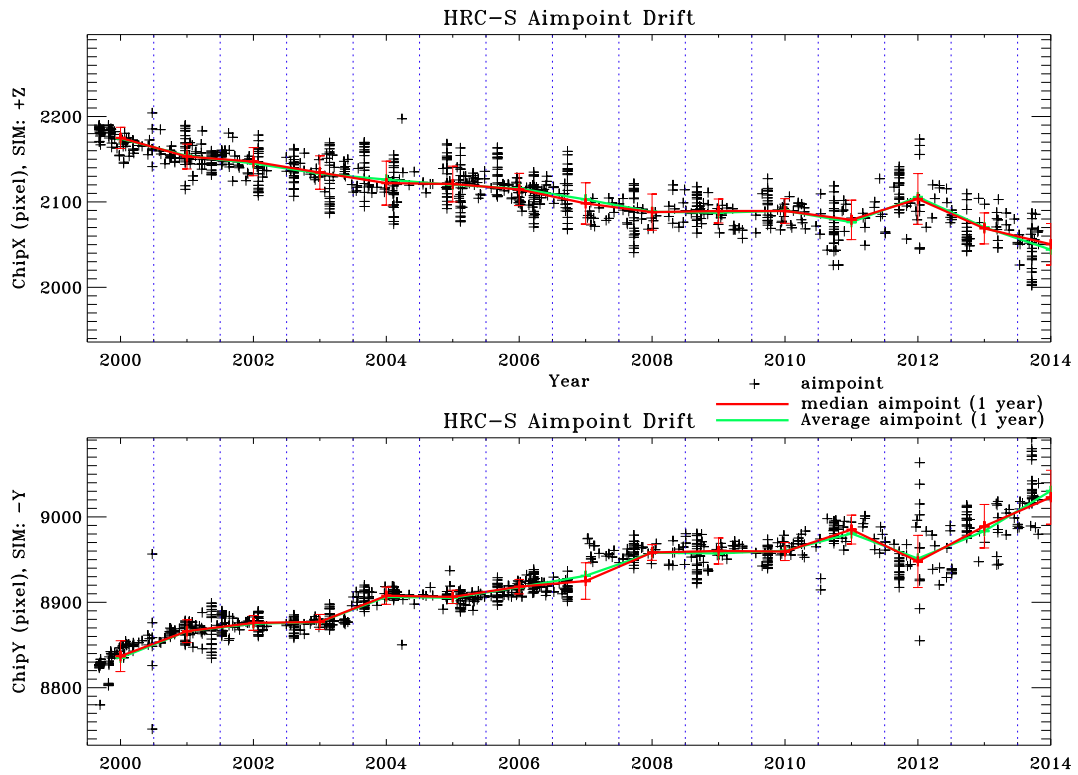
Figure 4: Aimpoint position as a function of time on HRC-S. Solid red (green) lines show the median (average) aimpoint drift in one year bins, separated by vertical dotted blue lines.
