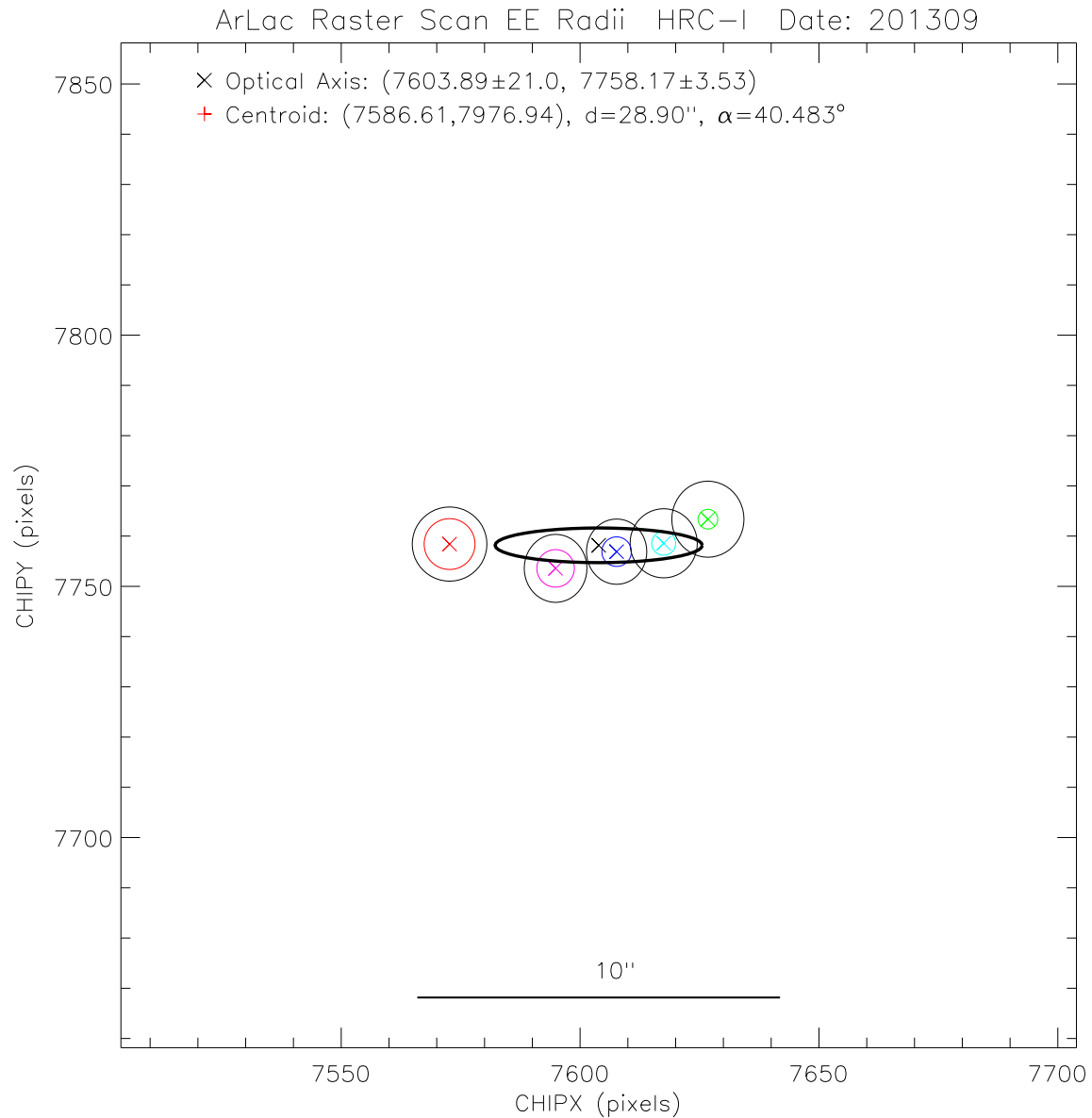
Figure 8: Same as Fig. 7 but zoomed in to the optical axis region. The five colored \times 's are the positions of quadratic function minimum for 50% – 90% encircled energy fit. The colored circles indicate their encircled energy radii. The black circles are the 1\text{-}\sigma fit errors. The black \times marks the optical axis position, taken as the mean of the above 5 minimums. The black oval is the 1\text{-}\sigma error ellipse.
