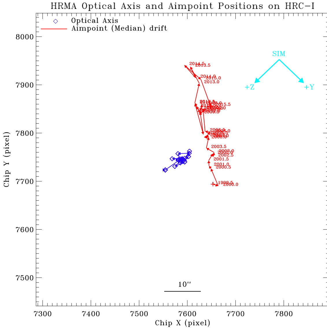
Figure 10: Chandra optical axis (blue) and median aimpoint (red, see Fig. 6) positions in half year bins on HRC-I. Each aimpoint position is labeled by the year. The cyan colored arrows show the SIM coordinates.
