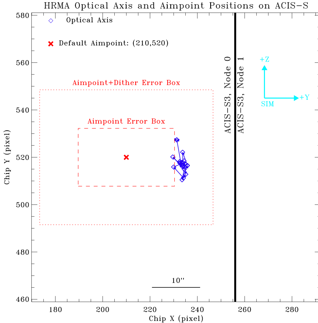
Figure 18: Chandra optical axis (blue diamonds) positions for each year and permanent default aimpoint (red cross) on ACIS-S. The small box (red dashed line, 20'' \times 12'' , or 40.7 \times 24.4 pixels) centered at the aimpoint is the error box of the aimpoint center, i.e. an on-axis target can be anywhere inside this box. The large box (red dotted line, 36'' \times 28'' , or 73.2 \times 56.9 pixels) is the error box of aimpoint with dither.
