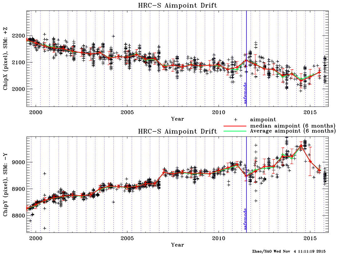
Figure 7: Aimpoint position as a function of time on HRC-S. Solid red (green) lines show the median (average) aimpoint drift in 6 months bins, separated by vertical dotted blue lines.
