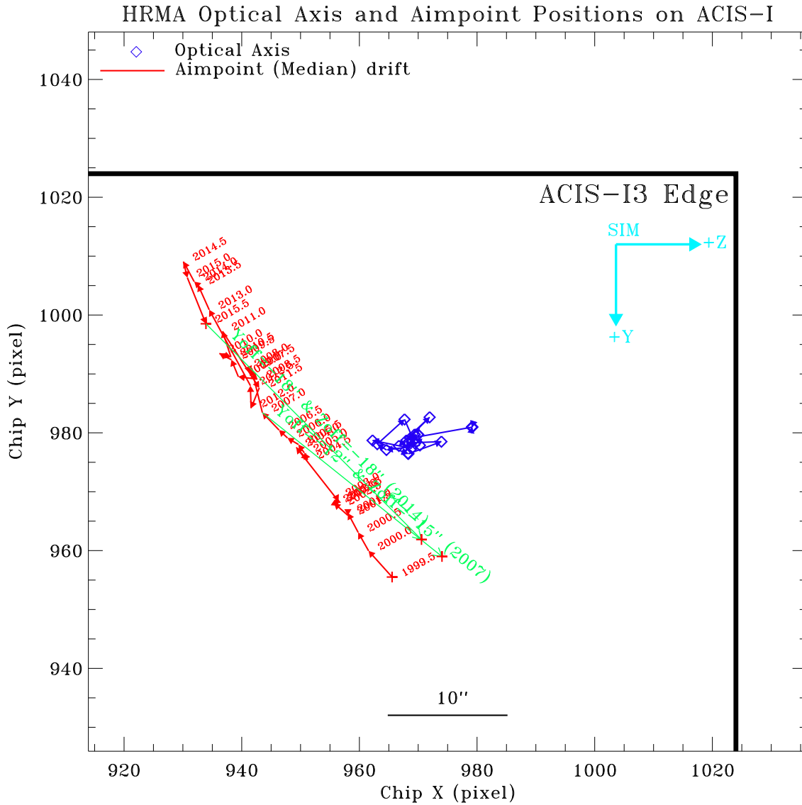
Figure 12: Chandra optical axis (blue) and median aimpoint (red, see Fig. 8) positions in half year bins on ACIS-I. Each aimpoint position is labeled by the year. The cyan colored arrows show the SIM coordinates. ACIS-I observations were conducted without default offset since the Chandra launch until the end of 2006. In December 2006, the aimpoint had a sudden shift of \sim 10'' due to the ACA primary focal plan CCD cool down from -15^{\circ}\text{C} to -20^{\circ}\text{C} . This sudden shift brought the aimpoint uncomfortably close to the ACIS-I3 chip edge. As it continue to drift towards the edge, the dither pattern ( 16'' peak-to-peak) will soon fall out of the chip. Therefore a default Y-offset = -15'' and Z-offset = -12'' was implemented to move the aimpoint away from the chip edge and also closer to the optical axis. Due to its accelerated drift since early 2012, the aimpoint was once again very close to the ACIS-I3 edge in late 2013. So since December 2013, a new default offset of Y-offset = -18'' and Z-offset = -18'' was applied. The two green arrows in the figure show the magnitude and the direction of the default offsets. All the ACIS-I observations were conducted with these default offsets starting in the year labels next to the green arrows, unless the observers requested otherwise.
