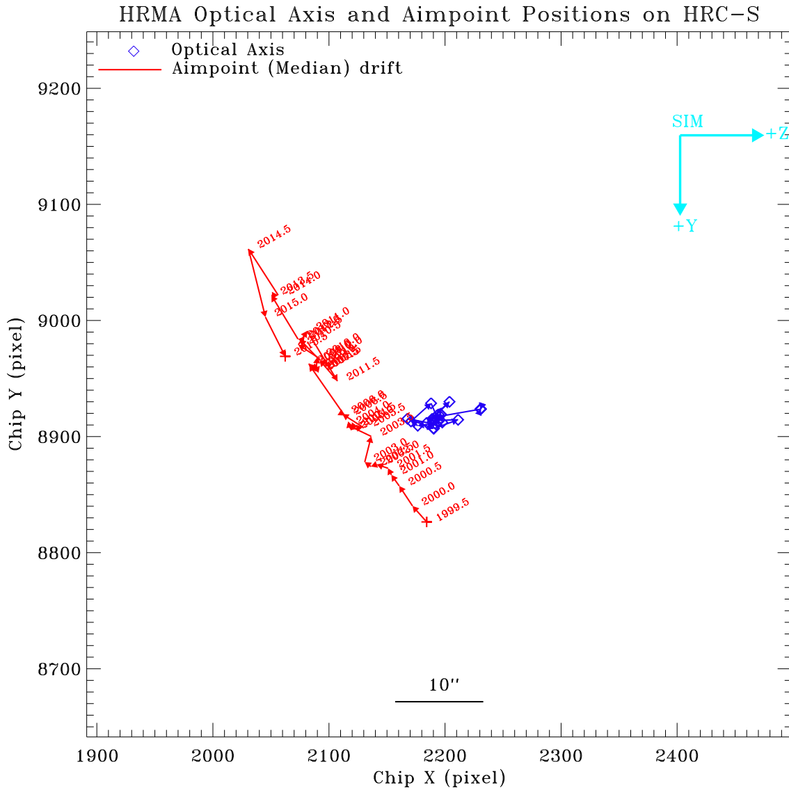
Figure 11: Chandra optical axis (blue) and median aimpoint (red, see Fig. 7) positions in half year bins on HRC-S. Each aimpoint position is labeled by the year. The cyan colored arrows show the SIM coordinates.
