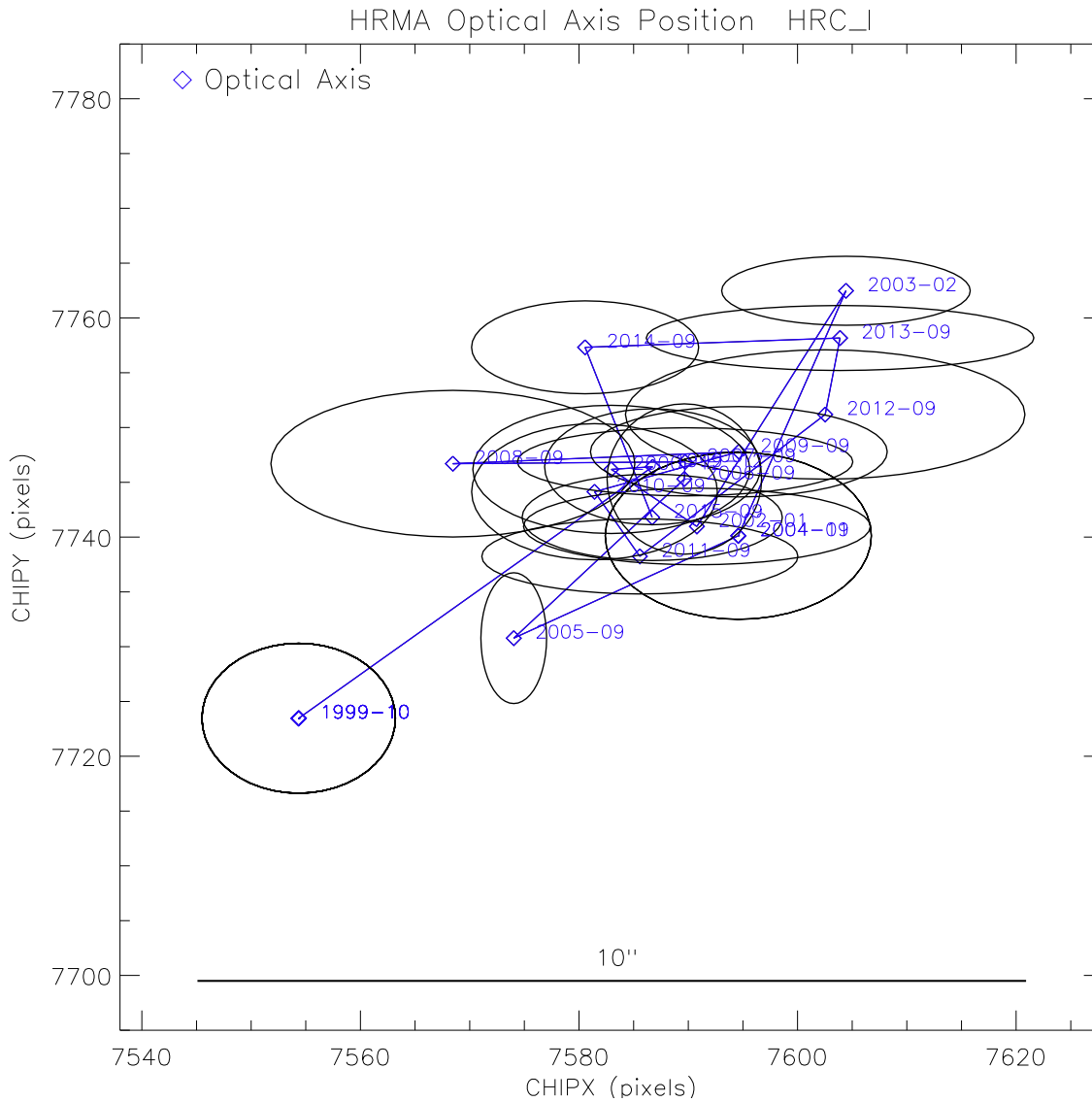
Figure 5: Chandra optical axis positions on HRC-I since launch. Each position is labeled by the year-month. The ellipse around each position is the 1 - \sigma measurement error ellipse for that given year. The drift of optical axis position is consistent with the measurement errors. The optical axis position is very stable and well within a 10'' region. Since year 2000, the optical axis drift was well within a 6'' region.
