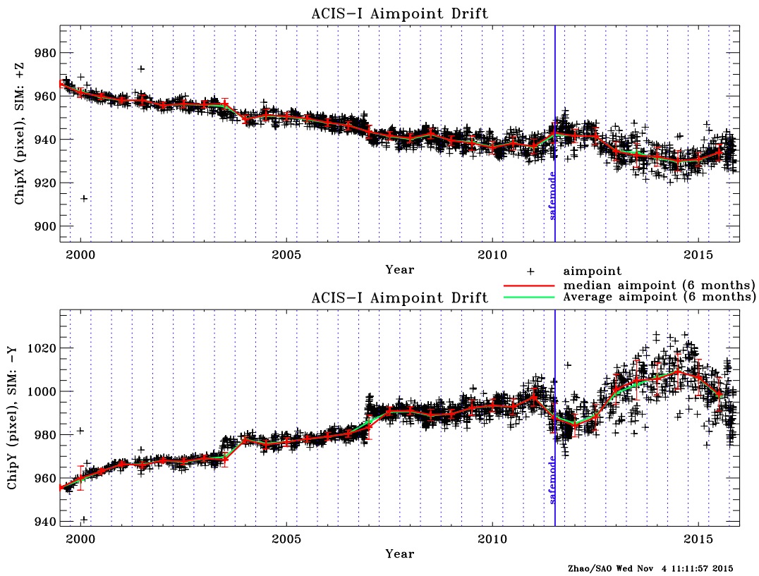
Figure 8: Aimpoint position as a function of time on ACIS-I. Solid red (green) lines show the median (average) aimpoint drift in 6 months bins, separated by vertical dotted blue lines.
