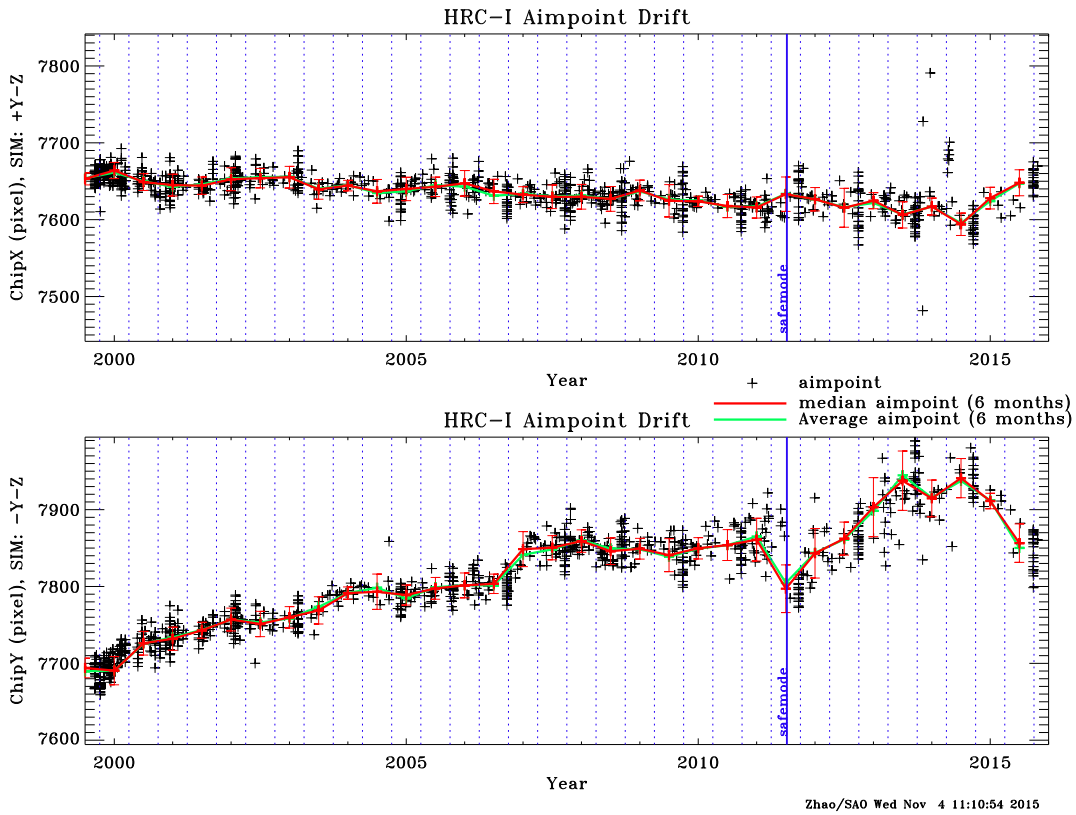
Figure 6: Aimpoint position as a function of time on HRC-I. Solid red (green) lines show the median (average) aimpoint drift in 6 months bins, separated by vertical dotted blue lines.
