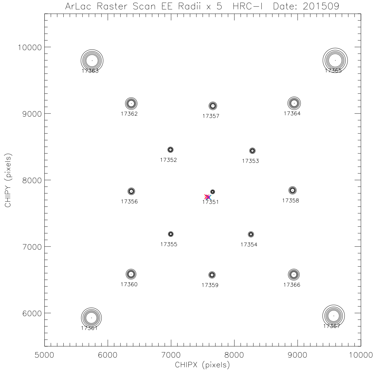
Figure 3: HRC-I raster scan observation of Ar Lac in chip coordinates. Circles around each observation point have the 50% – 90% encircled energy radii \times 5 . The data are fit to a 2-D quadratic function to find the optical axis. Data taken in September 2015. The numbers under the circles are the OBSIDs of the observations.
