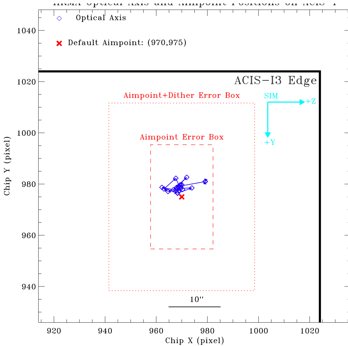
Figure 17: Chandra optical axis (blue diamonds) positions for each year and permanent default aimpoint (red cross) on ACIS-I. The small box (red dashed line, 12'' \times 20'' , or 24.4 \times 40.7 pixels) centered at the aimpoint is the error box of the aimpoint center, i.e. an on-axis target can be anywhere inside this box. The large box (red dotted line, 28'' \times 36'' , or 56.9 \times 73.2 pixels) is the error box of aimpoint with dither.
