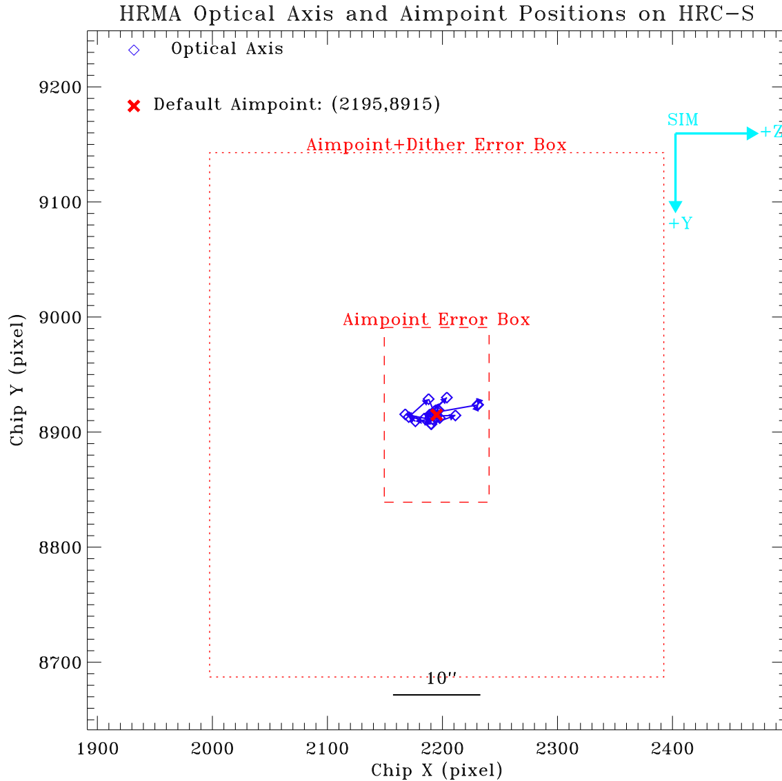
Figure 20: Chandra optical axis (blue diamonds) positions for each year and permanent default aimpoint (red cross) on HRC-S. The small box (red dashed line, 12'' \times 20'' , or 91.1 \times 151.8 pixels) centered at the aimpoint is the error box of the aimpoint center, i.e. an on-axis target can be anywhere inside this box. The large box (red dotted line, 52'' \times 60'' , or 394.7 \times 455.4 pixels) is the error box of aimpoint with dither.
