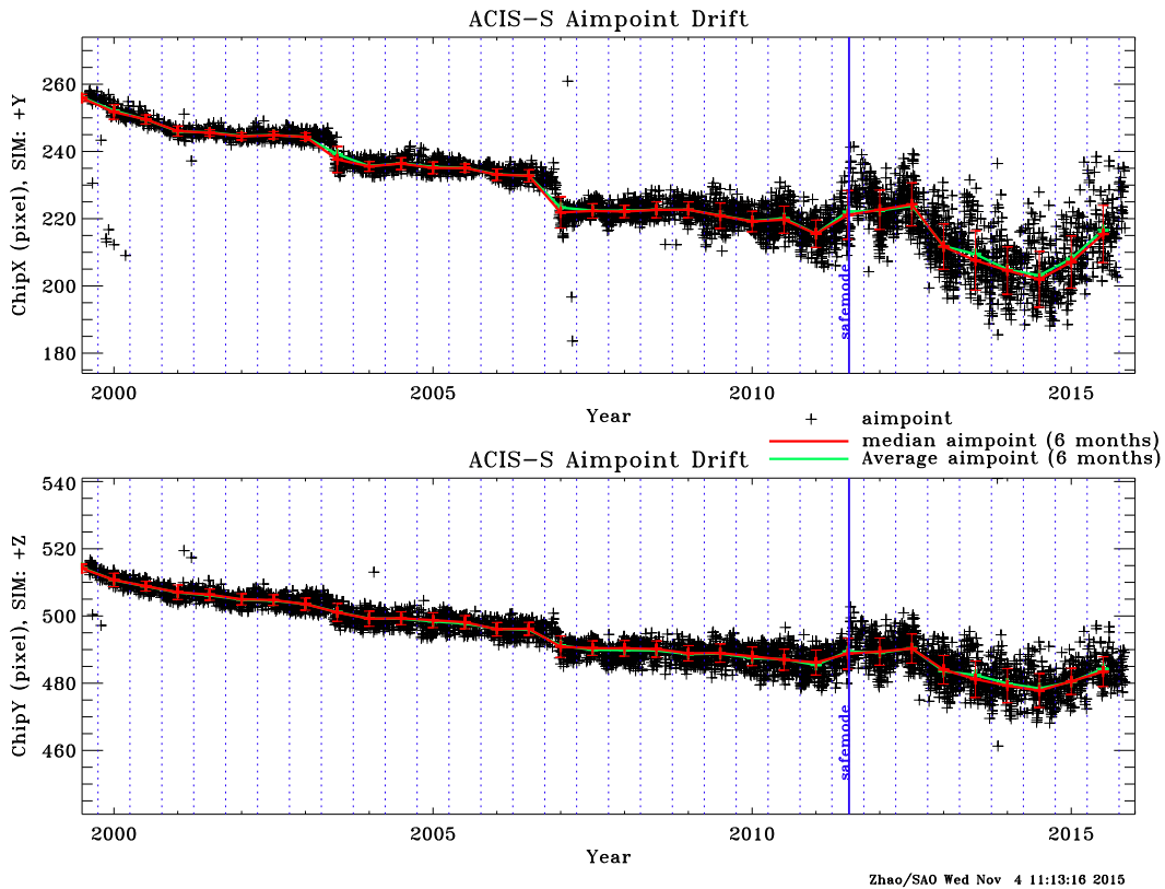
Figure 9: Aimpoint position as a function of time on ACIS-S. Solid red (green) lines show the median (average) aimpoint drift in 6 months bins, separated by vertical dotted blue lines.
