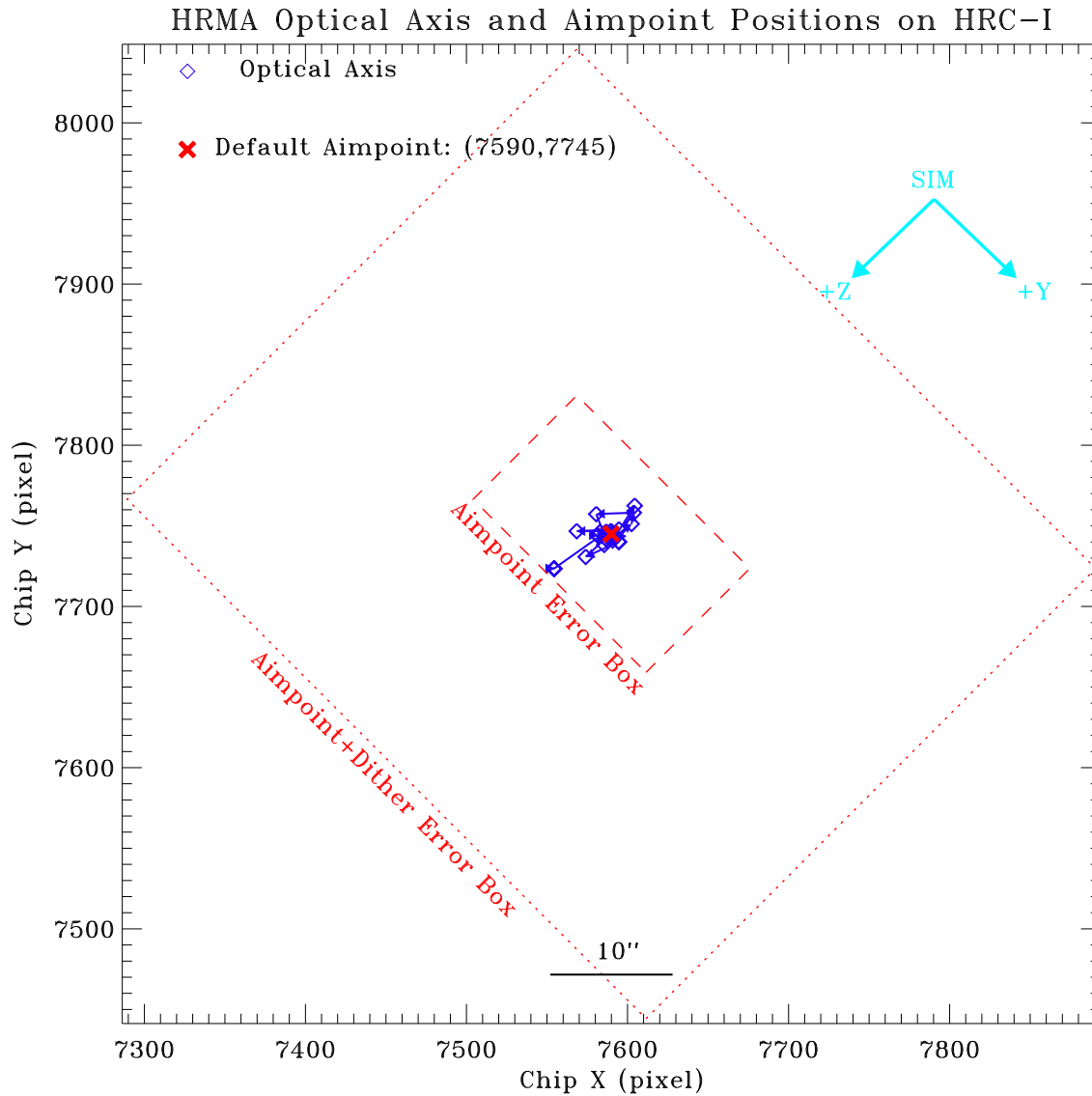
Figure 19: Chandra optical axis (blue diamonds) positions for each year and permanent default aimpoint (red cross) on HRC-I. The small box (red dashed line, 20'' \times 12'' , or 151.8 \times 91.1 pixels in SIM [Y, Z]) centered at the aimpoint is the error box of the aimpoint center, i.e. an on-axis target can be anywhere inside this box. The large box (red dotted line, 60'' \times 52'' , or 455.4 \times 394.7 pixels in SIM [Y, Z]) is the error box of aimpoint with dither.
