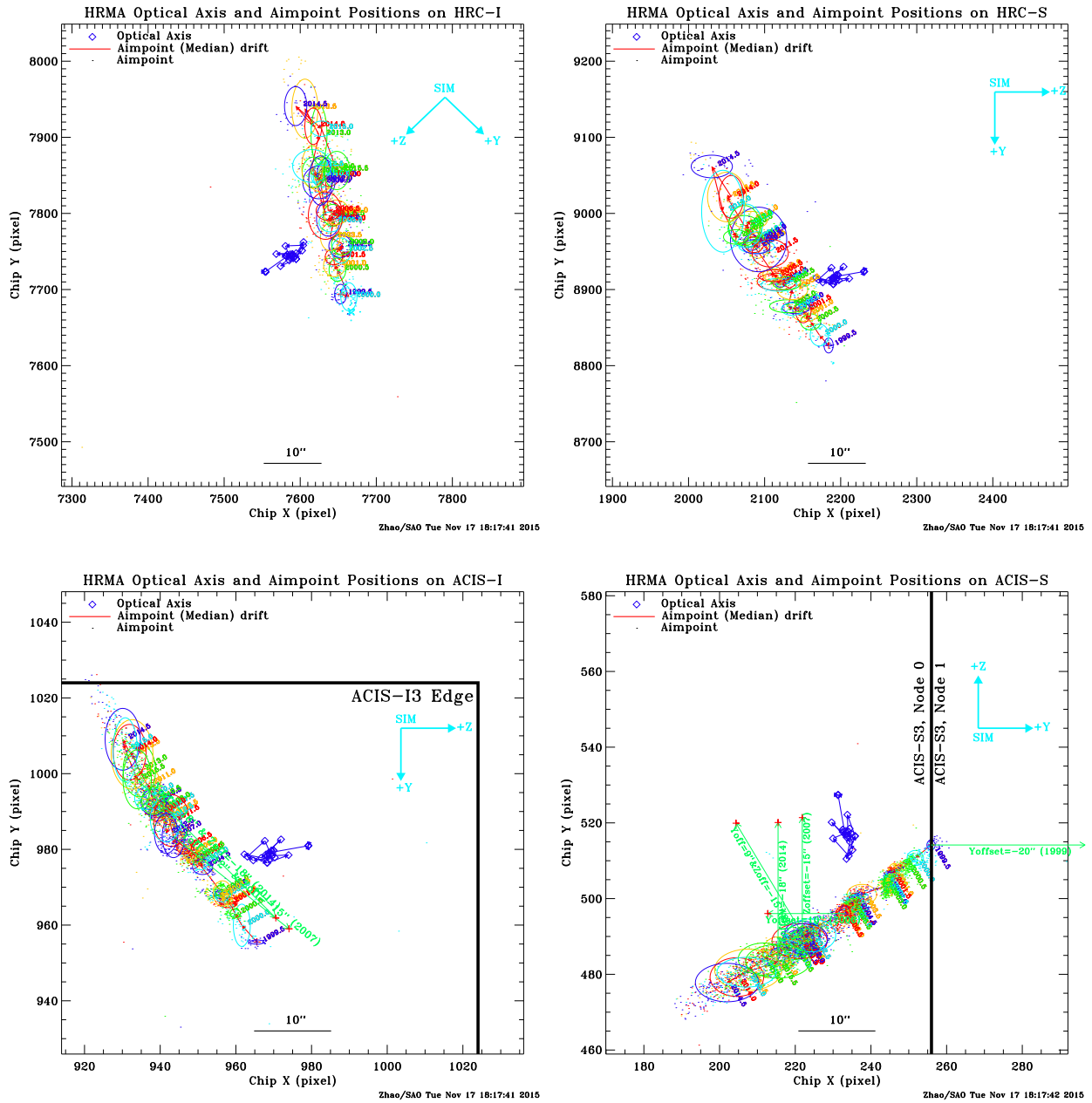
Figure 15: Same as Figures 14, the dots near the ovals of the same color are the aimpoints of individual observations for that given half year.
