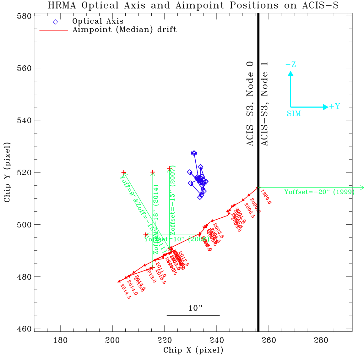
Figure 13: Chandra optical axis (blue) and median aimpoint (red, see Fig. 8) positions in half year bins on ACIS-S. Each aimpoint position is labeled by the year. The cyan colored arrows show the SIM coordinates. The green arrows show the default offsets implemented over the years (see Section 6 for more details). The current default offset is Y-offset = 0'' and Z-offset = -18'', implemented in December 2013. All the ACIS-S observations were conducted with these default offsets starting in the year labels next to the green arrows, unless the observers requested otherwise.
