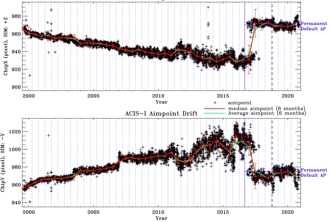
Figure 14: Aimpoint position as a function of time on ACIS-I since launch. Solid red (green) lines show the median (average) aimpoint drift in 6 month bins, separated by vertical dotted blue lines. The vertical solid blue line indicates the start of the dynamical aimpoint adjustment.
