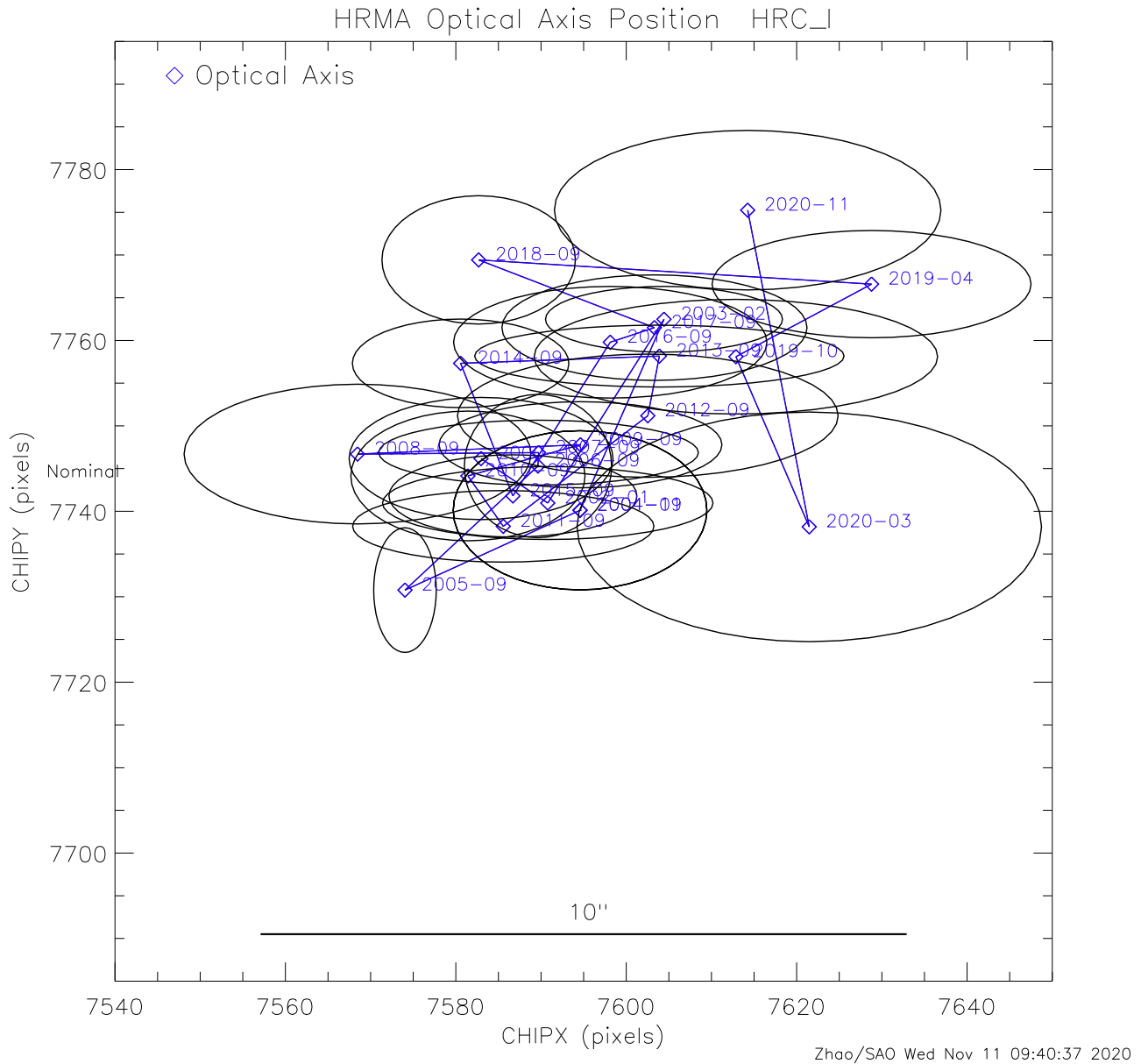
Figure 8: Chandra optical axis positions on HRC-I since launch. Each position is labeled by the year-month. The ellipse around each position is the 1\text{-}\sigma measurement error ellipse for that given year. The drift of optical axis position is consistent with the measurement errors. The optical axis position is very stable and well within a 10'' region.
