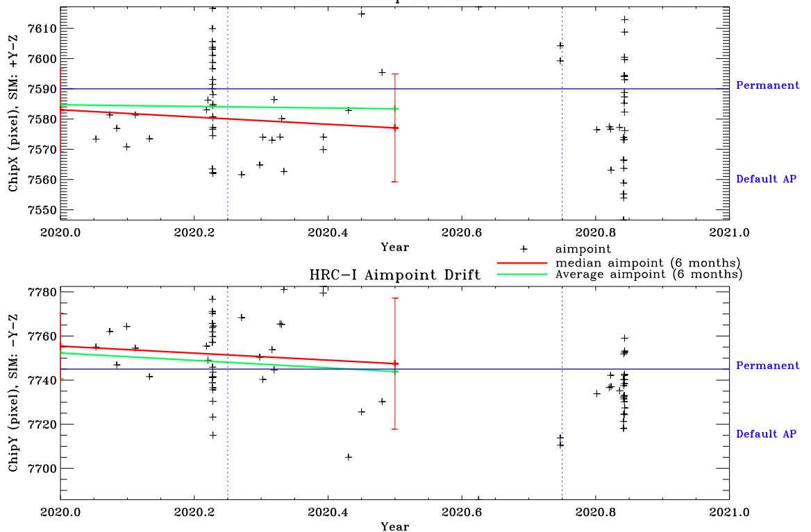
Figure 11: Aimpoint position as a function of time on HRC-I in the past year.
