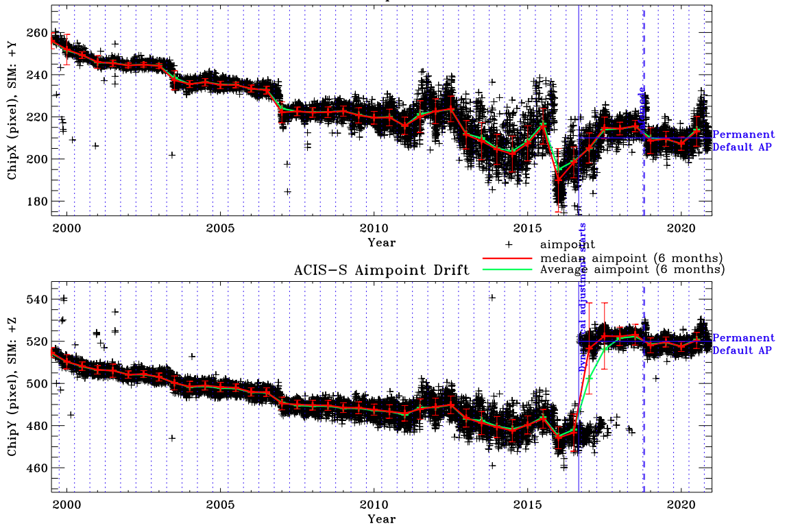
Figure 16: Aimpoint position as a function of time on ACIS-S since launch. Solid red (green) lines show the median (average) aimpoint drift in 6 month bins, separated by vertical dotted blue lines. The vertical solid blue line indicates the start of the dynamical aimpoint adjustment.
