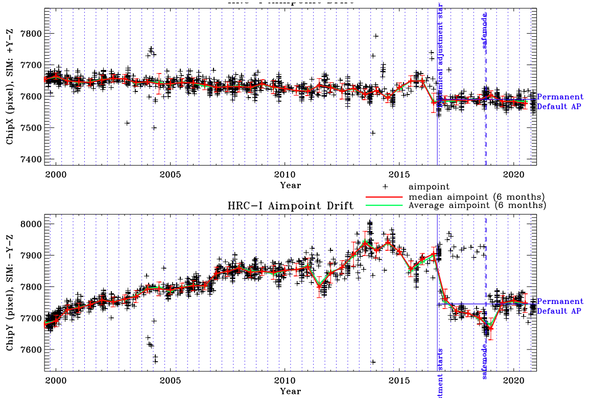
Figure 10: Aimpoint position as a function of time on HRC-I since launch. Solid red (green) lines show the median (average) aimpoint drift in 6 month bins, separated by vertical dotted blue lines. The vertical solid blue line indicates the start of the dynamical aimpoint adjustment.
