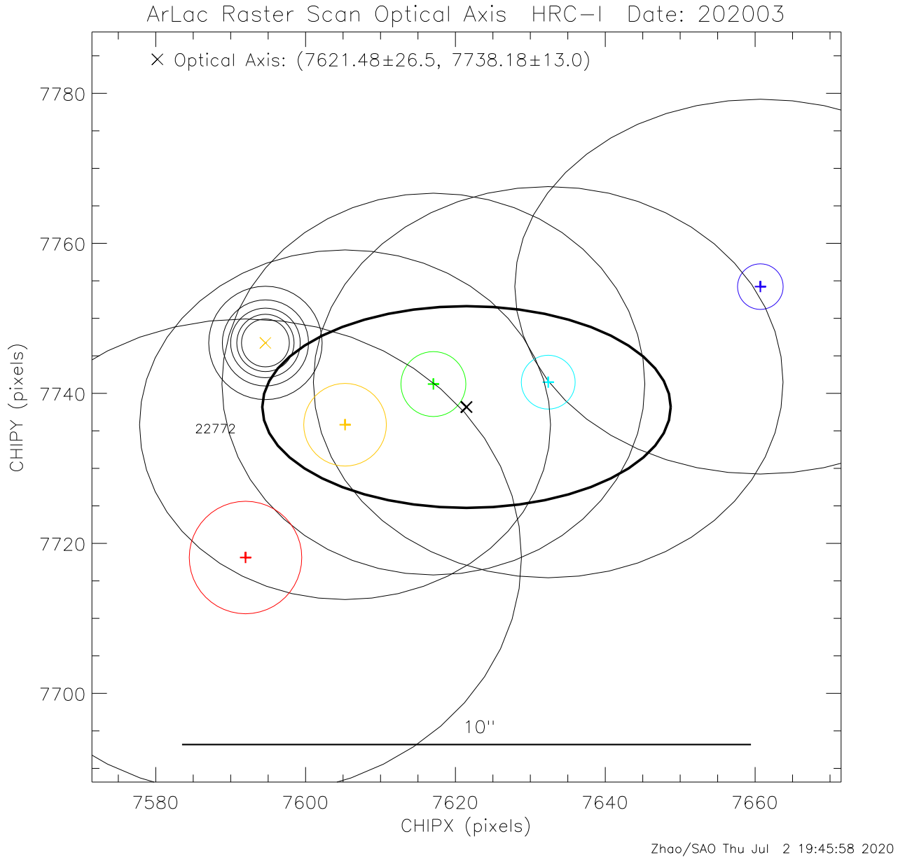
Figure 6: Same as Fig. 4 but zoomed in to the optical axis region. The five colored '+'s are the positions of the quadratic function minimum for 50% – 90% encircled energy fit. The colored circles around them are the 50% – 90% encircled energy radii of the fit. The thin black ovals around them are the 1\text{-}\sigma fit errors. The black × marks the optical axis position, taken as the mean of the above 5 minimums. The thick black oval is the 1\text{-}\sigma error ellipse. The yellow × to the left of the thick black oval and the circles around it are the 5 ks on-axis observation (OBSID 22772) and its 50% – 90% encircled energy radii \times 5 .
