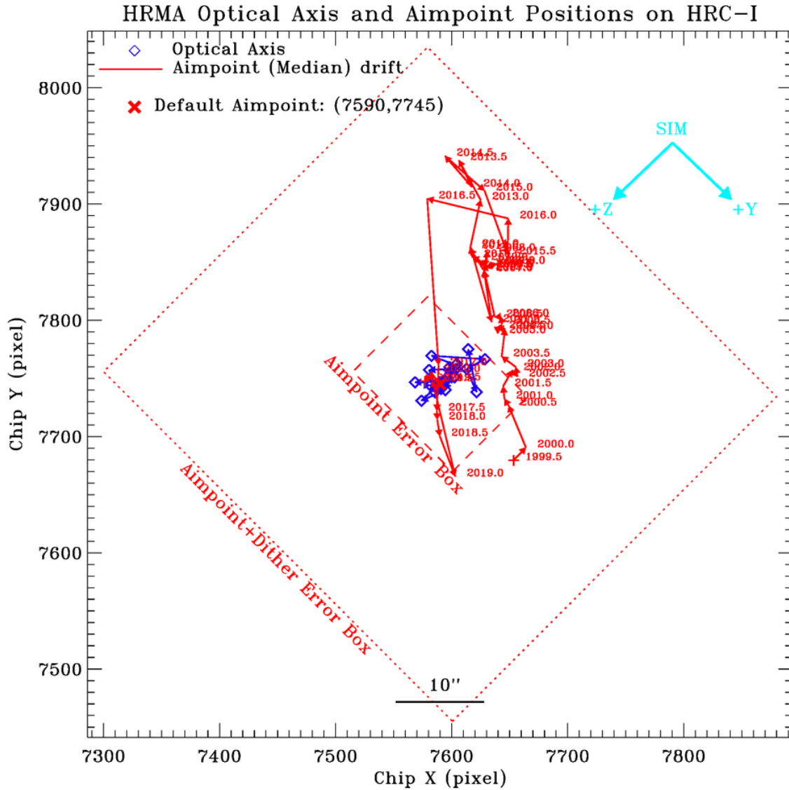
Figure 18: Chandra optical axis (blue) and median aimpoint (red, see Fig. 10) positions in half year bins on HRC-I. Each aimpoint position is labeled by the year. Starting in 2016 (Cycle 18), aimpoint is dynamically adjusted to put at the permanent default position (marked as red “x”) near the optical axis. The dotted and dashed rectangles are the error boxes of the default aimpoint implementation, with and without the dither. The cyan colored arrows show the SIM coordinates.
