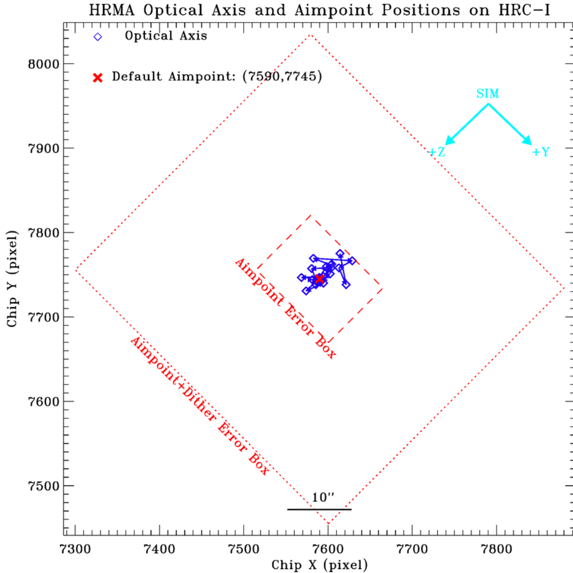
Figure 27: Chandra optical axis (blue diamonds) positions for each year and permanent default aimpoint (red cross) on HRC-I at [7590,7745]. The small box (red dashed line, 16'' \times 12'' , or 121.4 \times 91.1 pixels in SIM [Y, Z]) centered at the permanent default aimpoint is the error box of the effective aimpoint center, i.e. an on-axis target can be anywhere inside this box. The large box (red dotted line, 56'' \times 52'' , or 425.0 \times 394.7 pixels in SIM [Y, Z]) is the error box of effective aimpoint with dither.
