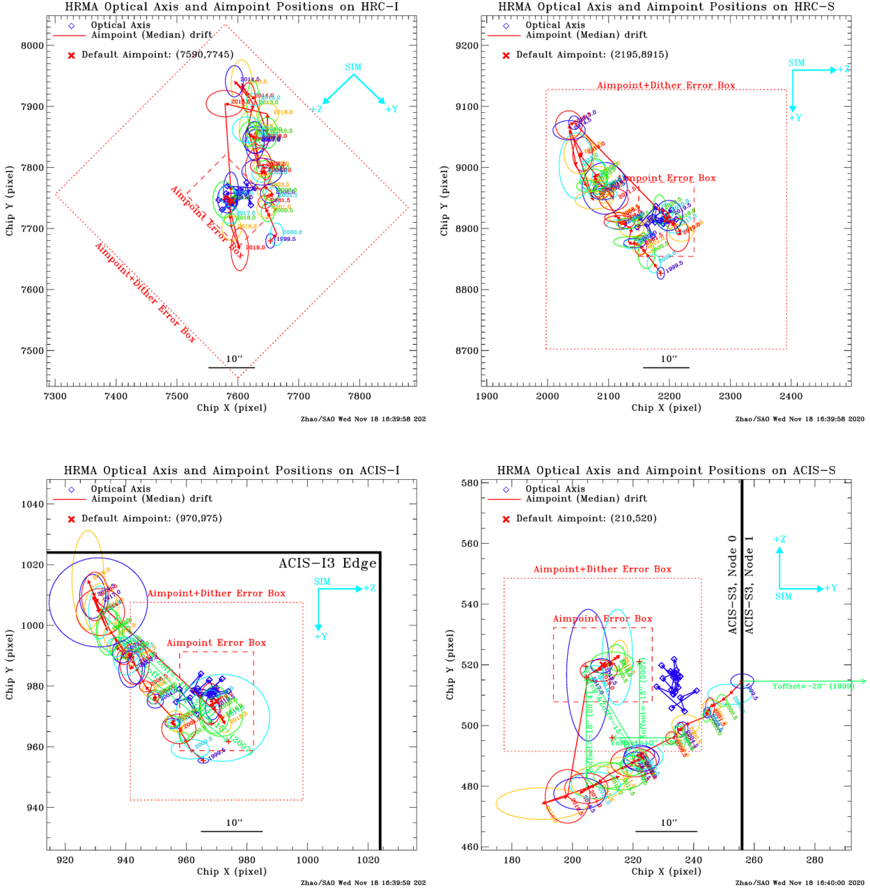
Figure 22: Same as Figures 18 – 21, the optical axis (blue) and median aimpoint (red) drifts on HRC-I (upper-left), HRC-S (upper-right), ACIS-I (lower-left) and ACIS-S (lower-right), with the colored ovals indicating the 1- \sigma error ellipse for data in a given half year bin.
