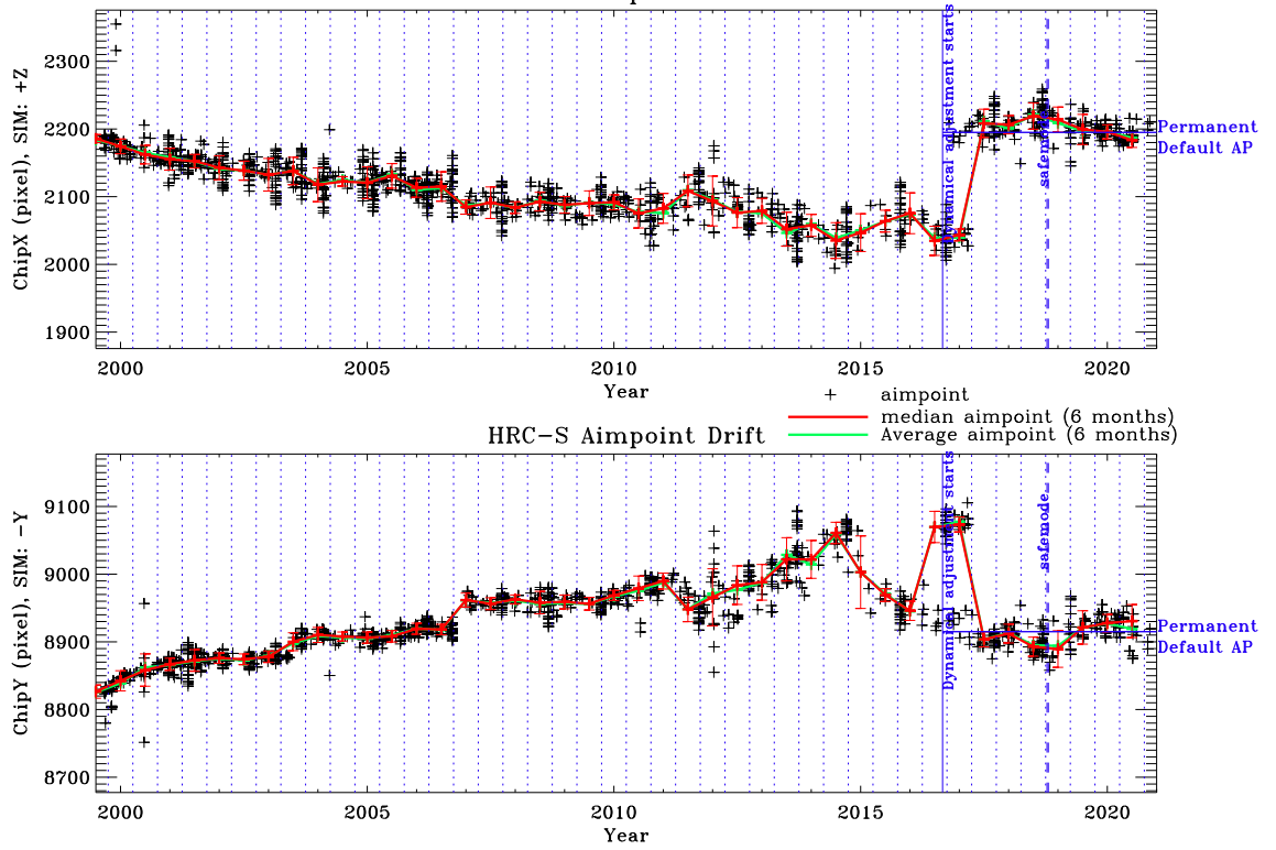
Figure 12: Aimpoint position as a function of time on HRC-S since launch. Solid red (green) lines show the median (average) aimpoint drift in 6 month bins, separated by vertical dotted blue lines. The vertical solid blue line indicates the start of the dynamical aimpoint adjustment.
