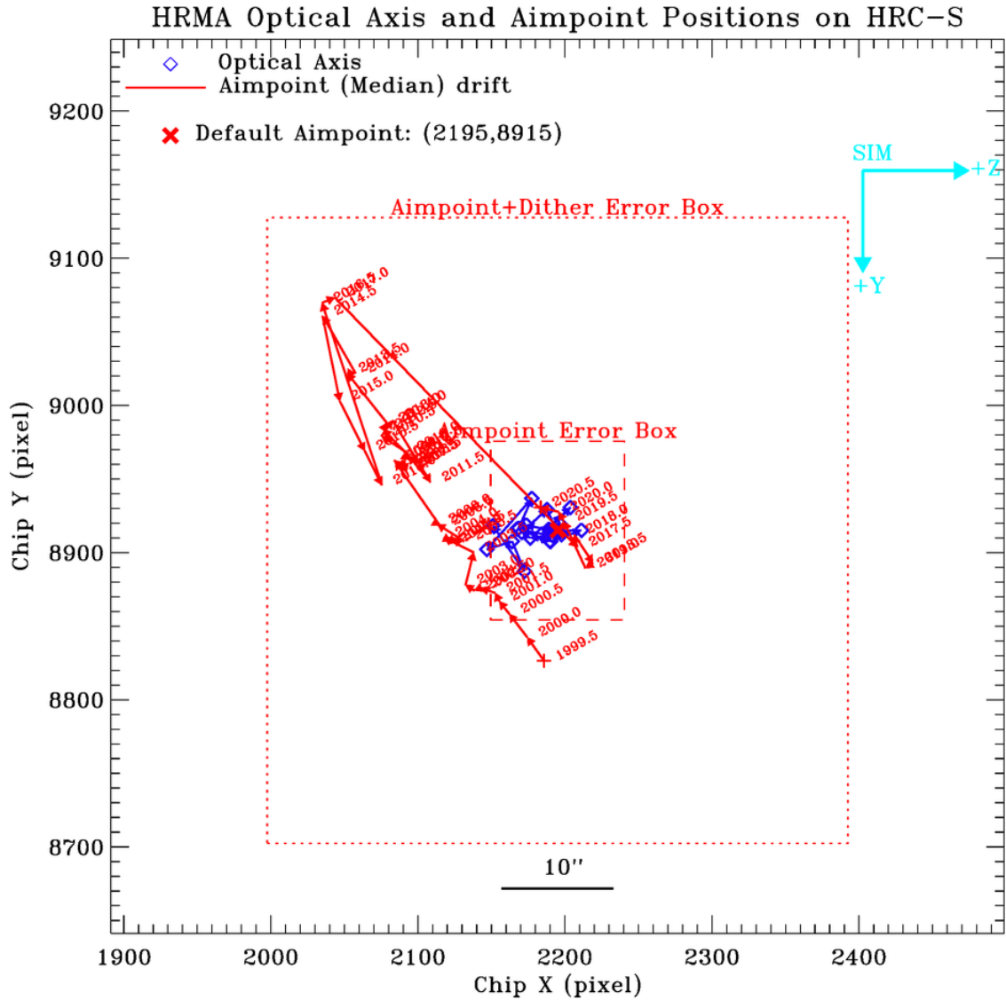
Figure 19: Chandra optical axis (blue) and median aimpoint (red, see Fig. 12) positions in half year bins on HRC-S. Each aimpoint position is labeled by the year. Starting in 2016 (Cycle 18), aimpoint is dynamically adjusted to put at the permanent default position (marked as red “x”) near the optical axis. The dotted and dashed rectangles are the error boxes of the default aimpoint implementation, with and without the dither. The cyan colored arrows show the SIM coordinates.
