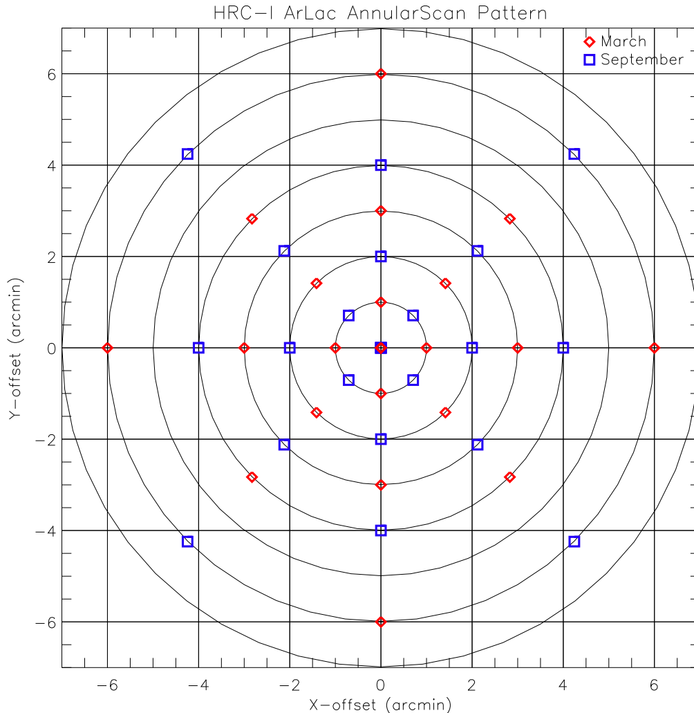
Figure 3: The annular scan pattern of Ar Lac using the HRC-I detector: The red diamond positions are scanned in the spring (March – April); the blue square positions are scanned in the fall (September – October), with 21 observations in each scan. The center (aimpoint) position has 5 ks exposure time; other positions have 1 ks exposure time.
