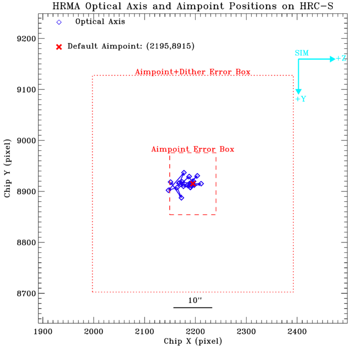
Figure 28: Chandra optical axis (blue diamonds) positions for each year and permanent default aimpoint (red cross) on HRC-S at [2195,8915]. The small box (red dashed line, 12'' \times 16'' , or 91.1 \times 121.4 pixels) centered at the permanent default aimpoint is the error box of the effective aimpoint center, i.e. an on-axis target can be anywhere inside this box. The large box (red dotted line, 52'' \times 56'' , or 394.7 \times 425.0 pixels) is the error box of effective aimpoint with dither.
