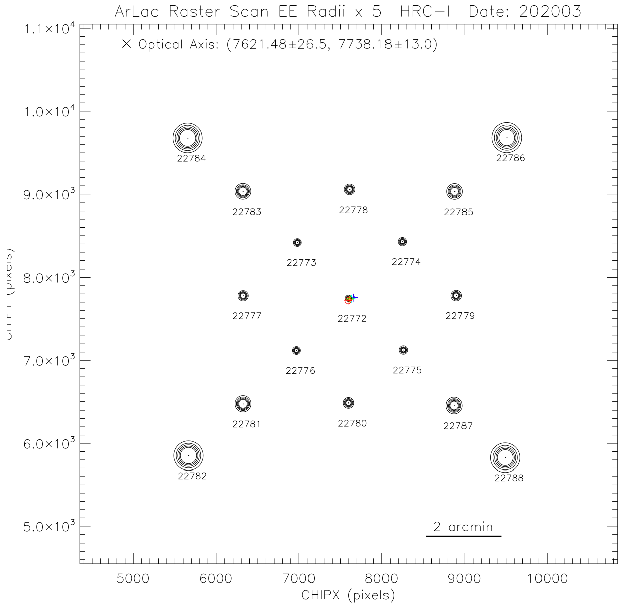
Figure 4: HRC-I annular scan observation of Ar Lac in chip coordinates. Circles around each observation point have the 50% – 90% encircled energy radii \times 5 . The data are fit to a 2-D quadratic function to find the optical axis. Data taken in March 2020. The numbers under the circles are the OBSIDs of the observations.
