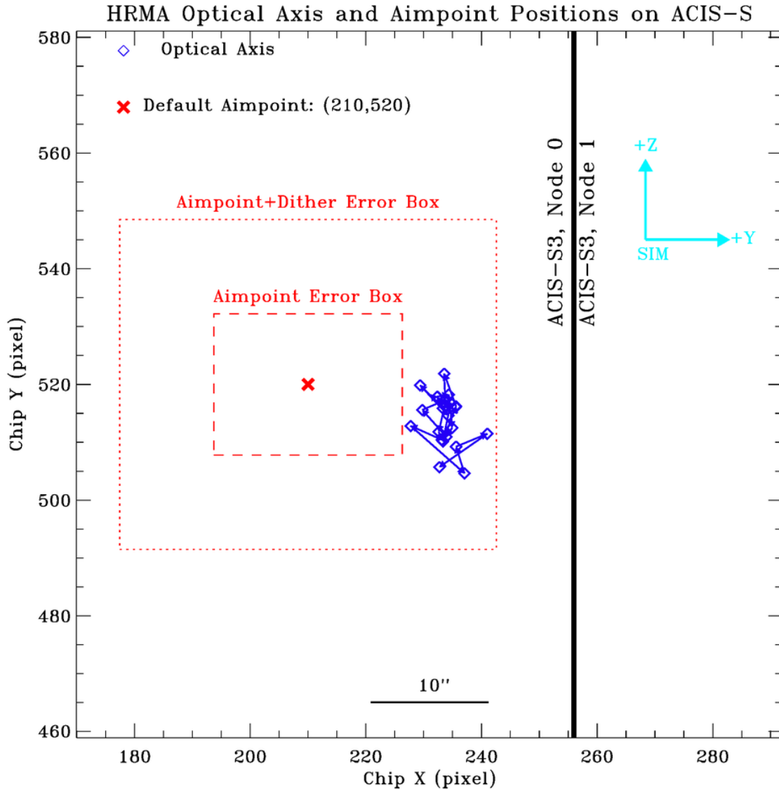
Figure 26: Chandra optical axis (blue diamonds) positions for each year and permanent default aimpoint (red cross) on ACIS-S at [210,520]. The small box (red dashed line, 16'' \times 12'' , or 32.5 \times 24.4 pixels) centered at the permanent default aimpoint is the error box of the effective aimpoint center, i.e. an on-axis target can be anywhere inside this box. The large box (red dotted line, 32'' \times 28'' , or 65.0 \times 56.9 pixels) is the error box of effective aimpoint with dither. Note the permanent default aimpoint is \sim 12'' from the optical axis in order to avoid the node boundary 0|1.
