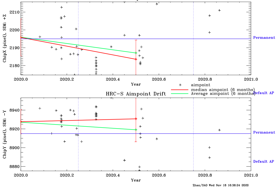
Figure 13: Aimpoint position as a function of time on HRC-S in the past year.
