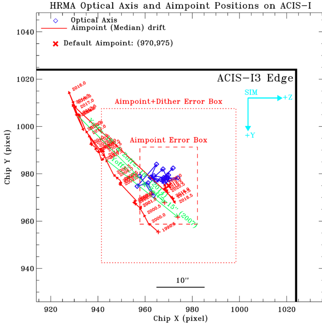
Zhao/SAO Wed Nov 18 16:39:59 2020 Figure 20: Chandra optical axis (blue) and median aimpoint (red, see Fig. 14) positions in half year bins on ACIS-I. Each aimpoint position is labeled by the year. The green arrows in the figure show the default offsets (starting in the year labels next to the green arrows) applied before 2016. All the observations were conducted with these default offsets, unless the observers requested otherwise. Starting in 2016 (Cycle 18), aimpoint is dynamically adjusted to put at the permanent default position (marked as red “x”) near the optical axis. The dotted and dashed rectangles are the error boxes of the default aimpoint implementation, with and without the dither. The cyan colored arrows show the SIM coordinates.
