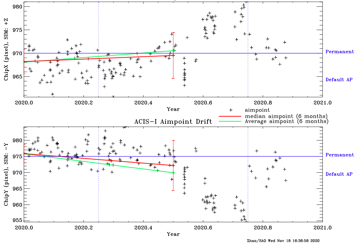
Figure 15: Aimpoint position as a function of time on ACIS-I in the past year.
