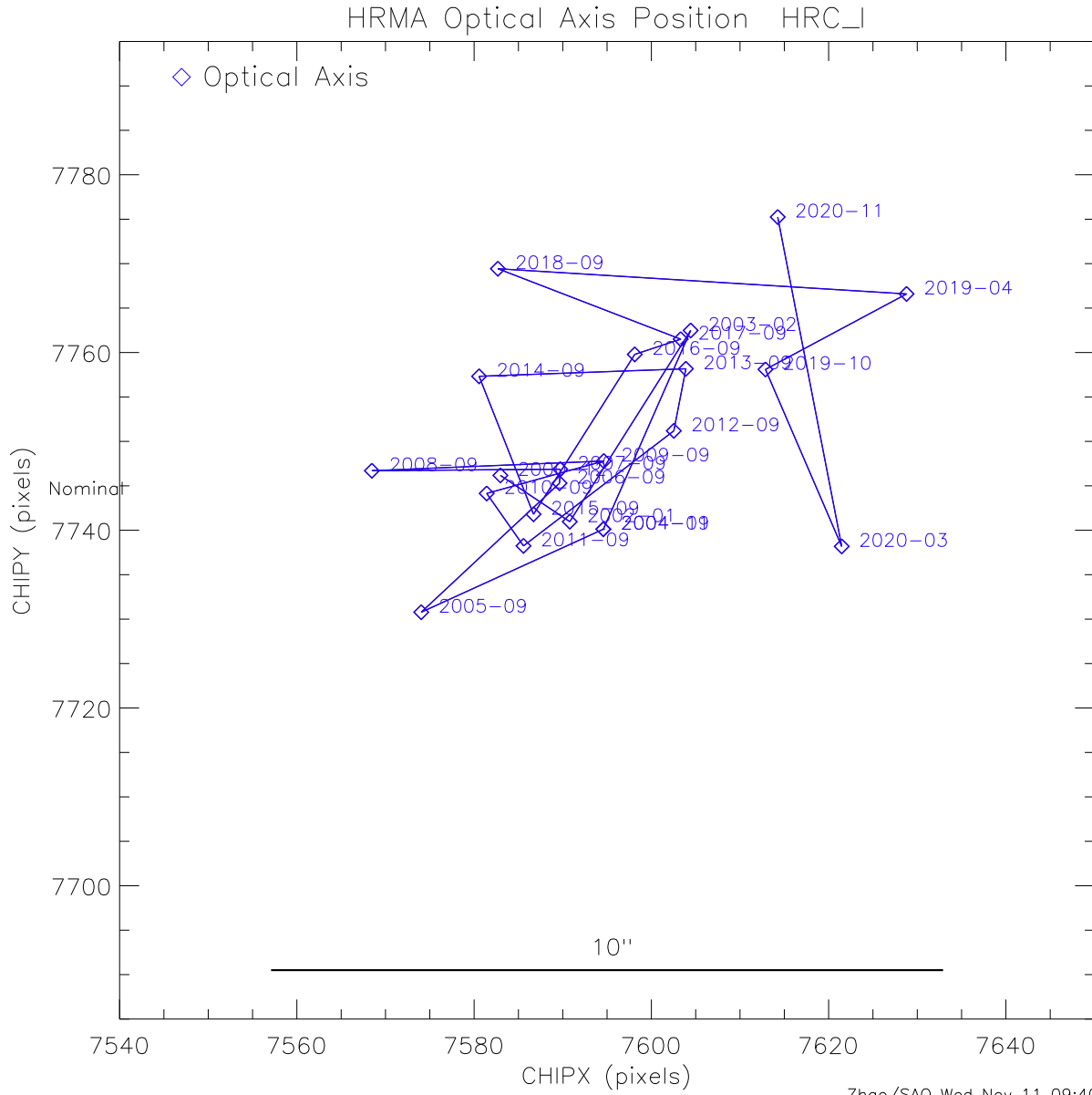
Figure 9: Same as Figure 8 with error ellipses removed for clarity.
