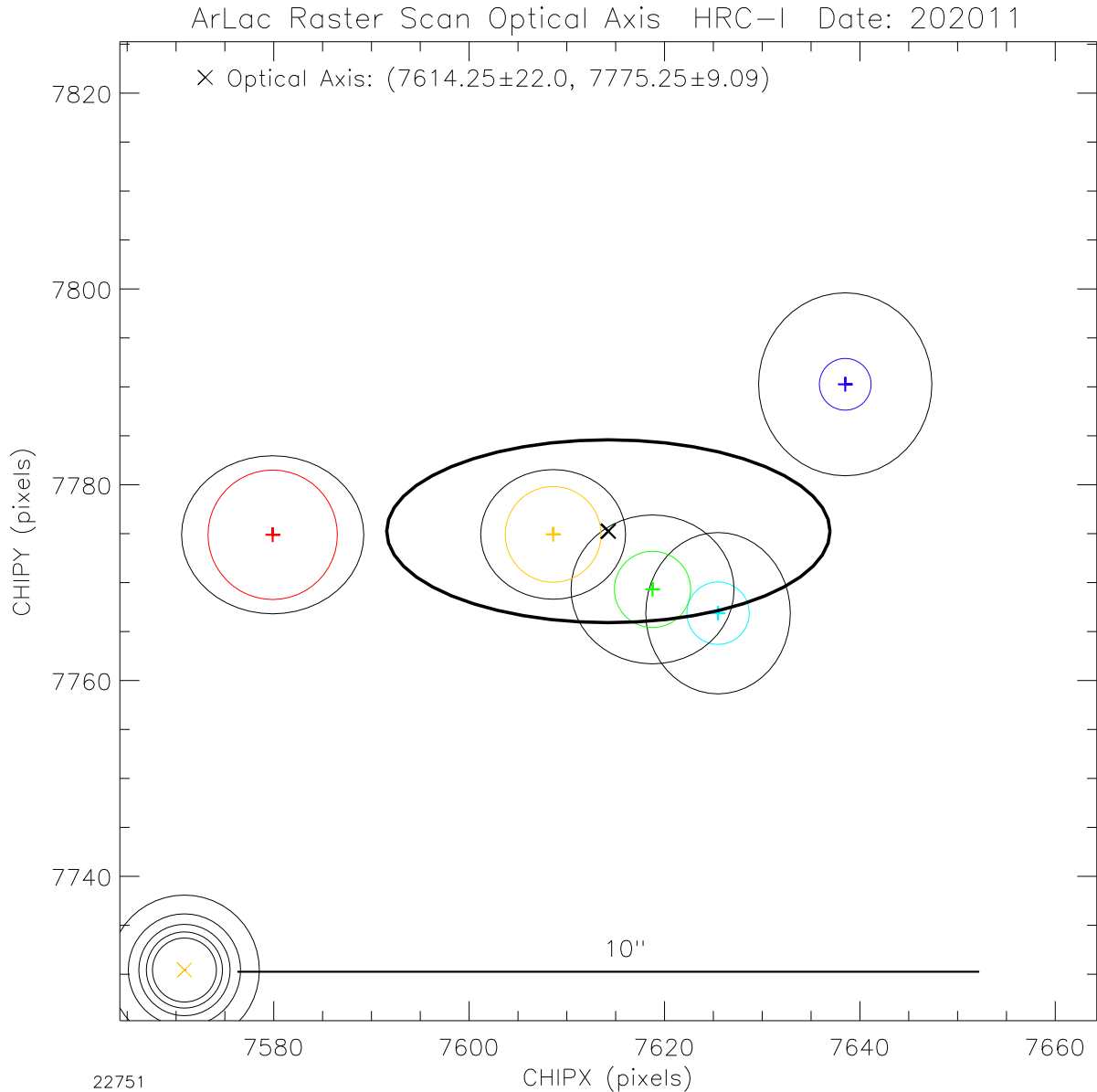
Figure 7: Same as Fig. 5 but zoomed in to the optical axis region. The five colored +’s are the positions of the quadratic function minimum for 50% – 90% encircled energy fit. The colored circles around them are the 50% – 90% encircled energy radii of the fit. The thin black ovals around them are the 1- \sigma fit errors. The black \times marks the optical axis position, taken as the mean of the above 5 minima. The thick black oval is the 1- \sigma error ellipse. The yellow \times at the lower left corner and the circles around it are the 5 ks on-axis observation (OBSID 22751) and its 50% – 90% encircled energy radii \times 5 .
