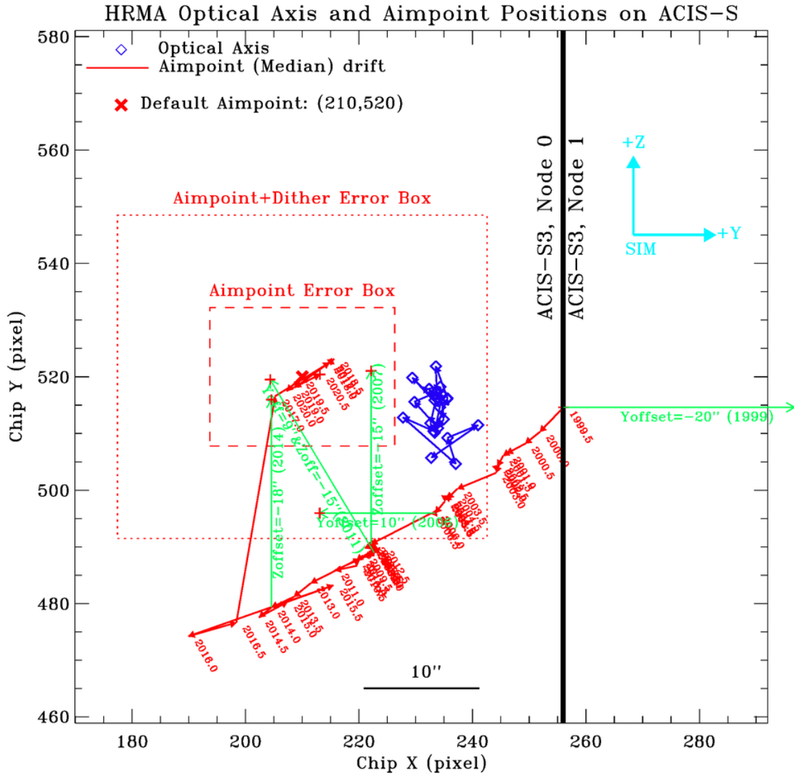
Figure 21: Chandra optical axis (blue) and median aimpoint (red, see Fig. 16) positions in half year bins on ACIS-S. Each aimpoint position is labeled by the year. The green arrows in the figure show the default offsets (starting in the year labels next to the green arrows) applied before 2016. All the observations were conducted with these default offsets, unless the observers requested otherwise. Starting in 2016 (Cycle 18), aimpoint is dynamically adjusted to put at the permanent default position (marked as red “x”) near the optical axis. The dotted and dashed rectangles are the error boxes of the default aimpoint implementation, with and without the dither. The cyan colored arrows show the SIM coordinates.
