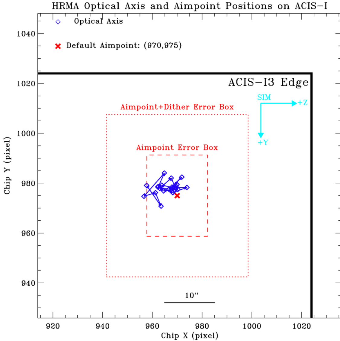
Figure 25: Chandra optical axis (blue diamonds) positions for each year and permanent default aimpoint (red cross) on ACIS-I at [970,975]. The small box (red dashed line, 12'' \times 16'' , or 24.4 \times 32.5 pixels) centered at the permanent default aimpoint is the error box of the effective aimpoint center, i.e. an on-axis target can be anywhere inside this box. The large box (red dotted line, 28'' \times 32'' , or 56.9 \times 65.0 pixels) is the error box of effective aimpoint with dither.
