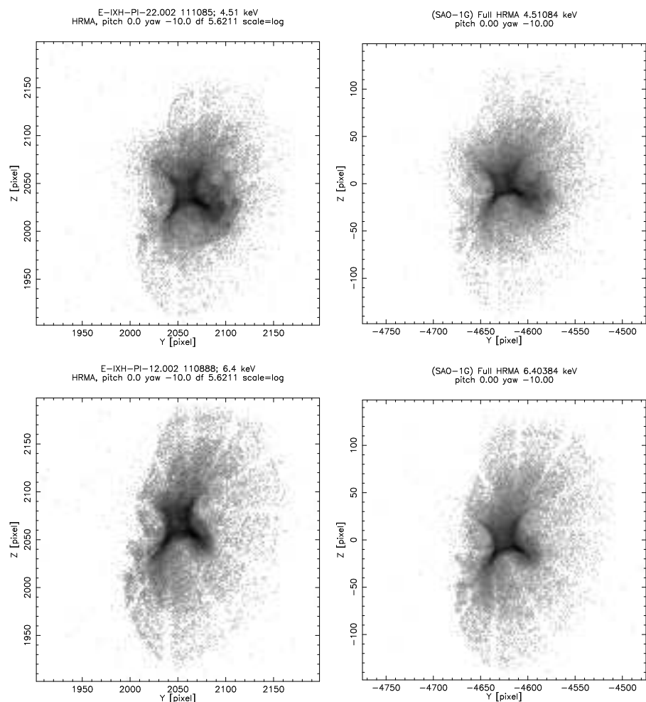
Figure 22.3: Top left: hsi110885i0 X-ray image; 10' off-axis, Ti-K \alpha . ( 2 \times 2 HSI pixels.) Top right: Raytrace; 10' off-axis, Ti-K \alpha . ( 2 \times 2 HSI pixels.) Bottom left: hsi110888i0 X-ray image; 10' off-axis, Fe-K \alpha . ( 2 \times 2 HSI pixels.) Bottom right: Raytrace; 10' off-axis, Fe-K \alpha . ( 2 \times 2 HSI pixels.) The images are log stretched.
