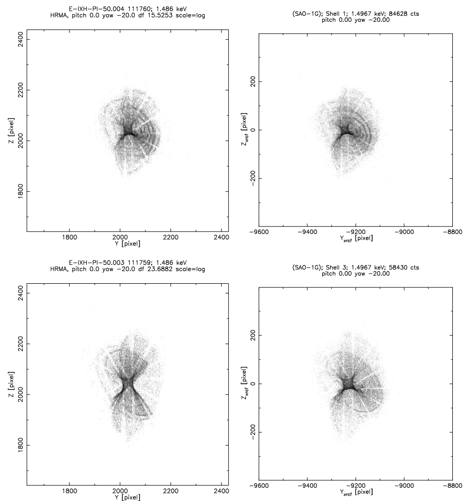
Figure 22.13: Top left: hsi111760i0 X-ray image; shell 1, 20' off-axis, Al-K \alpha . ( 2 \times 2 HSI pixels.) Top right: Raytrace; shell 1, 20' off-axis, Al-K \alpha . ( 2 \times 2 HSI pixels.) Bottom left: hsi111759i0 X-ray image; shell 3, 20' off-axis, Al-K \alpha . ( 2 \times 2 HSI pixels.) Bottom right: Raytrace; shell 3, 20' off-axis, Al-K \alpha . ( 2 \times 2 HSI pixels.) The images are log stretched.
