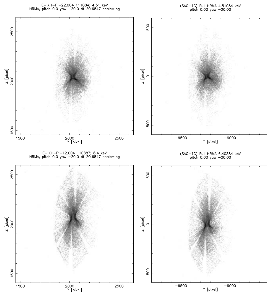
Figure 22.6: Top left: hsi111084i0 X-ray image; 20' off-axis, Ti-K \alpha . ( 4 \times 4 HSI pixels.) Top right: Raytrace; 20' off-axis, Ti-K \alpha . ( 4 \times 4 HSI pixels.) Bottom left: hsi110887i0 X-ray image; 20' off-axis, Fe-K \alpha . ( 4 \times 4 HSI pixels.) Bottom right: Raytrace; 20' off-axis, Fe-K \alpha . ( 4 \times 4 HSI pixels.) The images are log stretched.
