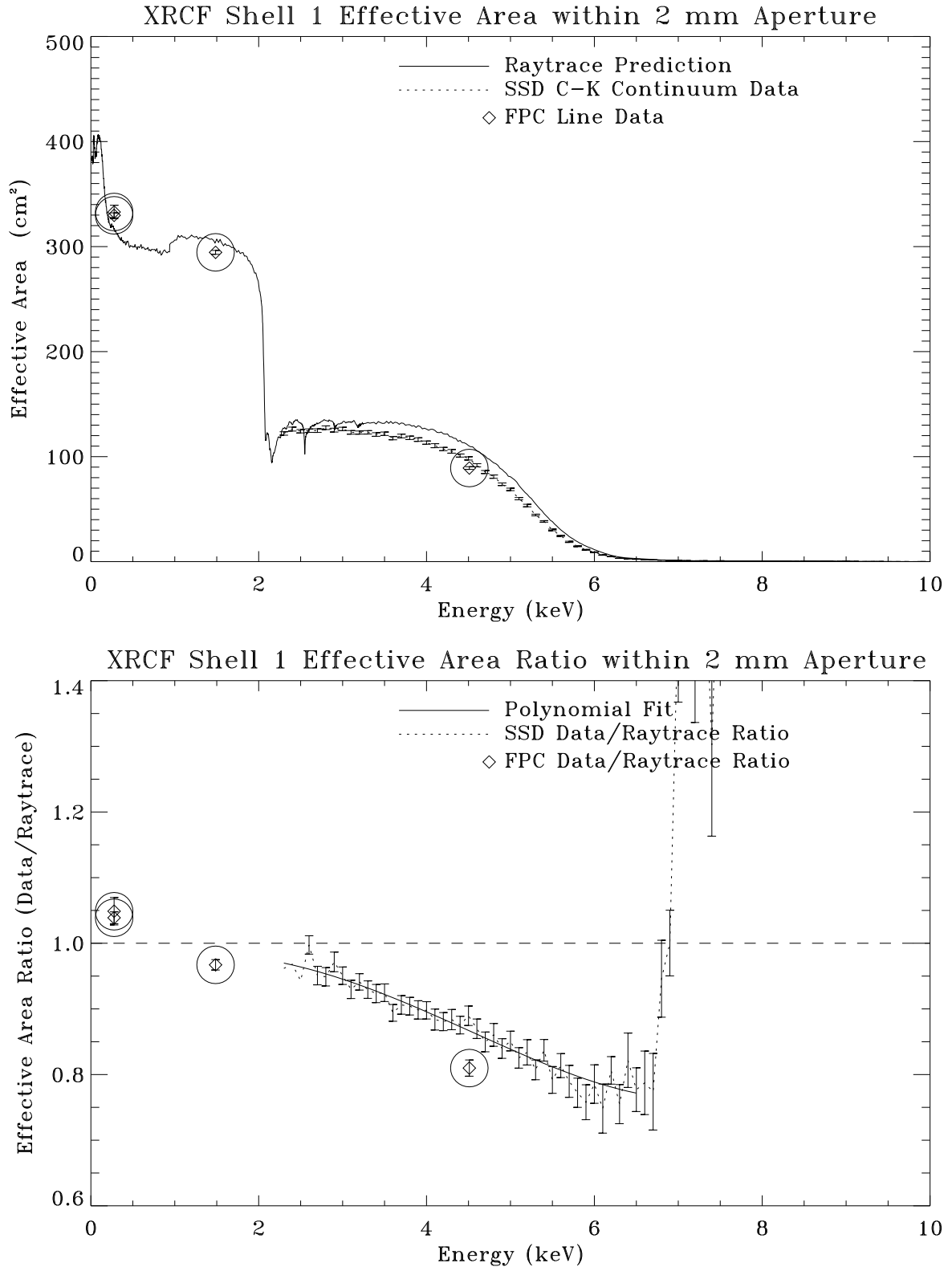
Figure 11.36: Calibration data vs. raytrace prediction. Top panel shows the XRCF Shell 1 effective area within 2 mm aperture. Bottom panel shows the effective area ratio of data/raytrace.
