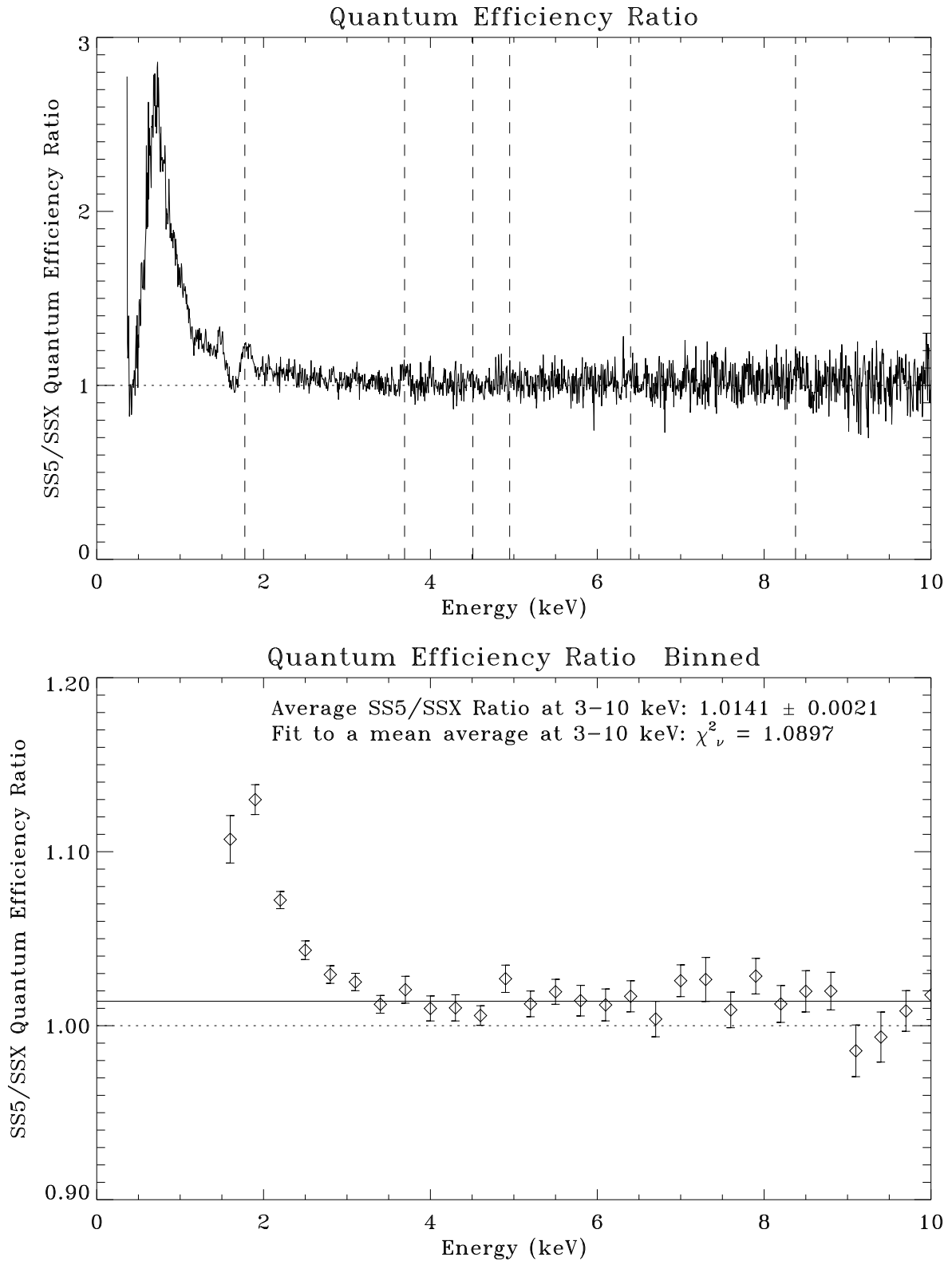
Figure 11.28: SS5/SSX quantum efficiency ratio. In the top panel, the large ratio below 2 keV is mainly due to the different ice build up on the two detectors. The bottom panel shows the ratio curve binned and fitted to a constant ratio. The solid line is the average ratio at 3–10 keV.
