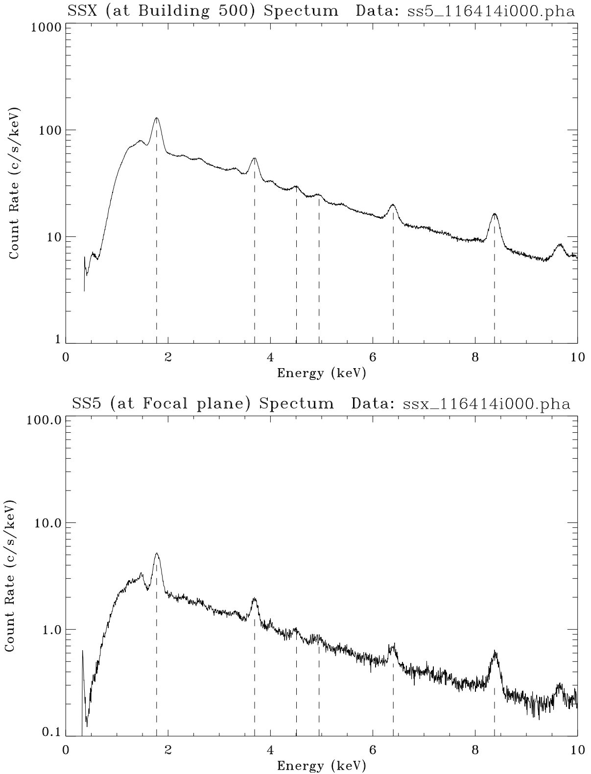
Figure 11.20: C-continuum flat field test SSX and SS5 spectra as functions of energy, using energy scales from Figure 11.18.
