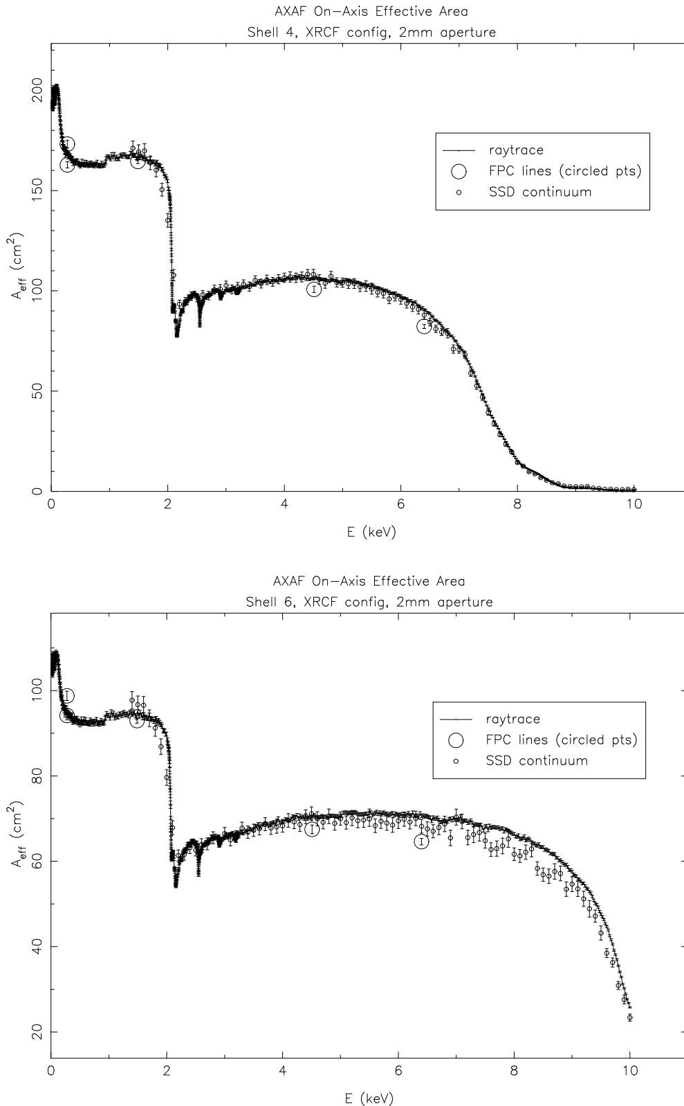
Figure 12.5: Measurements and Ray traces for effective area through 2 mm pinholes for shells 4 and 6. Both fpc_ and SSD continuum measurements are shown.
