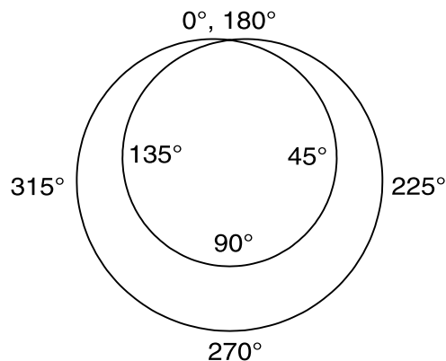
Figure 28.1: Schematic of coma circle ( 2\theta ) image distortion. The limaçon is the pattern of the photons at the focal surface. The angles refer to the azimuth of the optic at which the photons were reflected.
