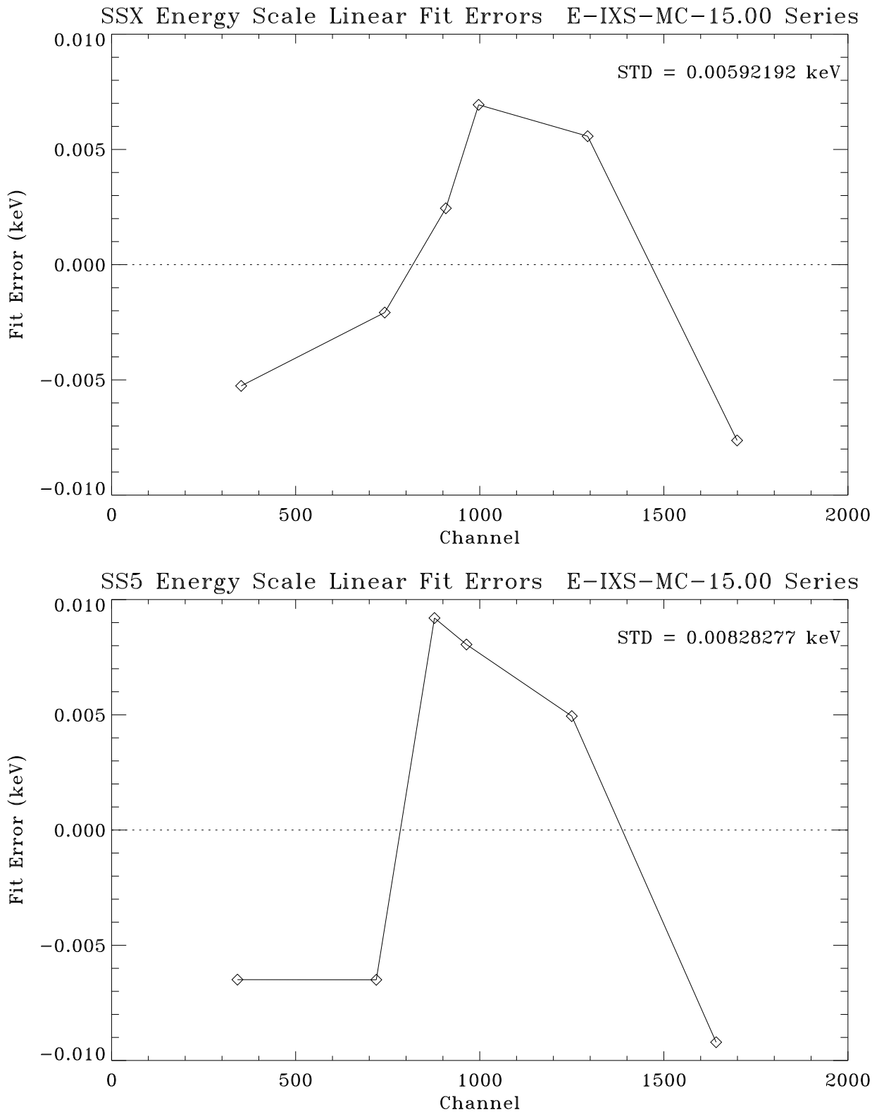
Figure 11.22: SSX and SS5 energy scale linear fit residuals for the C-continuum effective area measurements (Phase-E).
