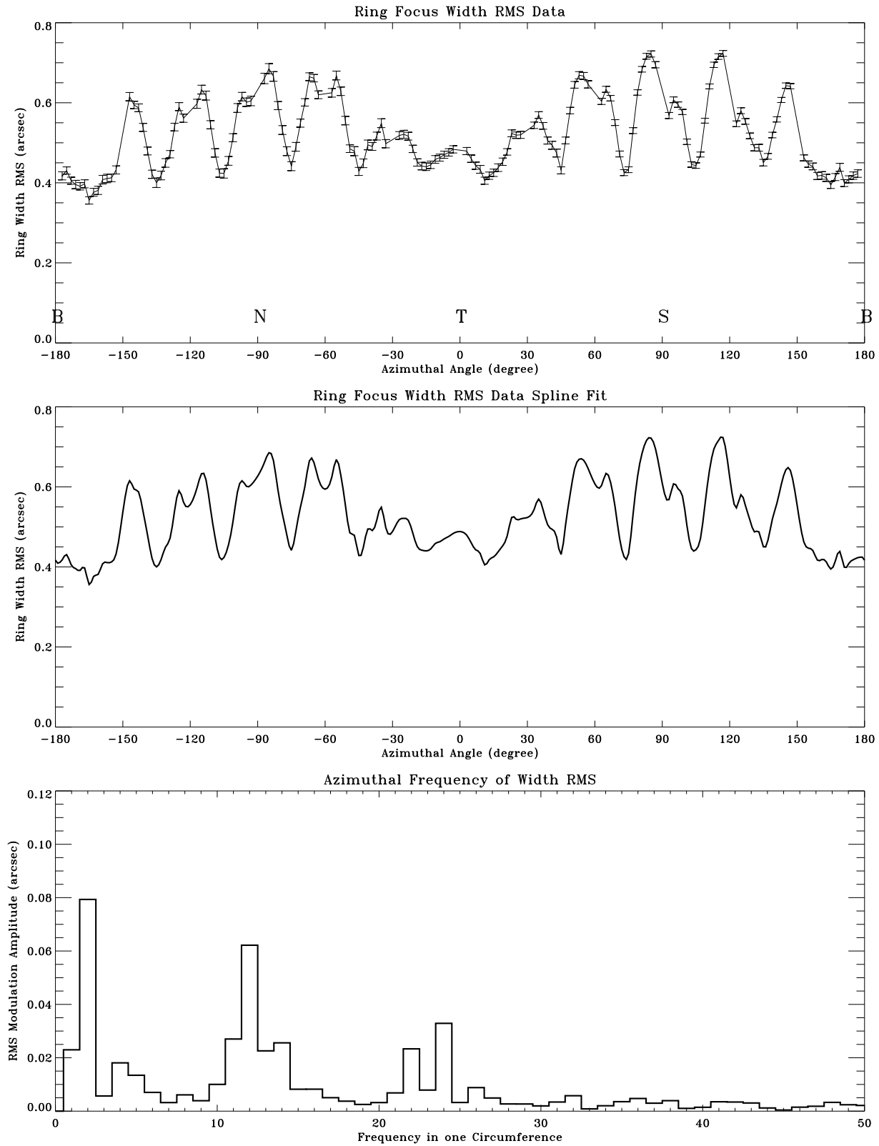
Figure 18.13: The Ring width RMS for ring 4. Date: 1997/01/24; TRW ID: D-IXH-RF-1.005; Run ID: 110004; Source: A1-K; Defocus: 65.2 mm.
