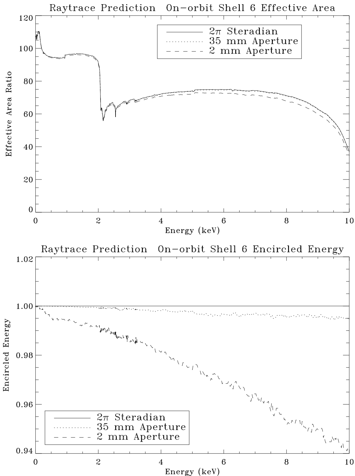
Figure 11.49: Raytrace prediction of on-orbit Shell 6 effective area and encircled energy. Top panel shows the effective area curves within 2 mm, 35 mm apertures, and 2\pi steradian. Bottom panel shows the encircled energies of 2 mm and 35 mm apertures as fractions of that within 2\pi steradian.
