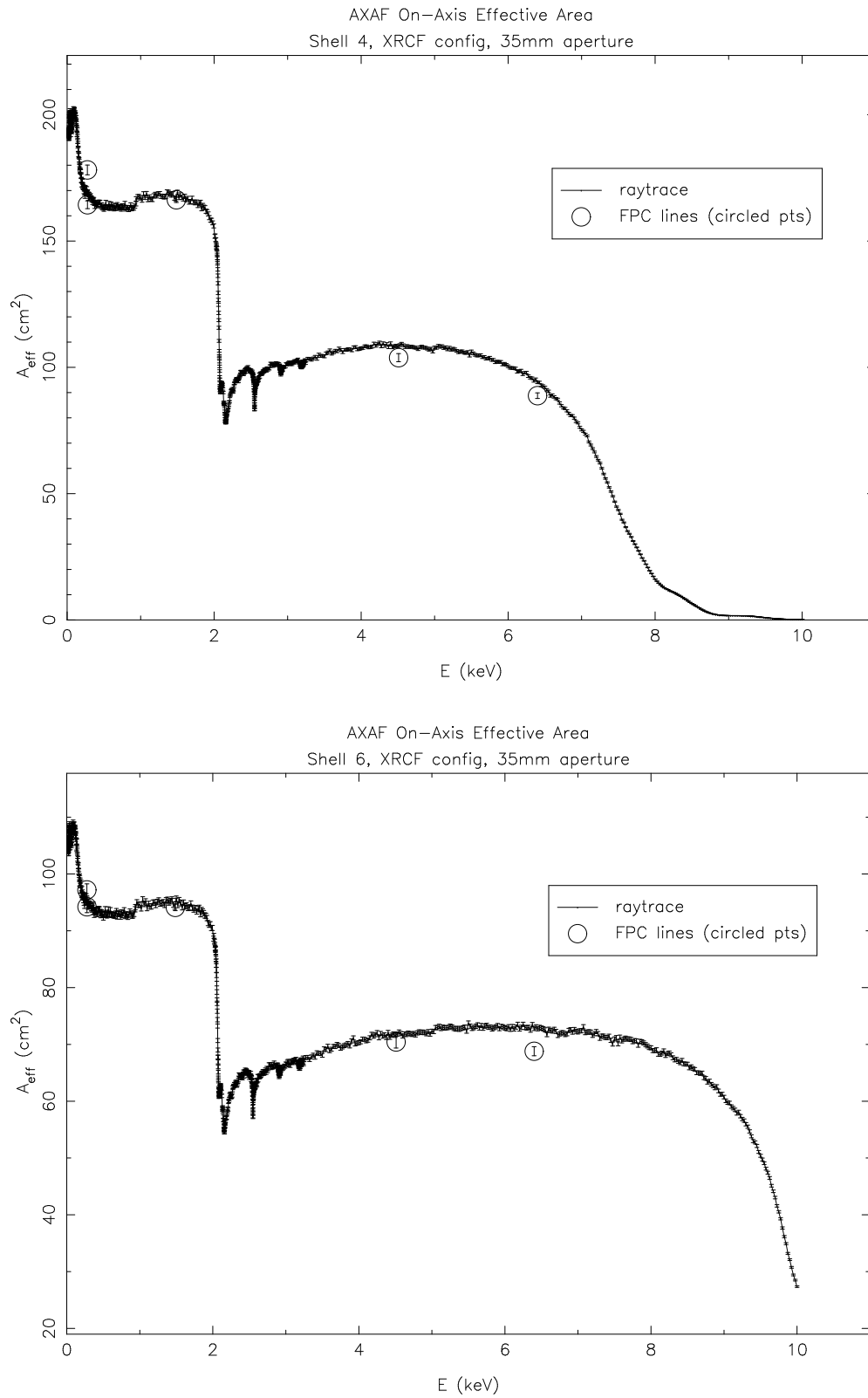
Figure 12.2: Measurements and Ray traces for effective area through 35 mm pinholes for shells 4 and 6.
