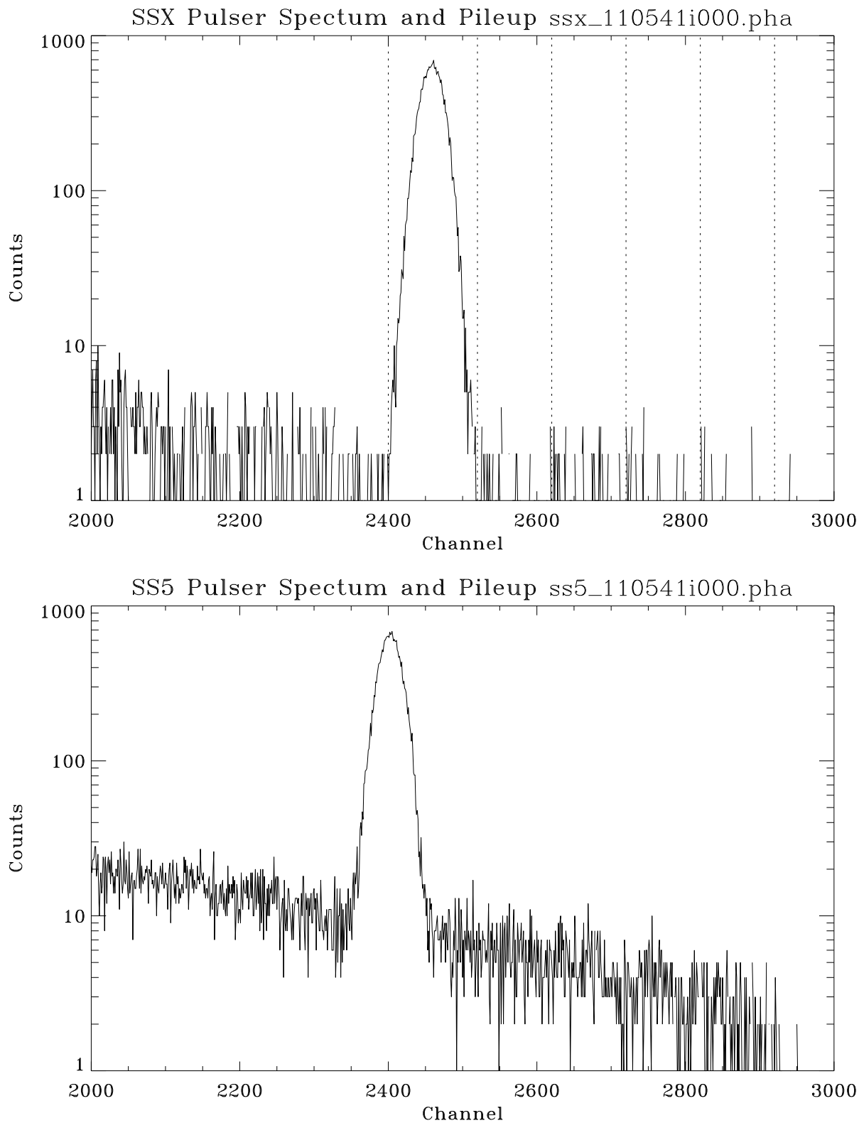
Figure 11.7: SSX and SS5 pulser spectra: Shell 4; Run ID: 110541. Counts to the right of the SSX pulser peak are mainly due to pileups from the pulser, a small amount are due to pileups from the continuum.
