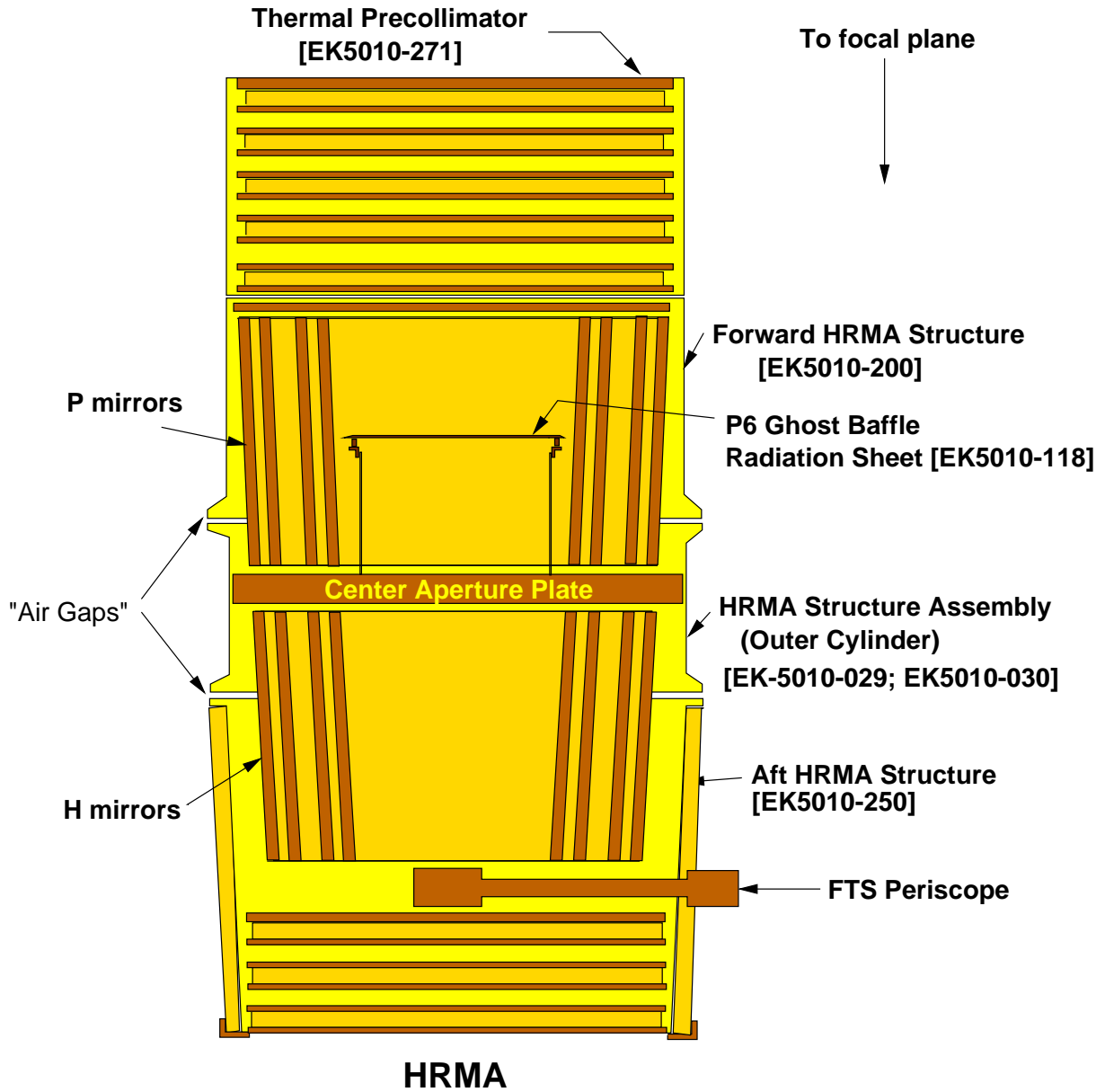
Figure E.1: Schematic of relevant HRMA assemblies
