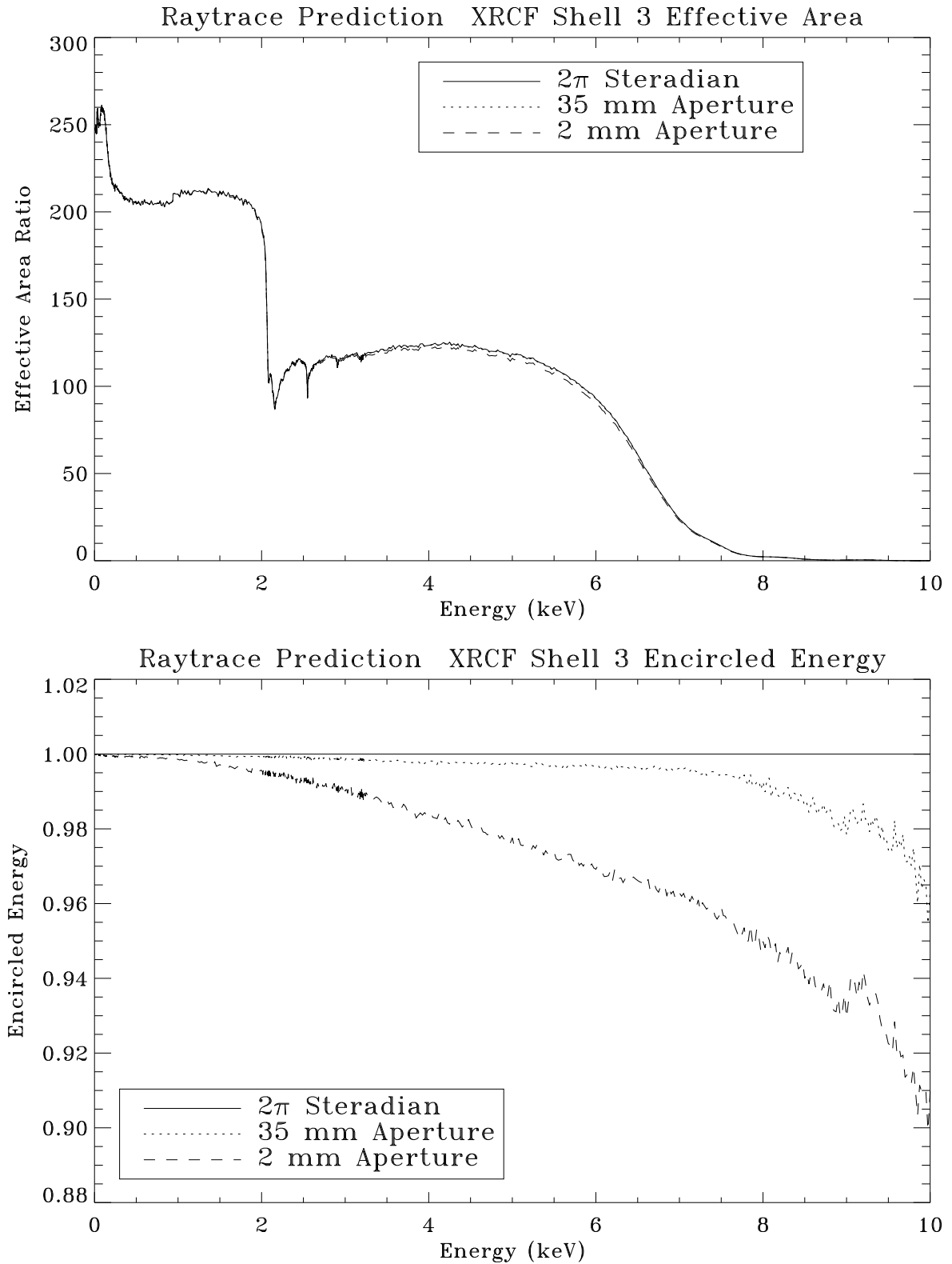
Figure 11.42: Raytrace prediction of XRCF Shell 3 effective area and encircled energy. Top panel shows the effective area curves within 2 mm, 35 mm apertures, and 2\pi steradian. Bottom panel shows the encircled energies of 2 mm and 35 mm apertures as fractions of that within 2\pi steradian.
