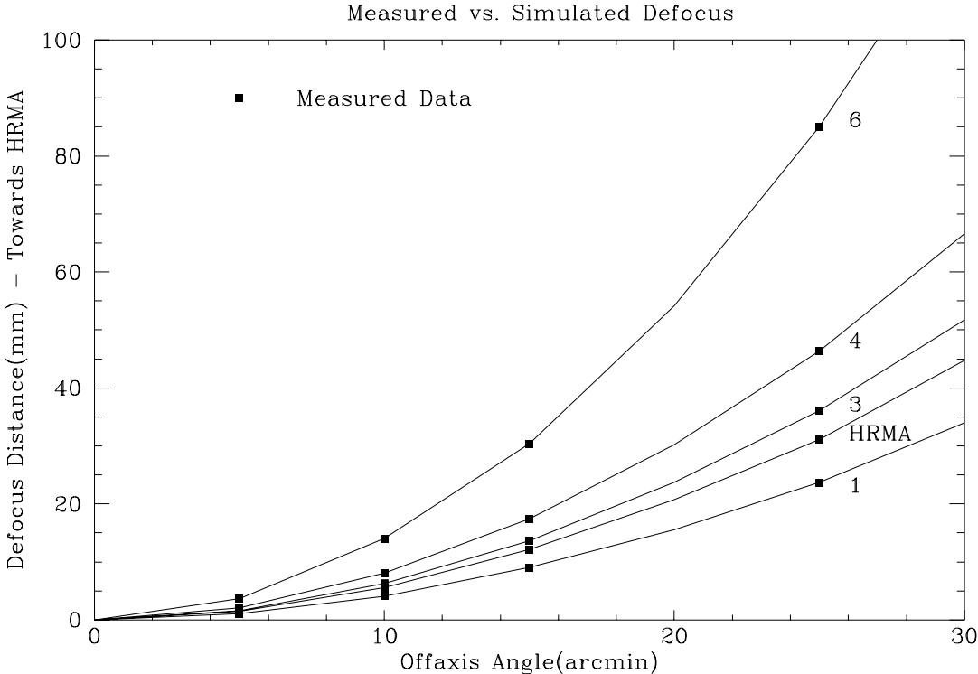
Figure 29.1: Measured vs. Simulated Off-Axis Focus Data
