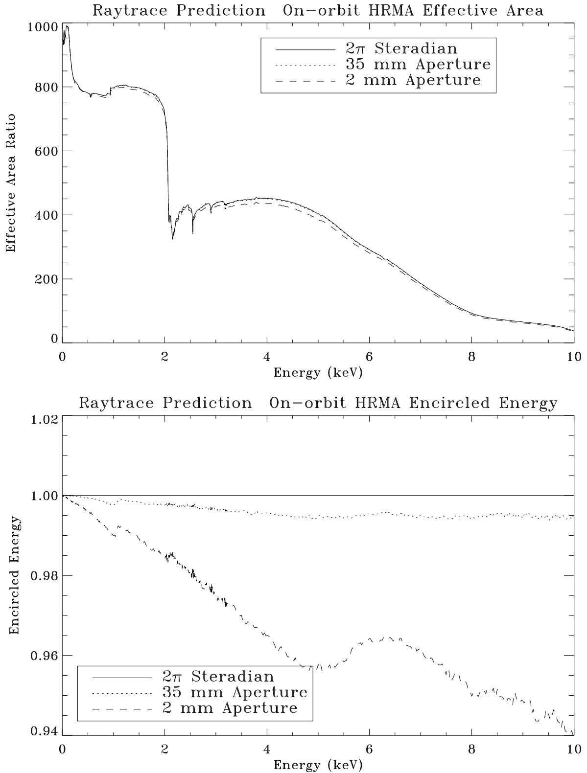
Figure 11.50: Raytrace prediction of on-orbit HRMA effective area and encircled energy. Top panel shows the effective area curves within 2 mm, 35 mm apertures, and 2\pi steradian. Bottom panel shows the encircled energies of 2 mm and 35 mm apertures as fractions of that within 2\pi steradian.
