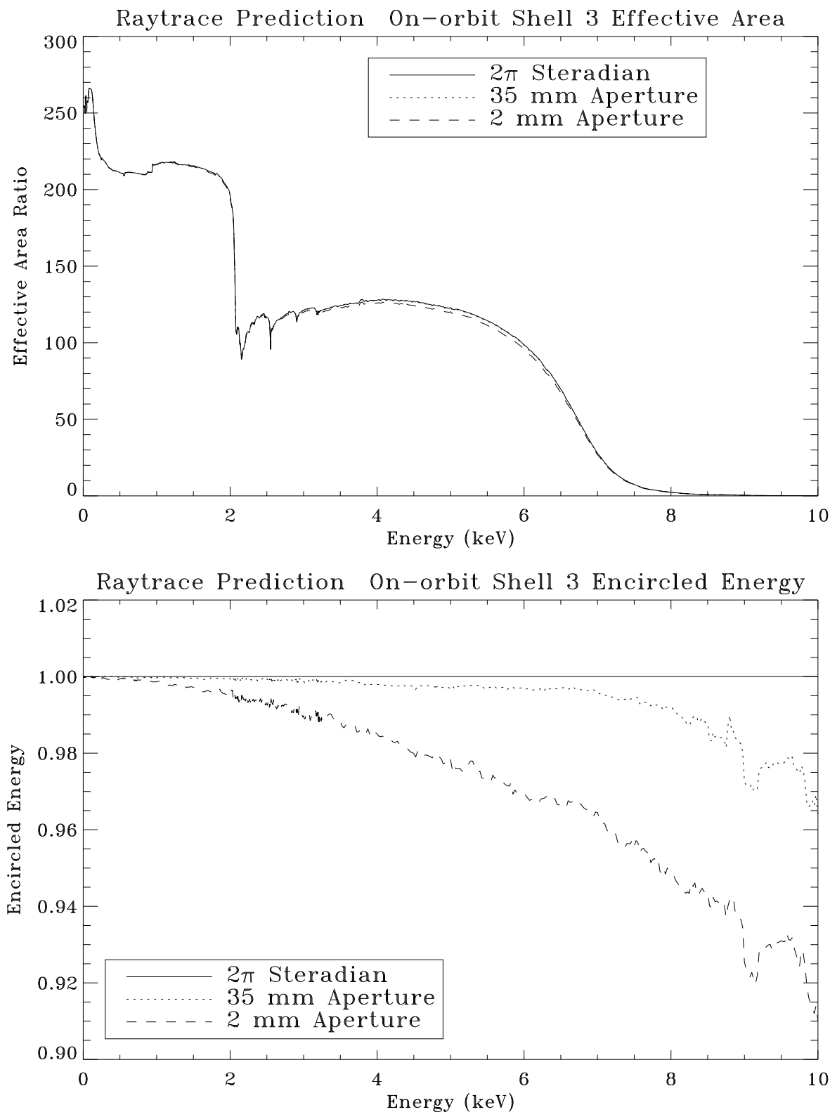
Figure 11.47: Raytrace prediction of on-orbit Shell 3 effective area and encircled energy. Top panel shows the effective area curves within 2 mm, 35 mm apertures, and 2\pi steradian. Bottom panel shows the encircled energies of 2 mm and 35 mm apertures as fractions of that within 2\pi steradian.
