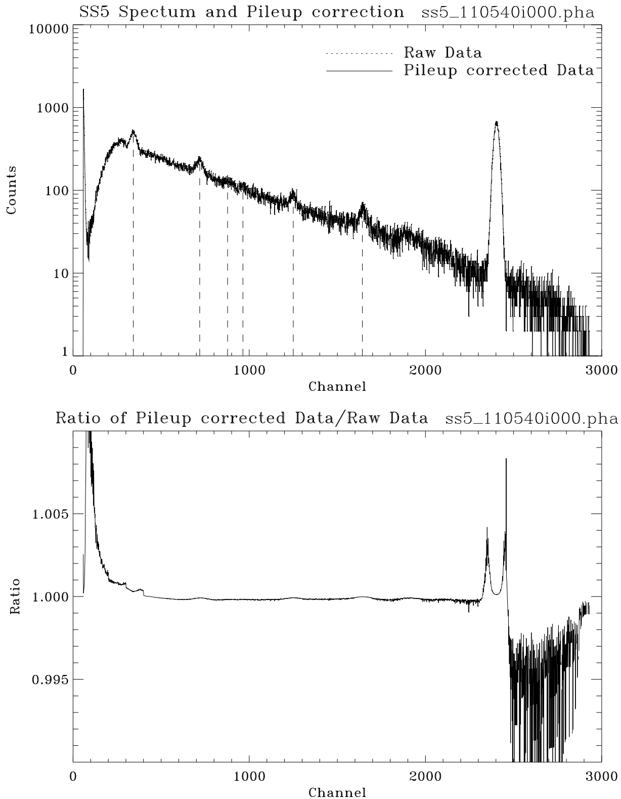
Figure 11.14: SS5 spectrum and pileup correction: Shell 3; Run ID: 110540. Upper panel shows the raw data and pileup corrected data. Dashed vertical lines indicate the X-ray lines to be used to calibrate the energy scale. Lower panel shows the ratio of pileup corrected data to the raw data.
