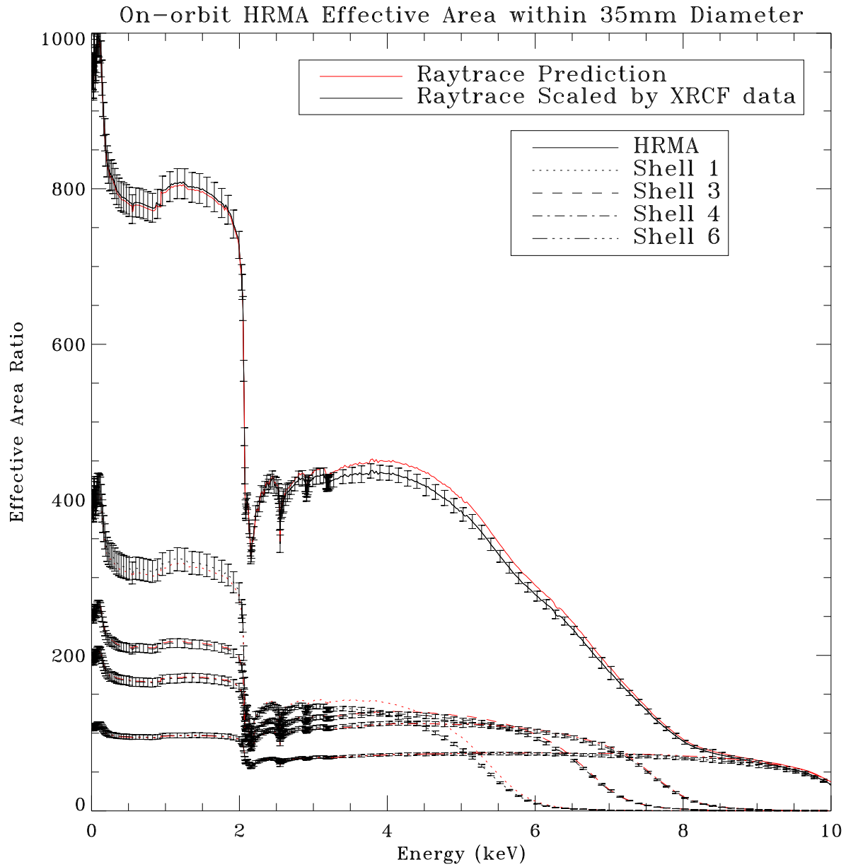
Figure 11.55: The on-orbit HRMA and four shells effective areas within 35 mm aperture. The original raytrace predictions and the calibration data scaled raytrace predictions.
