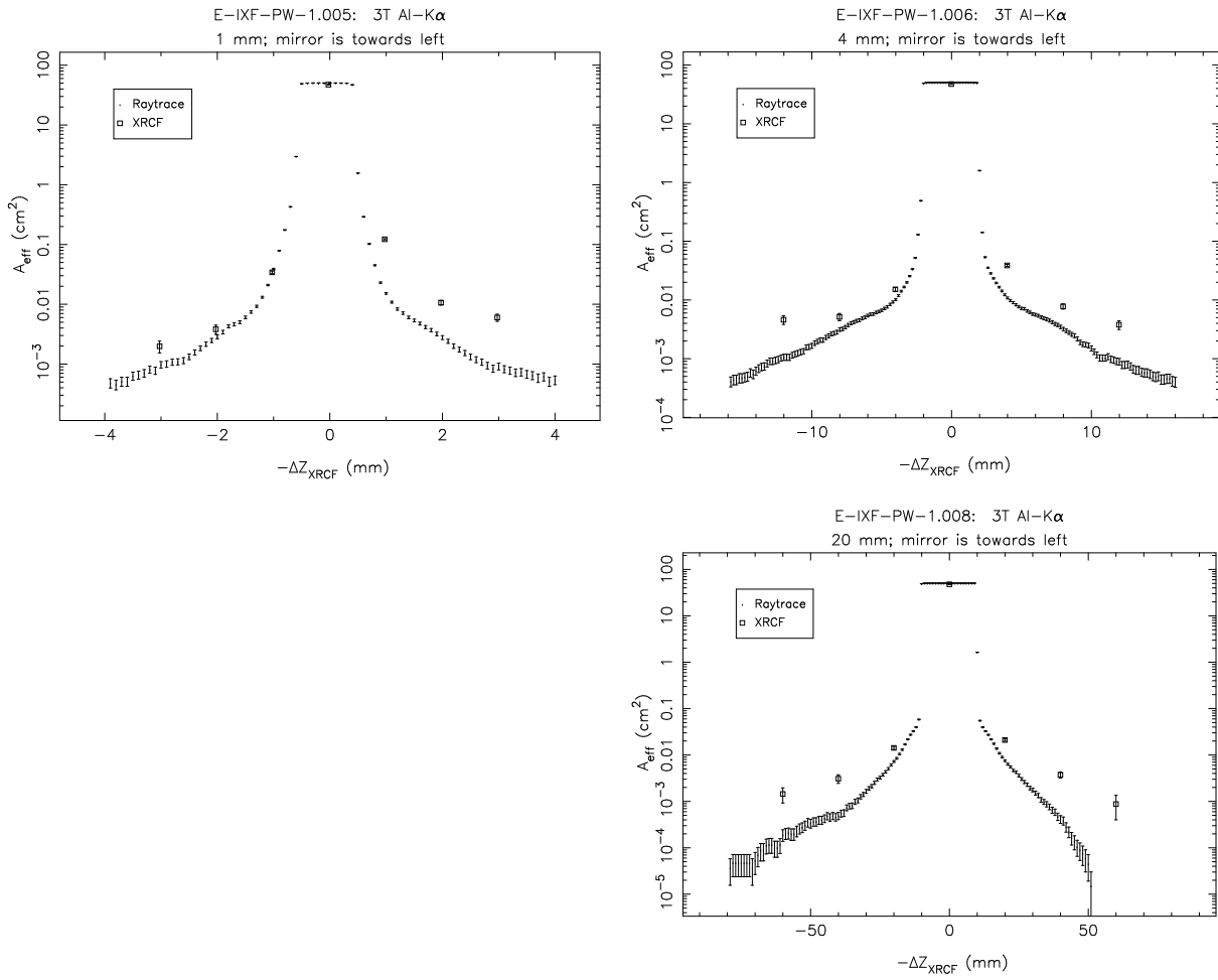
Figure 14.12: Pinhole effective areas; Shell 3T at Al-K \alpha .
