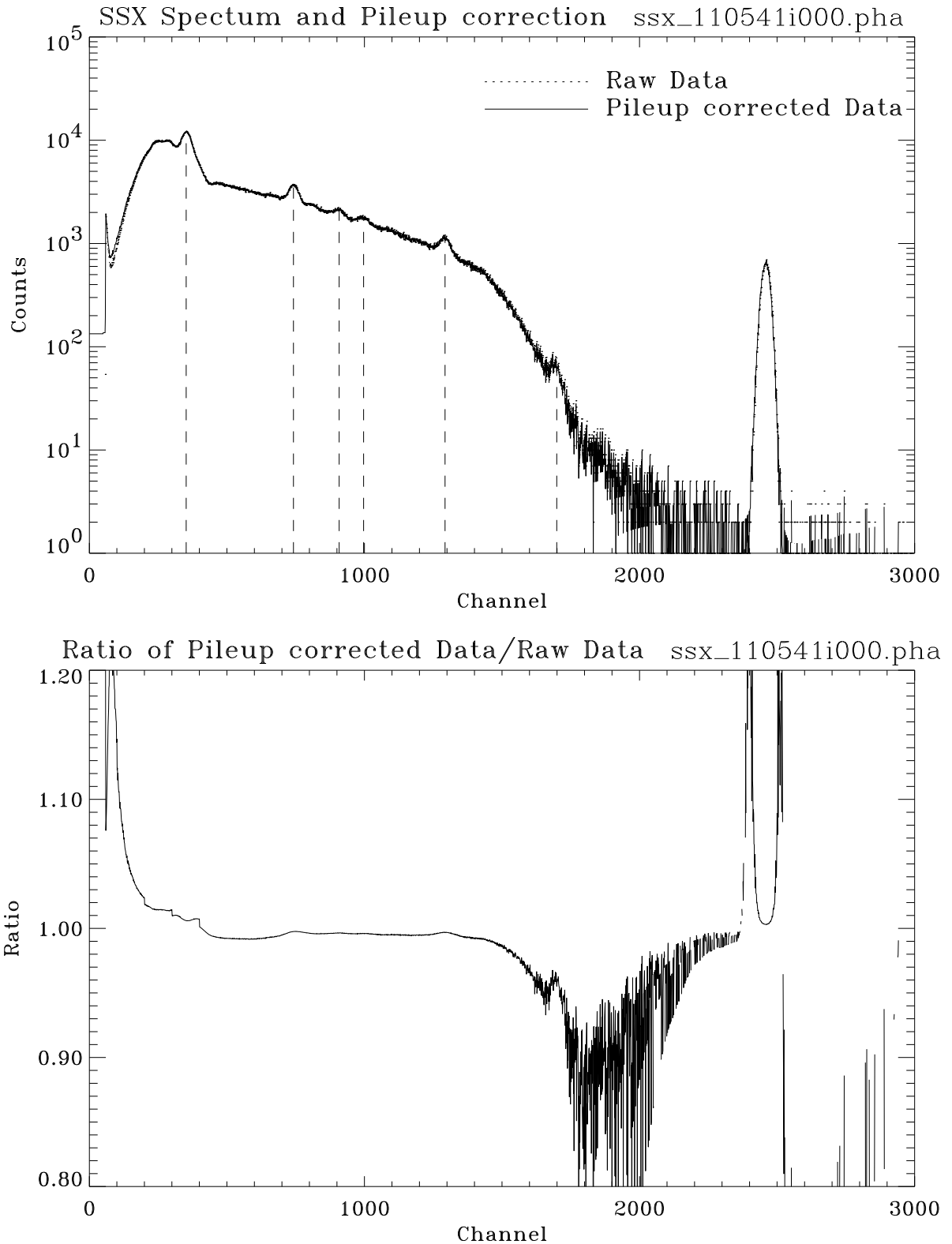
Figure 11.11: SSX spectrum and pileup correction: Shell 4; Run ID: 110541. Upper panel shows the raw data and pileup corrected data. Dashed vertical lines indicate the X-ray lines to be used to calibrate the energy scale. Lower panel shows the ratio of pileup corrected data to the raw data.
