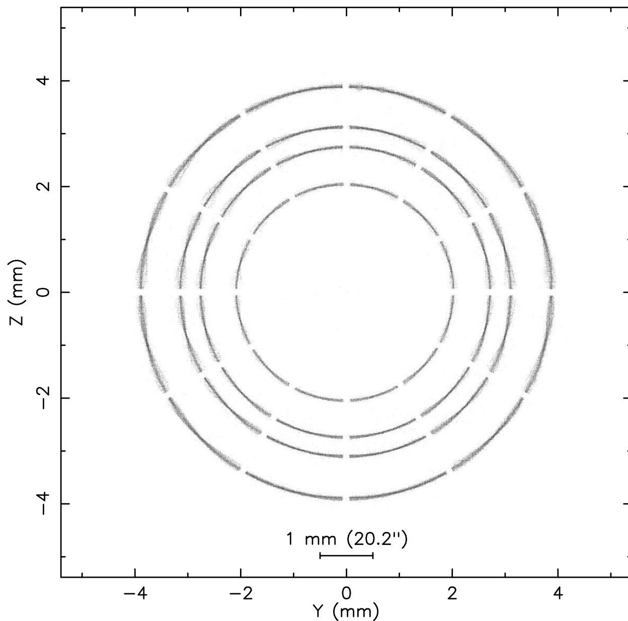
Figure 18.19: The HRMA ring focus model with -0.5% epoxy strain. Source: Al-K; Defocus: 65.2 mm
