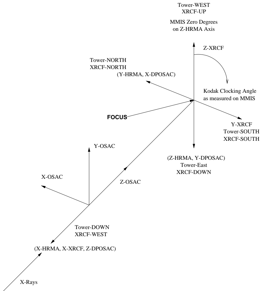
Figure B.1: Relations between HATS tower, XRCF, and SA0sac coordinates
