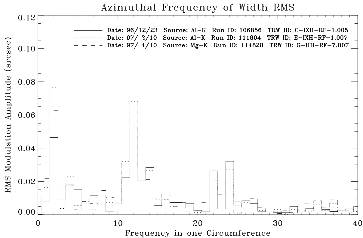
Figure 18.25: The Ring width RMS for ring 4, from three ring focus measurements on 1996/12/23, 1997/02/10 and 1997/04/10.
