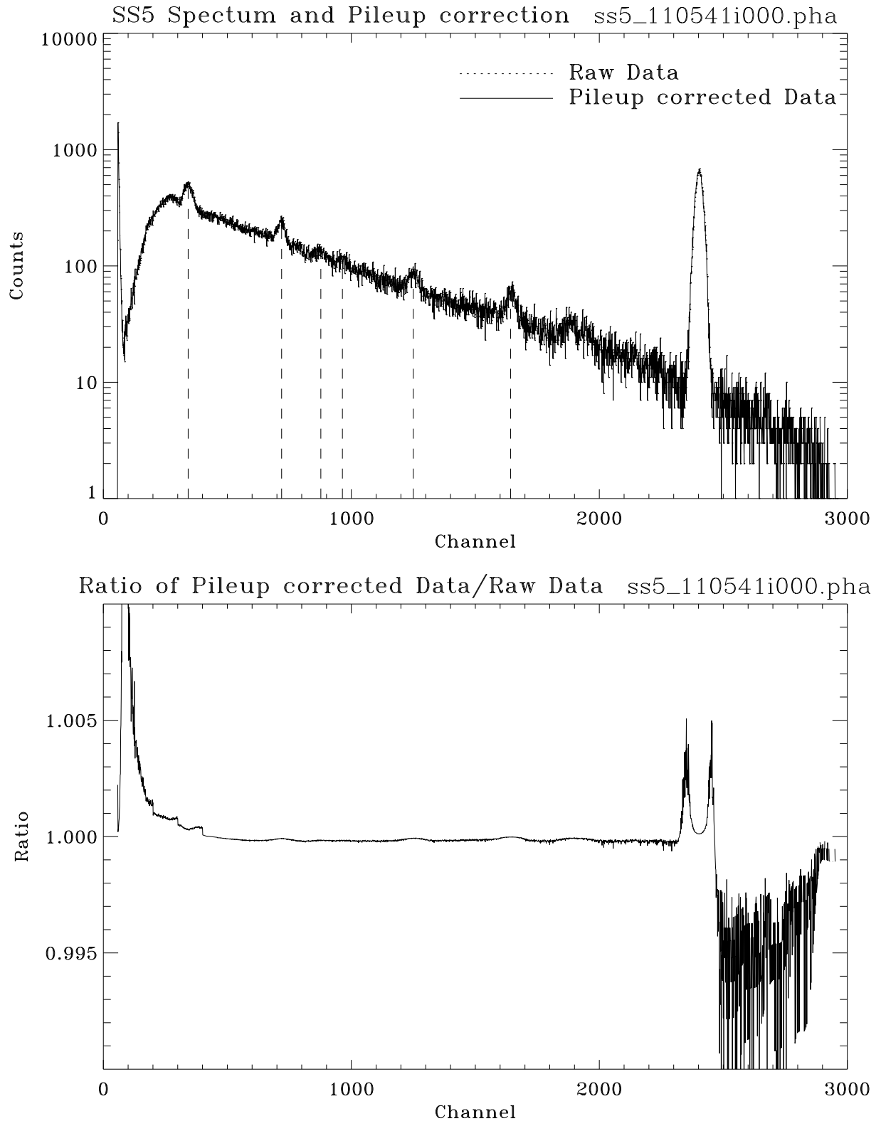
Figure 11.15: SS5 spectrum and pileup correction: Shell 4; Run ID: 110541. Upper panel shows the raw data and pileup corrected data. Dashed vertical lines indicate the X-ray lines to be used to calibrate the energy scale. Lower panel shows the ratio of pileup corrected data to the raw data.
