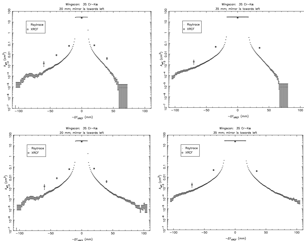
Figure 14.2: Effect of quadrant shutter vignetting. The top panels were raytraced for shell 3 alone and with quadrant configuration cccc-ccco-cccc-cccc while the bottom panels were traced with shell 3 alone but with all the South shutters open (quadrant shutter configuration ccco-ccco-ccco-ccco ).
