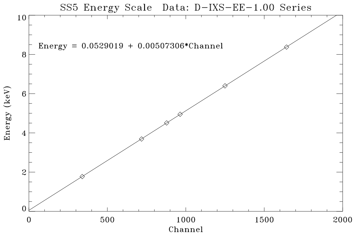
Figure 11.23: SSX and SS5 energy scales for the C-continuum effective area measurements (Phase-D), fitted with six X-ray line energies, averaged over four spectra (Run IDs: 108426, 108450, 108484, 108500).
