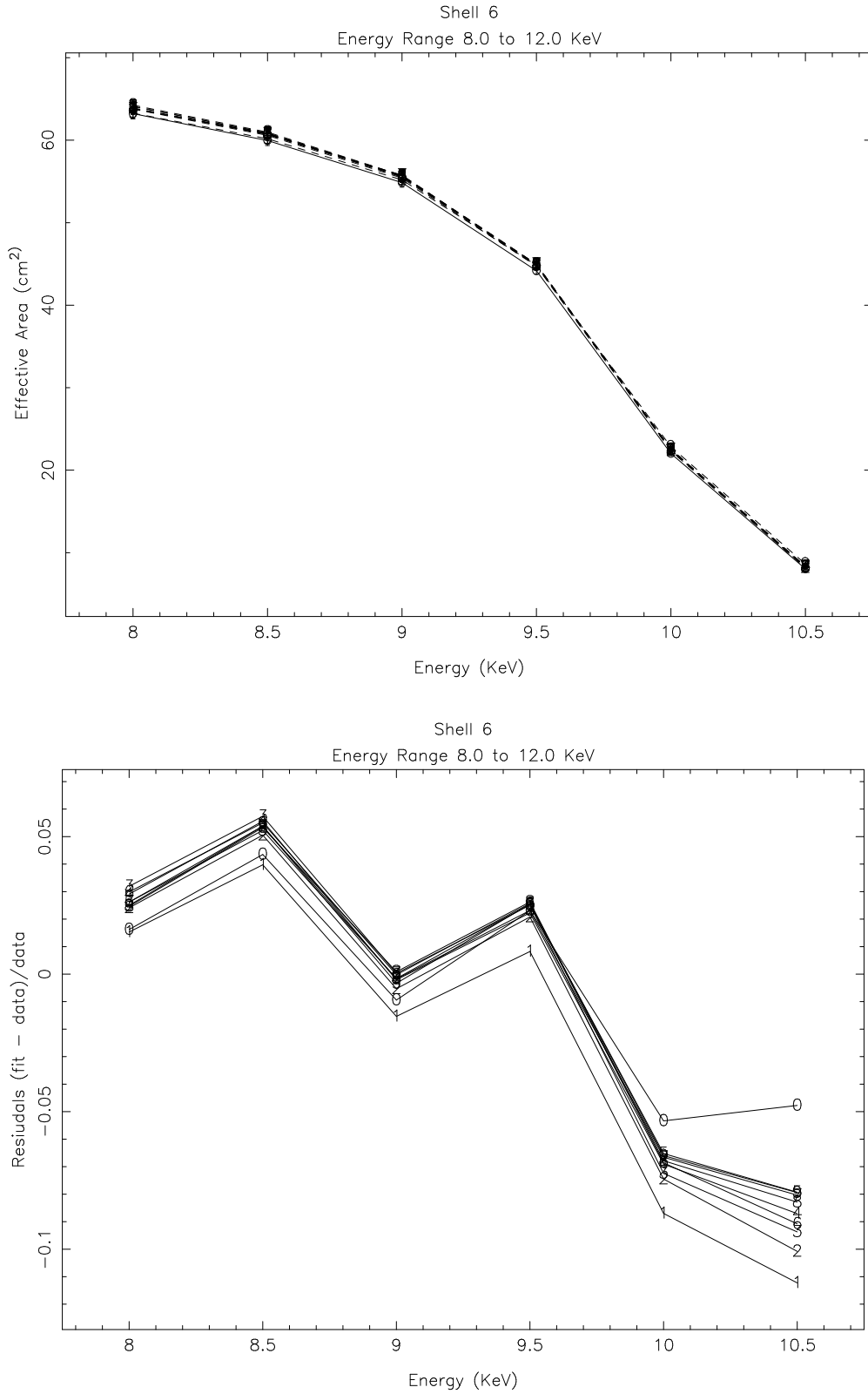
Figure 13.29: SSD continuum data and model effective area and residuals through 2mm pinhole for shell 6 between 8.0 and 12.0 keV.
