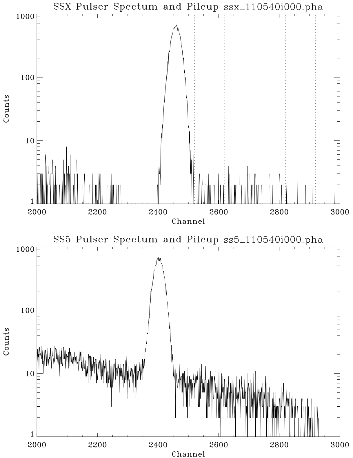
Figure 11.6: SSX and SS5 pulser spectra: Shell 3; Run ID: 110540. Counts to the right of the SSX pulser peak are the pileups from the pulser and low energy photons. Dotted vertical lines in the upper panel indicate the pulser region and four pileup bands.
