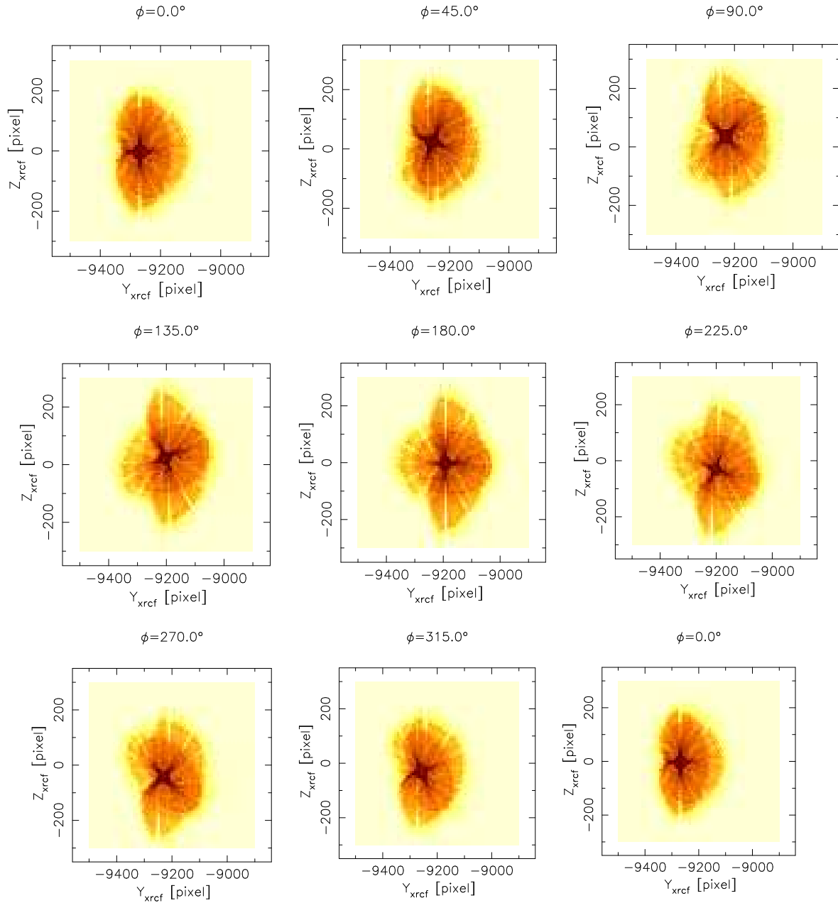
Figure 30.4: Variation of off-axis image with angle between source and decenter direction. Shell 3, pitch = 16.42' , yaw = 17.68' . Pixel width 6.43 \mu\text{m} ; binned to 8 \times 8 pixels. (Raytrace data; logarithmic stretch)
