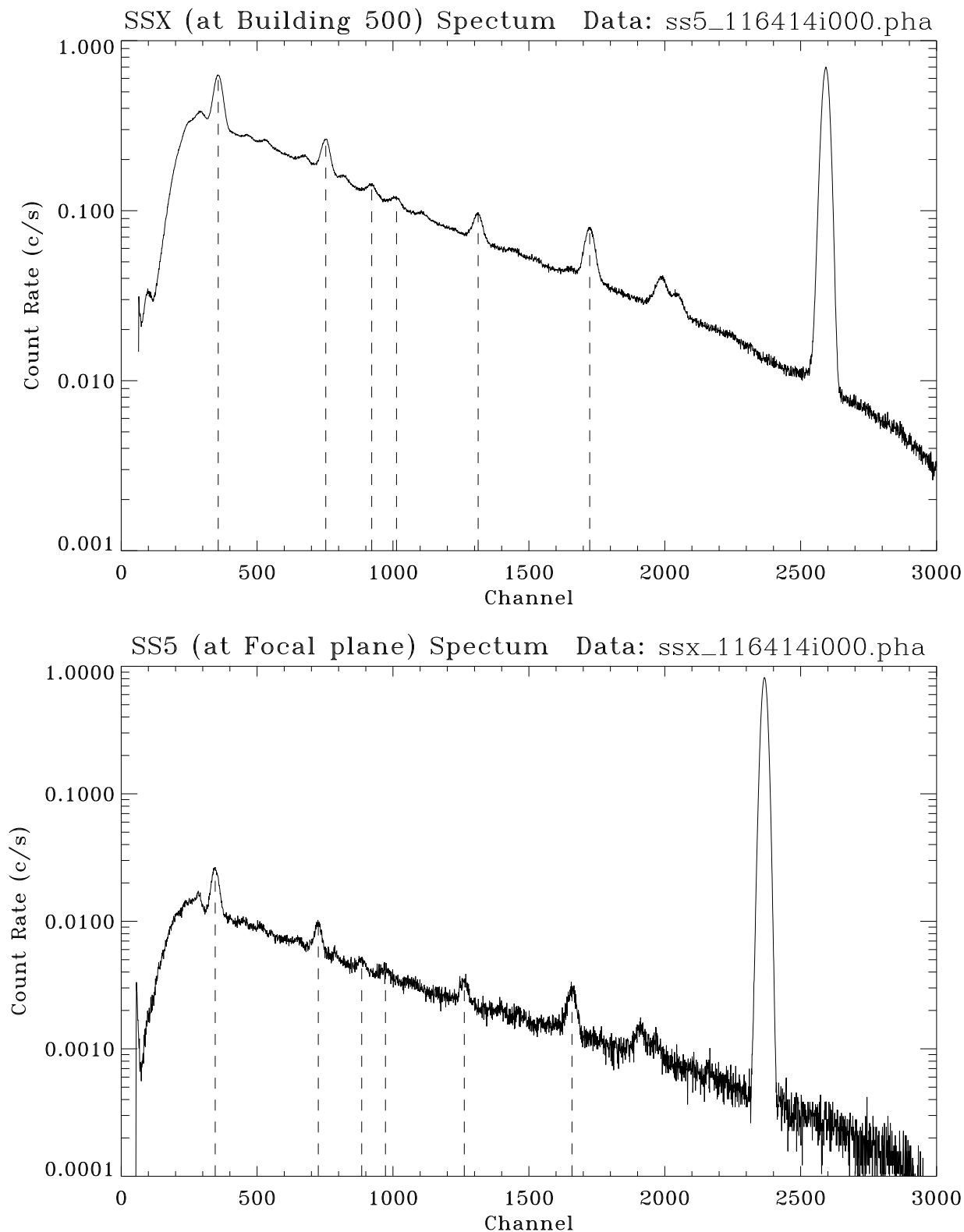
Figure 11.17: C-continuum flat field test SSX and SS5 spectra: Date: 970625; TRW ID: J-BND-BU-2.137; Run ID: 116414; Integration time: 57600 seconds. Dashed vertical lines indicate fitted centers of X-ray characteristic lines atop of the C-continuum spectrum.
