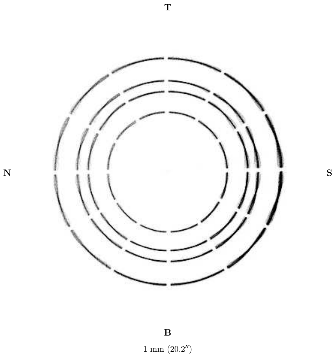
Figure 18.4: The HRMA ring focus HSI image. Date: 1997/01/24; TRW ID: D-IXH-RF-1.005; Run ID: 110004; Source: Al-K; Defocus: 65.2 mm; Integration time: 1800 seconds.
