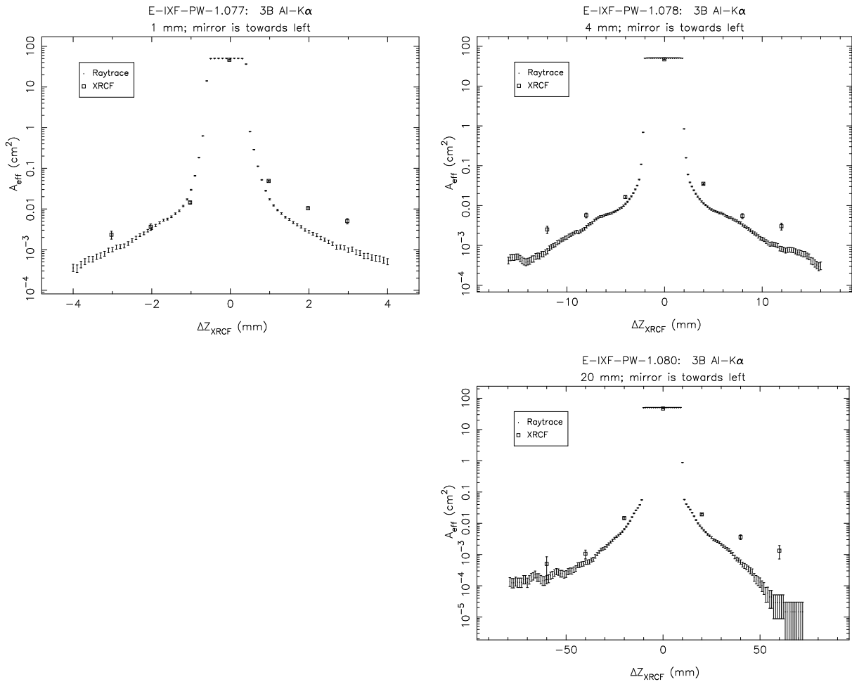
Figure 14.14: Pinhole effective areas; Shell 3B at Al-K \alpha .
