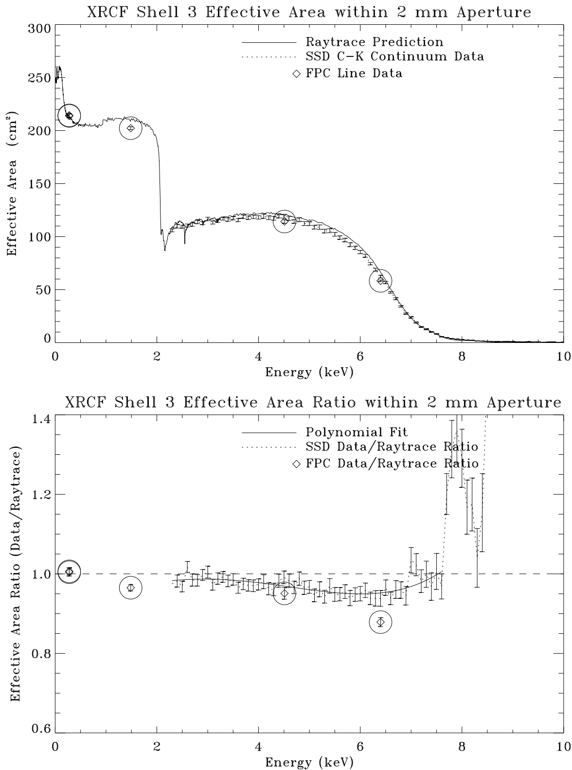
Figure 11.37: Calibration data vs. raytrace prediction. Top panel shows the XRCF Shell 3 effective area within 2 mm aperture. Bottom panel shows the effective area ratio of data/raytrace.
