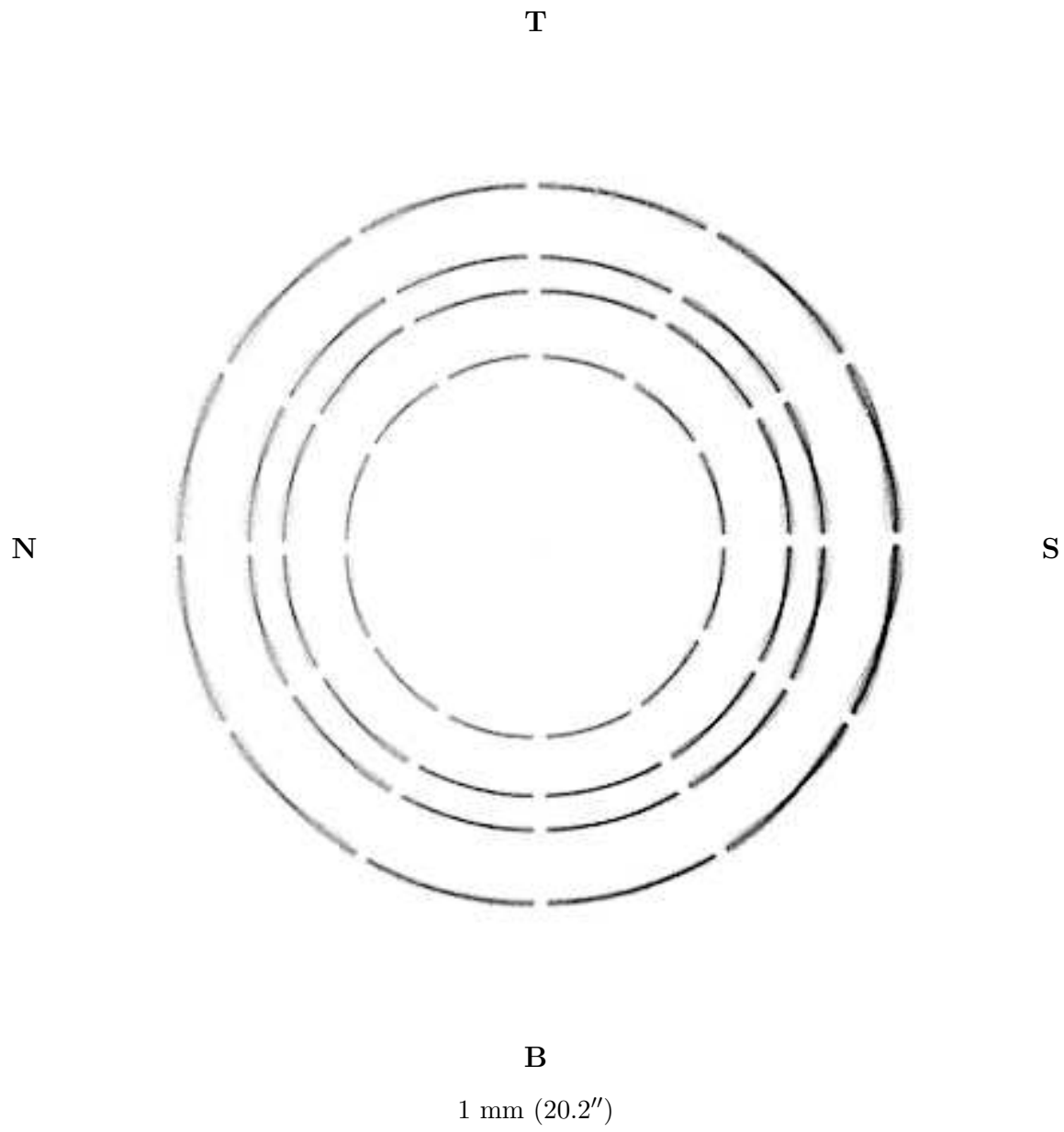
Figure 18.5: The HRMA ring focus HSI image. Date: 1997/02/10; TRW ID: E-IXH-RF-1.007; Run ID: 111804; Source: A1-K; Defocus: 65.2 mm; Integration time: 1800 seconds.
