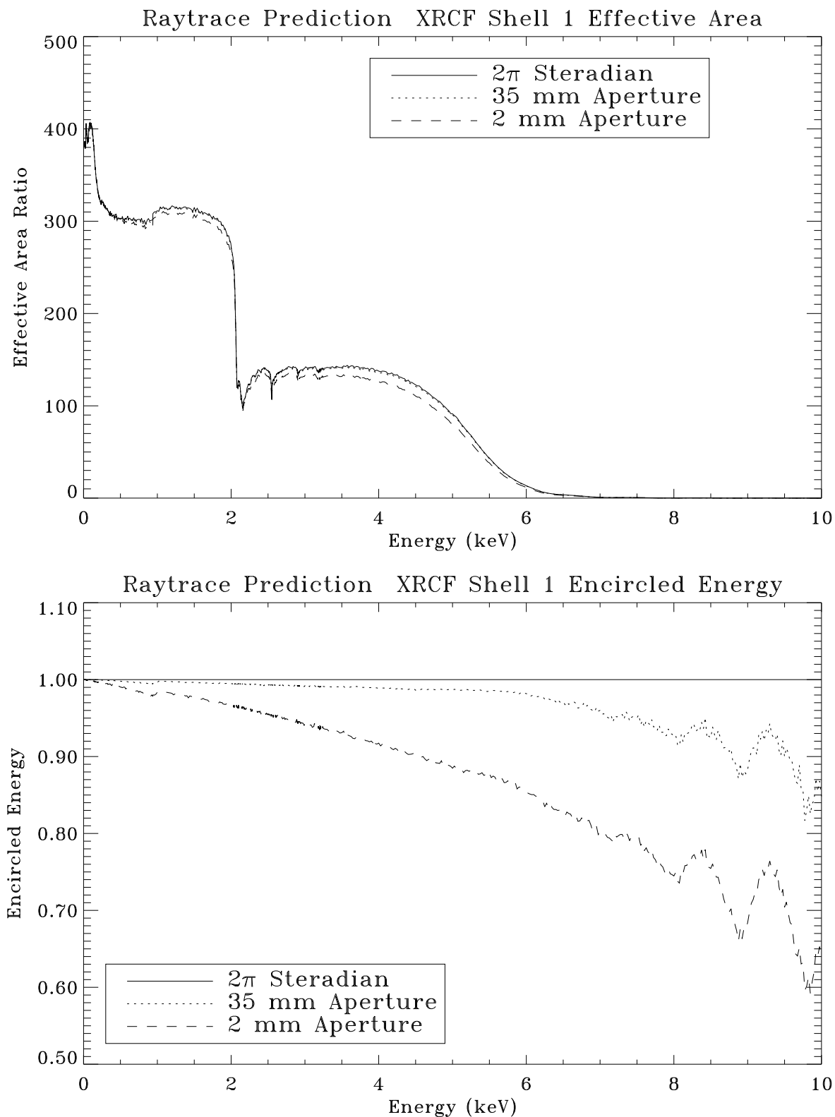
Figure 11.41: Raytrace prediction of XRCF Shell 1 effective area and encircled energy. Top panel shows the effective area curves within 2 mm, 35 mm apertures, and 2\pi steradian. Bottom panel shows the encircled energies of 2 mm and 35 mm apertures as fractions of that within 2\pi steradian.
