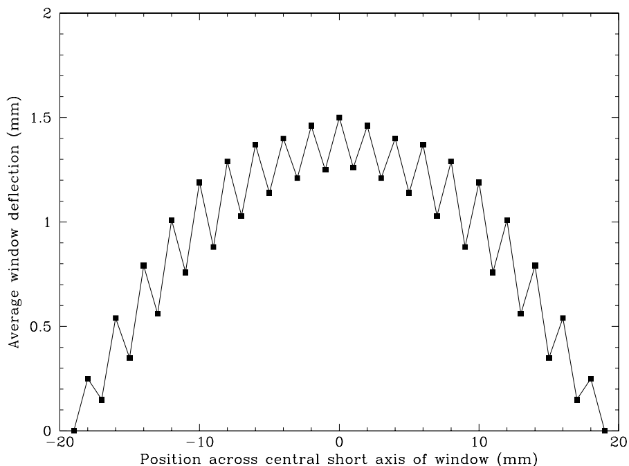
Figure 3.15: Measured deflection of the polyimide/Al window material across the central short axis. The average is shown from three windows, all measured at the standard operating pressure of 400 torr. Deflections were measured in the center of each windowlet and underneath the support wires. Variation between the two most different windows was typically 0.30 mm.
