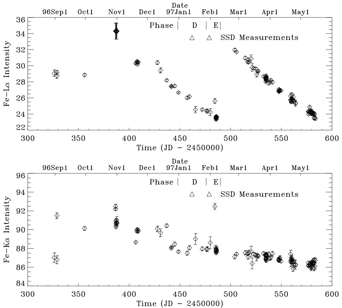
Figure 11.29: SSD 500 icing data (courtesy: Allyn Tennant). In order to monitor the ice build up, a radioactive isotope ^{244}_{96}\text{Cm} excited Fe source was placed on the aperture wheel and rotated to front of the SS5 from time to time. The Figure shows the Fe-L \alpha (0.705 keV) and Fe-K \alpha (6.40 keV) line intensity with error bars measured with SS5 as a function of time from 960824 to 970521 (JD 2450320 – 2450590). Upper portions of each panel show the Phase D and E of the HRMA calibration and the dates of the SSD C-continuum measurements. In the top panel, the Fe-L \alpha intensity has two peaks, on 961031 and 970223, followed by declines. These two peaks indicate the time when the SS5 was warmed up and assuming there was no ice then. The declines indicate the ice build up and therefore reducing the transmission of Fe-L \alpha into the SS5. In the bottom panel, the fluctuations of Fe-K \alpha intensity could be due to icing, source aging and other temporal variations. To obtain the icing information, we only need to focus on the intensity ratio of Fe-L \alpha /Fe-K \alpha . At the end of each ice build up period, the Fe-L \alpha /Fe-K \alpha transmission ratio is 74% of its value at the beginning. This result is used to obtain the ice thickness.
