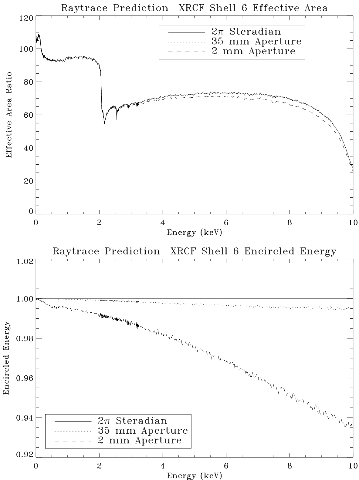
Figure 11.44: Raytrace prediction of XRCF Shell 6 effective area and encircled energy. Top panel shows the effective area curves within 2 mm, 35 mm apertures, and 2\pi steradian. Bottom panel shows the encircled energies of 2 mm and 35 mm apertures as fractions of that within 2\pi steradian.
