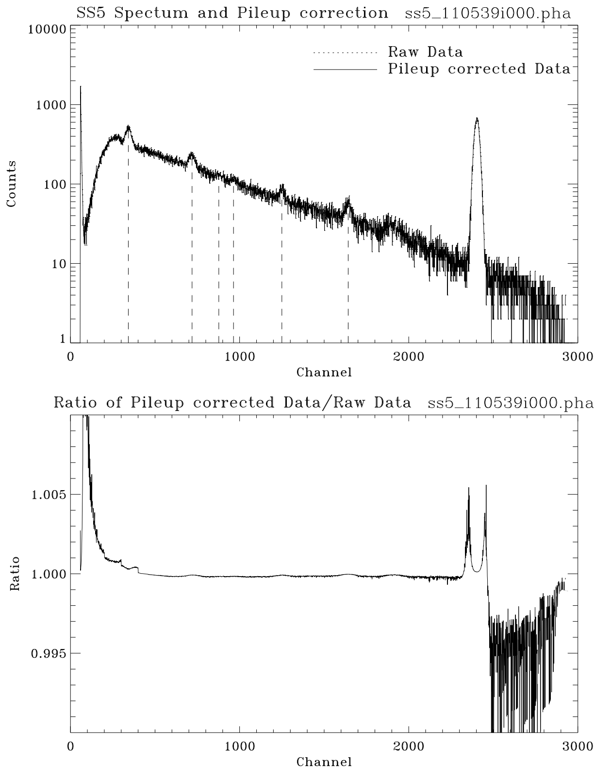
Figure 11.13: SS5 spectrum and pileup correction: Shell 1; Run ID: 110539. Upper panel shows the raw data and pileup corrected data. Dashed vertical lines indicate the X-ray lines to be used to calibrate the energy scale. Lower panel shows the ratio of pileup corrected data to the raw data.
