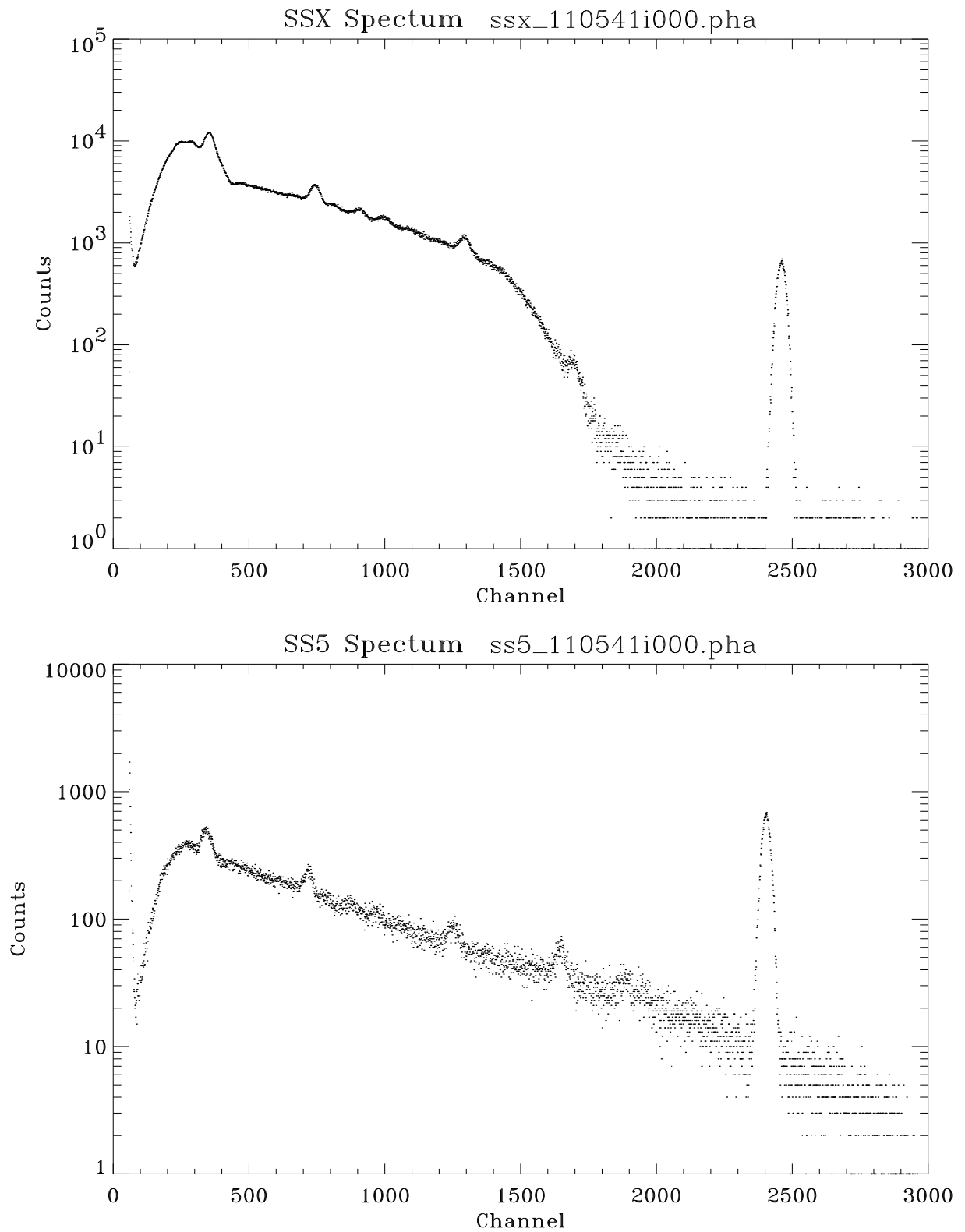
Figure 11.3: C-continuum SSX and SS5 spectra: Shell 4; Date: 970130; TRW ID: E-IXS-MC-15.003; Run ID: 110541; Aperture: 2 mm; Integration time: 1000 seconds.
