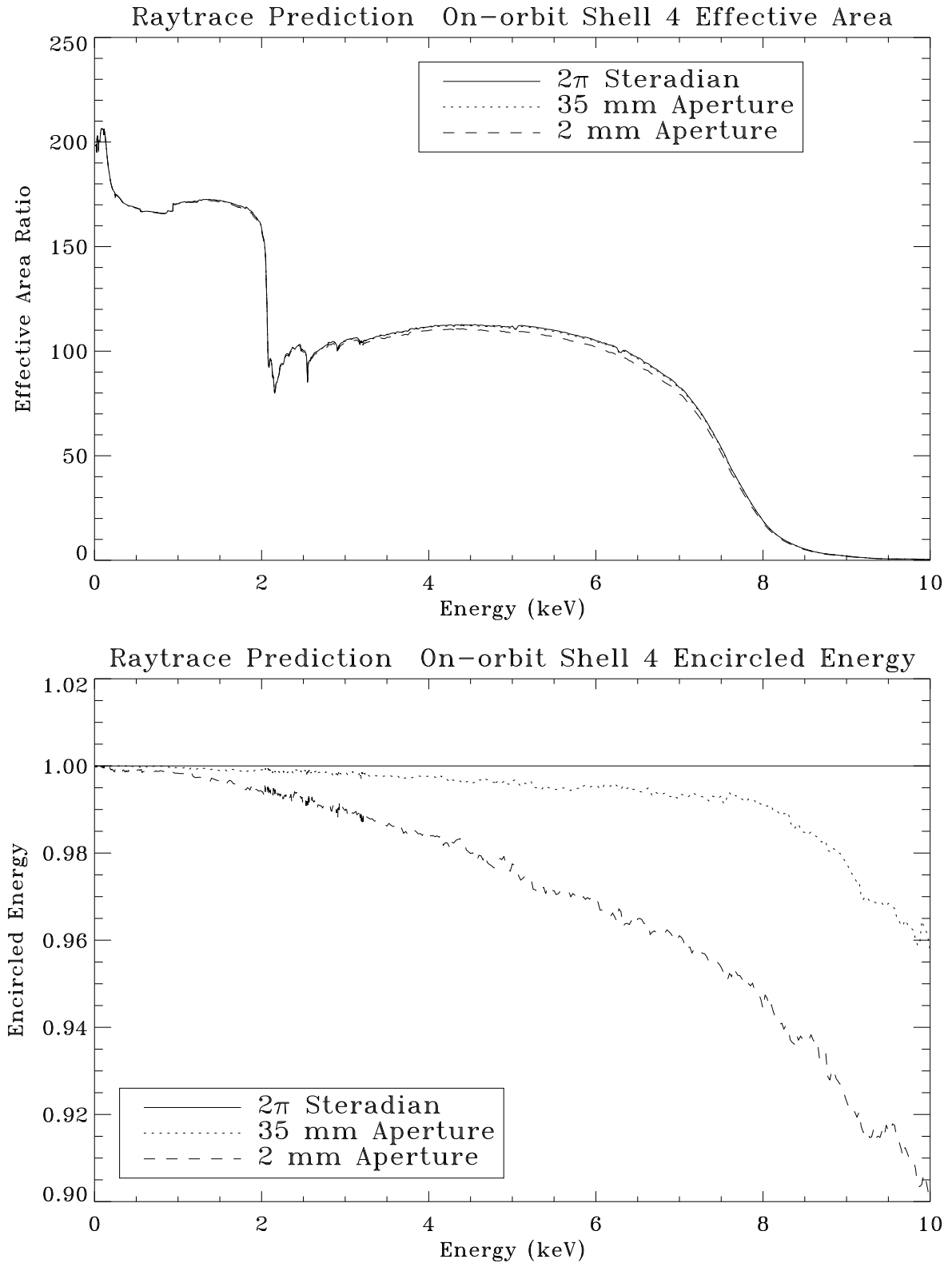
Figure 11.48: Raytrace prediction of on-orbit Shell 4 effective area and encircled energy. Top panel shows the effective area curves within 2 mm, 35 mm apertures, and 2\pi steradian. Bottom panel shows the encircled energies of 2 mm and 35 mm apertures as fractions of that within 2\pi steradian.
