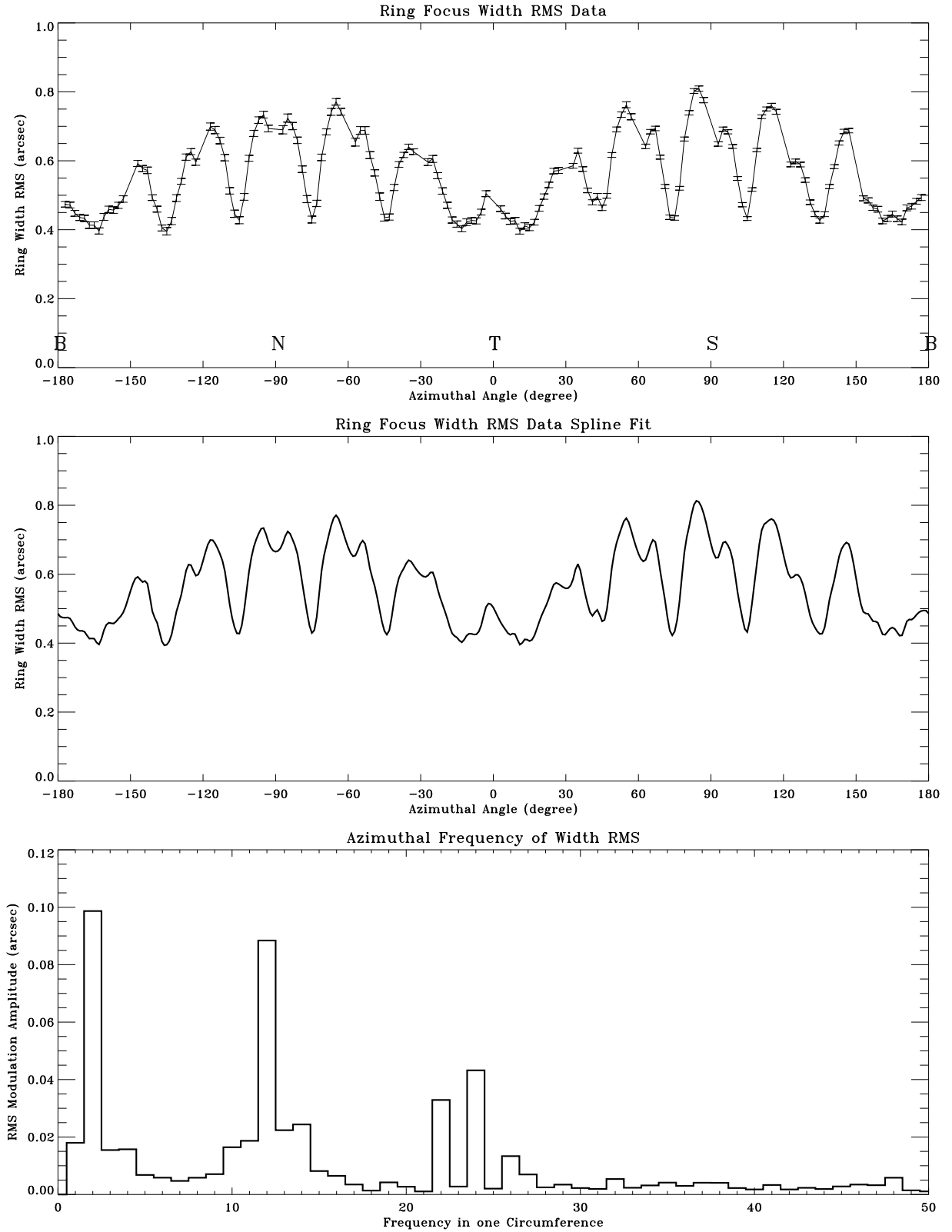
Figure 18.12: The Ring width RMS for ring 3. Date: 1997/01/24; TRW ID: D-IXH-RF-1.005; Run ID: 110004; Source: Al-K; Defocus: 65.2 mm.
