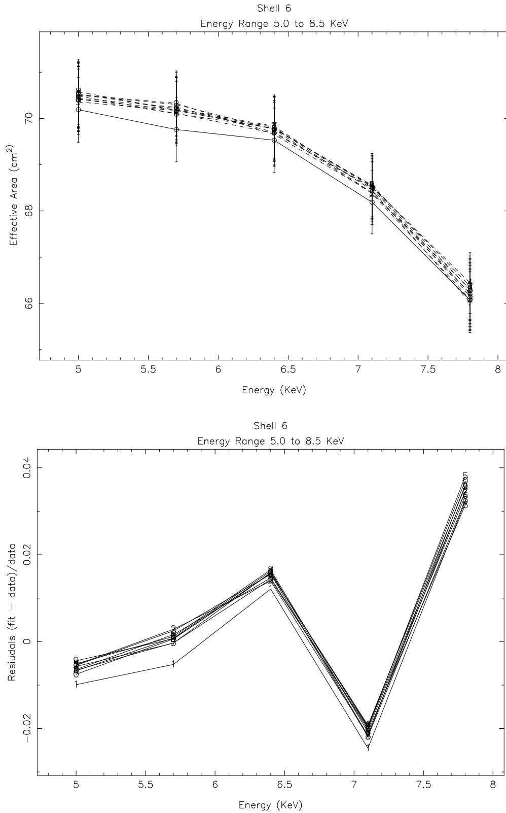
Figure 13.28: SSD continuum data and model effective area and residuals through 2mm pinhole for shell 6 between 5.0 and 8.5 keV.
