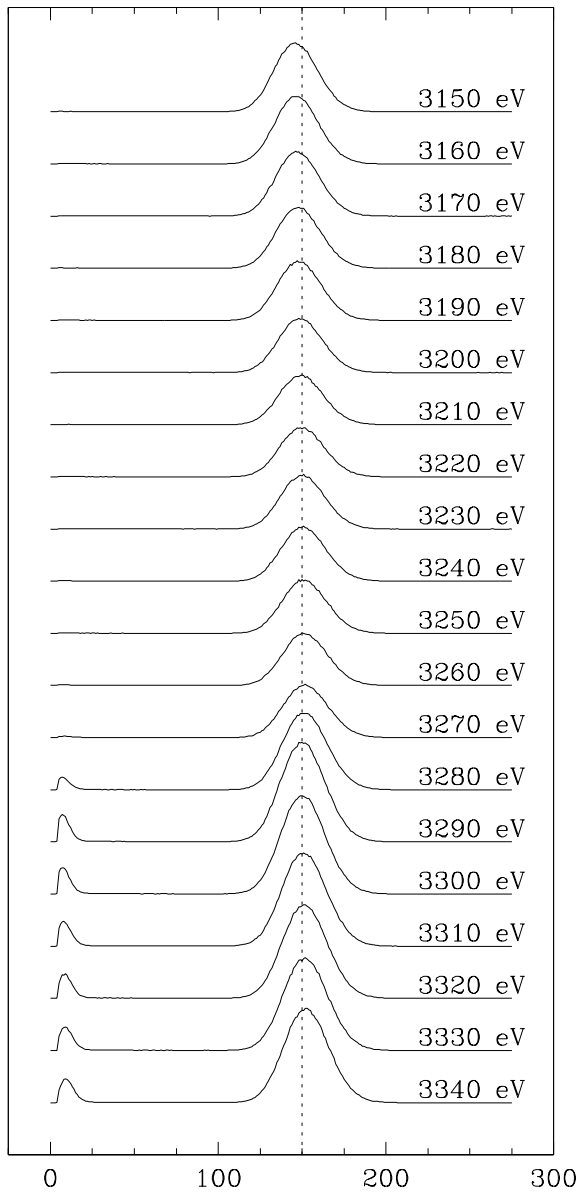
Figure 3.3: Ar-K edge scan with BESSY KMC monochromator. These data were used to measure the FPC gas opacity just below the edge. Listed energies are those requested; the true edge energy (indicated by the appearance of an escape peak and a jump in the strength of the main peak) is 3206 eV, thus calibrating the monochromator energy scale as approximately 75 eV too high. The dotted vertical line is merely to help discern relative peak positions.
