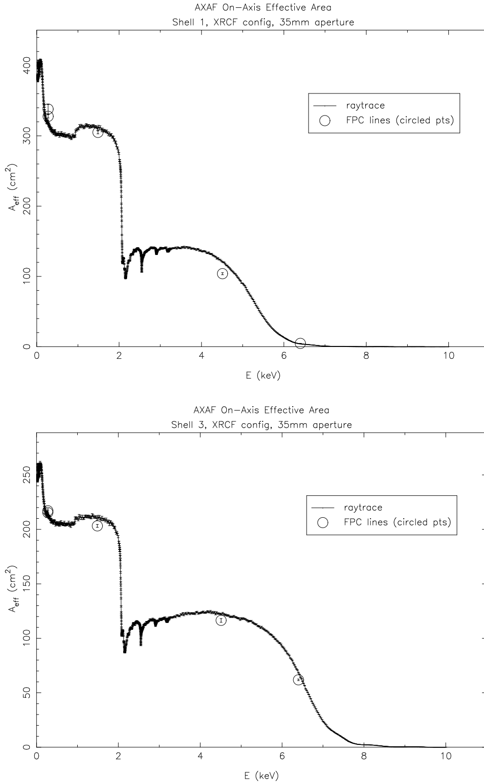
Figure 12.1: Measurements and Ray traces for effective area through 35 mm pinholes for shells 1 and 3.
