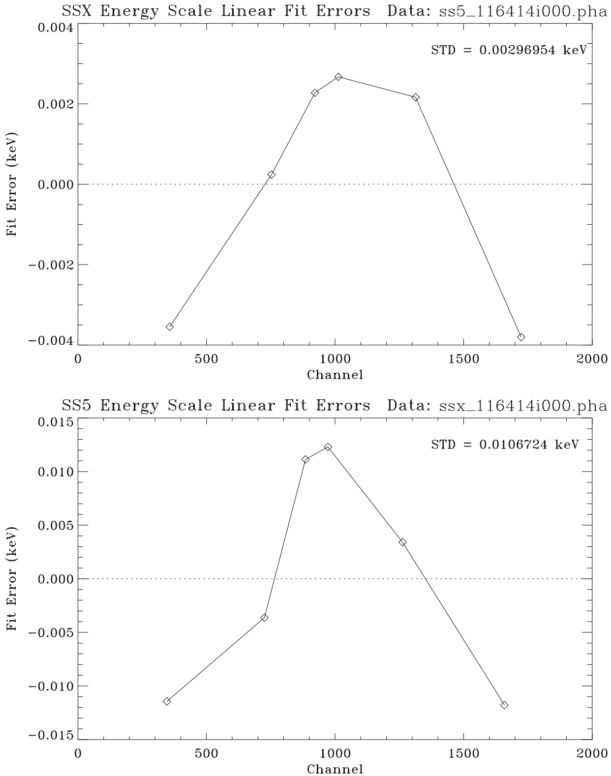
Figure 11.19: SSX and SS5 energy scale linear fit residuals for the flat field test (Phase-J).
