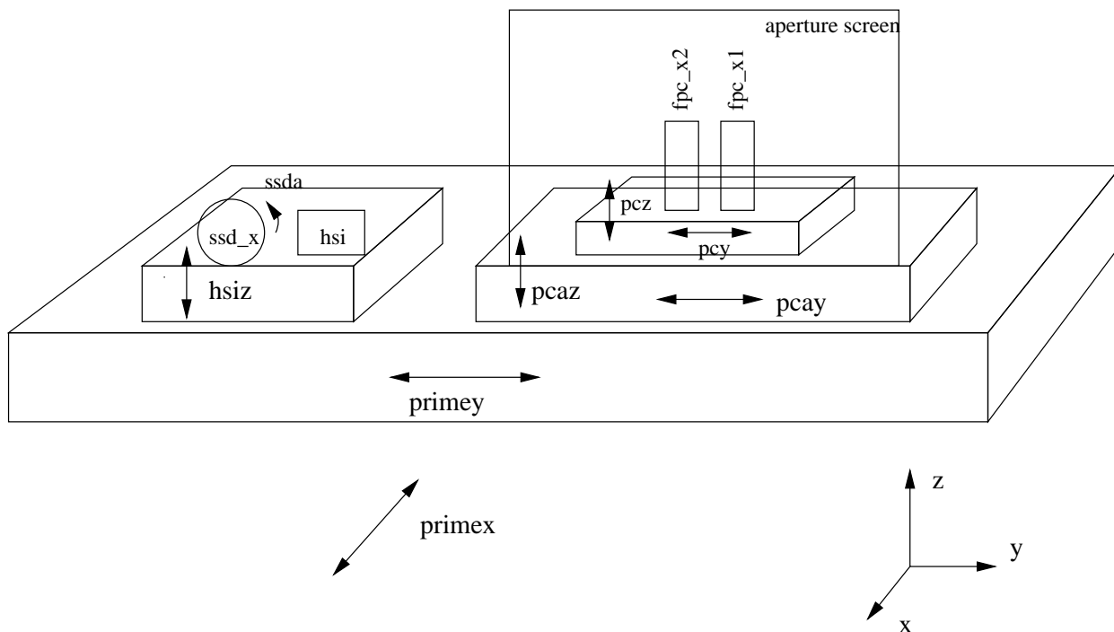
Figure 8.1: A diagram of the focal plane HXDA translation stages and detectors. Coordinates are XRCF coordinates; the HRMA is in the +x direction from the detectors. Top refers to the +z direction, and South to the +y direction.
