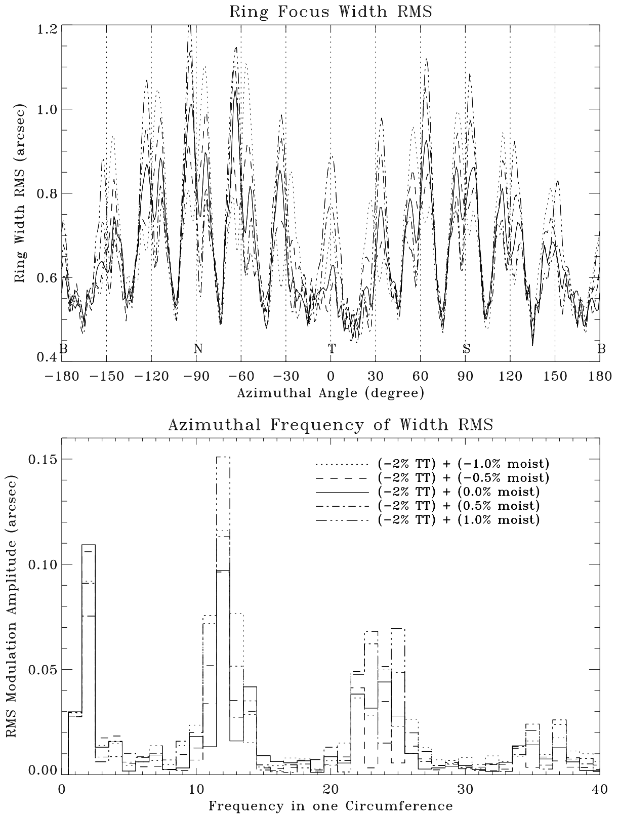
Figure 18.22: HRMA ring focus model: Ring 1, Al-K source, with gravity and epoxy strain change.
