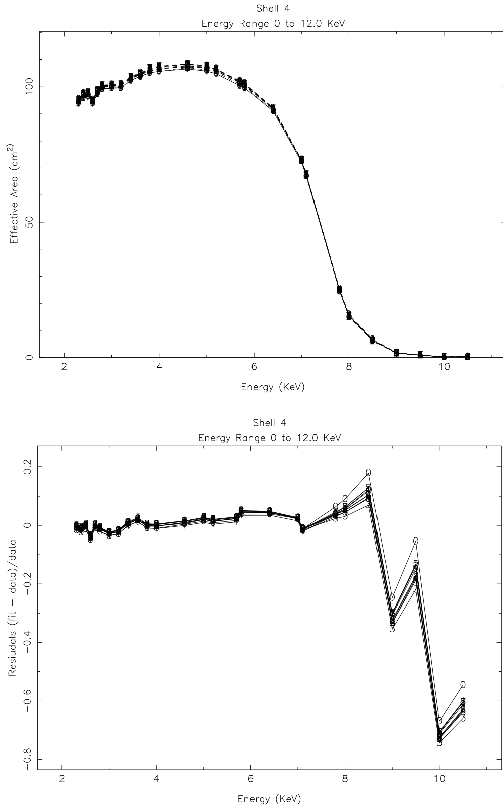
Figure 13.4: SSD continuum data and model effective area and residuals through 2mm pinhole for shell 4.
