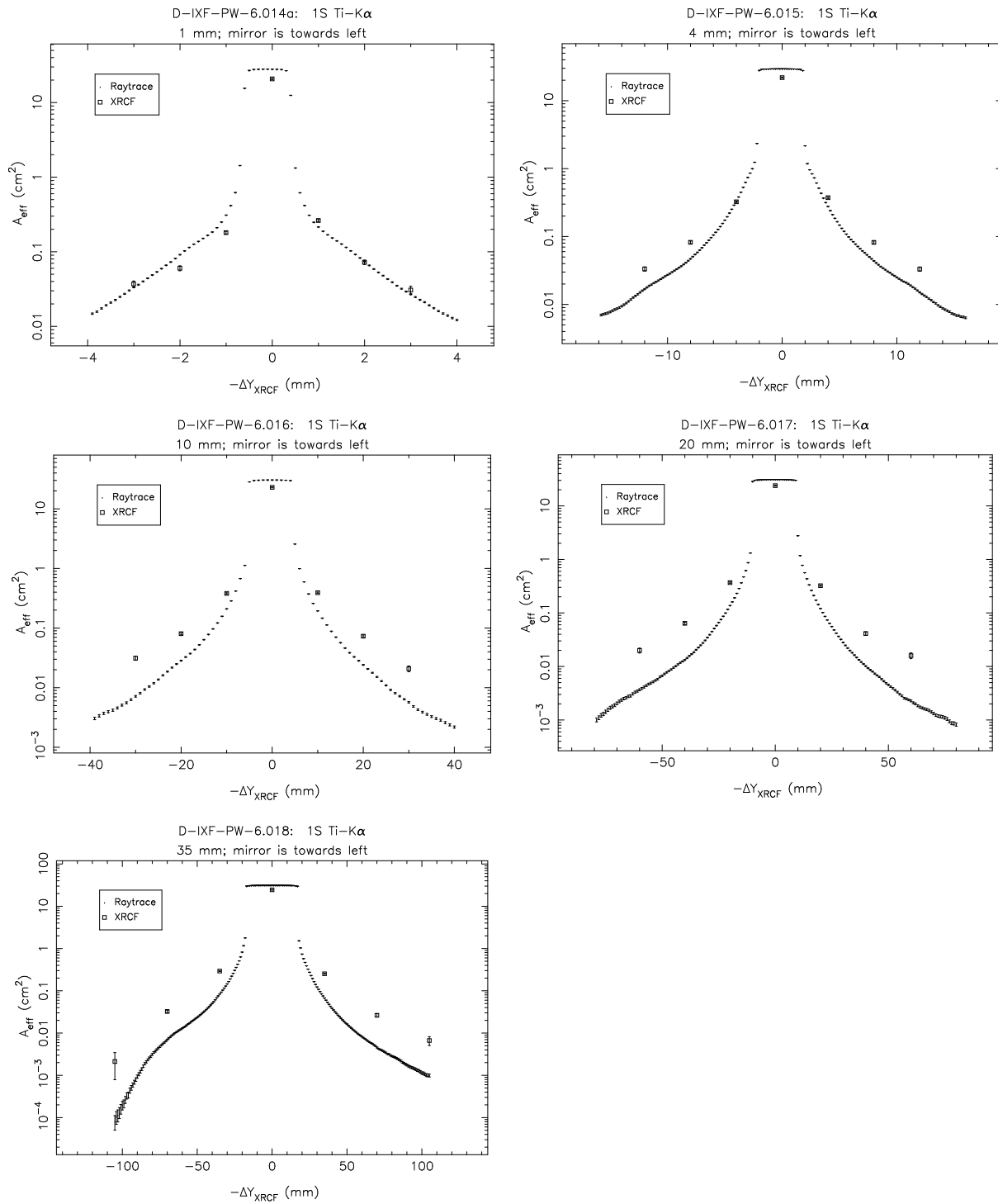
Figure 14.11: Pinhole effective areas; Shell 1S at \text{Ti-K}\alpha .
