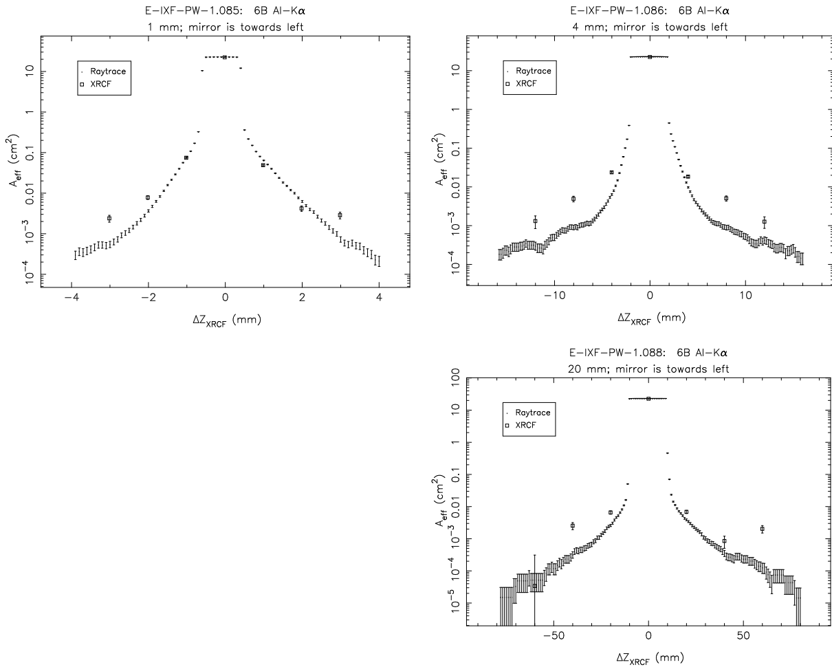
Figure 14.36: Pinhole effective areas; Shell 6B at Al-K \alpha .
