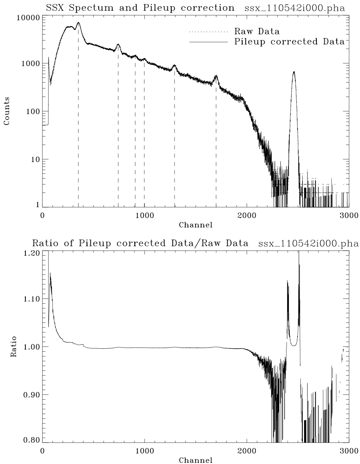
Figure 11.12: SSX spectrum and pileup correction: Shell 6; Run ID: 110542. Upper panel shows the raw data and pileup corrected data. Dashed vertical lines indicate the X-ray lines to be used to calibrate the energy scale. Lower panel shows the ratio of pileup corrected data to the raw data.
