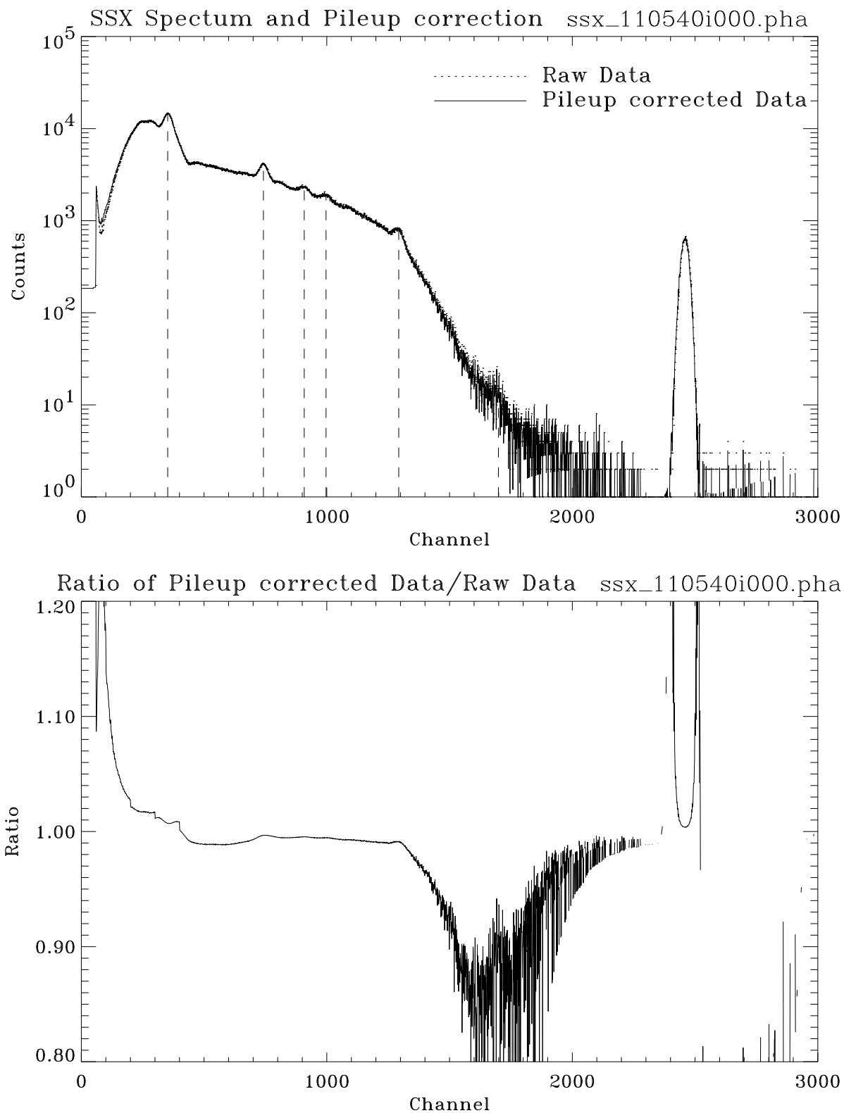
Figure 11.10: SSX spectrum and pileup correction: Shell 3; Run ID: 110540. Upper panel shows the raw data and pileup corrected data. Dashed vertical lines indicate the X-ray lines to be used to calibrate the energy scale. Lower panel shows the ratio of pileup corrected data to the raw data.
