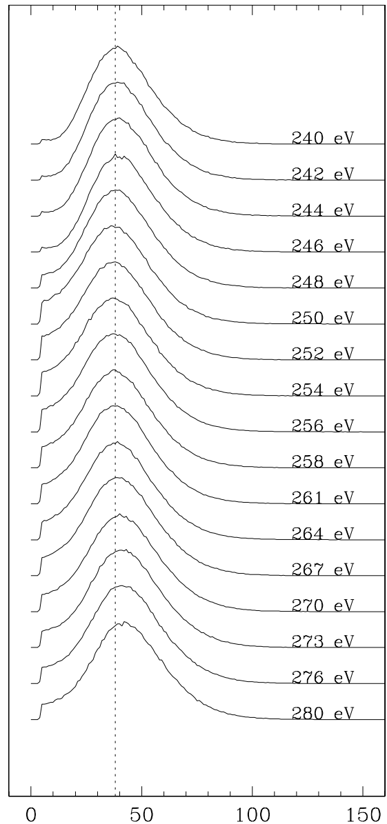
Figure 3.4: Ar-L edge scan with BESSY SX700 monochromator. Nominal L_{III} edge energy is 248.4 eV. Note that the main peak position does a little “back-step” as the beam energy crosses the edges (see the vertical dotted line for reference). This change in the average energy per effective secondary electron is plotted in Figure 3.6, and Figure 3.5 for the Ar-K edge. Charge diffusion losses may also be involved, particularly at the Ar-L edge.
