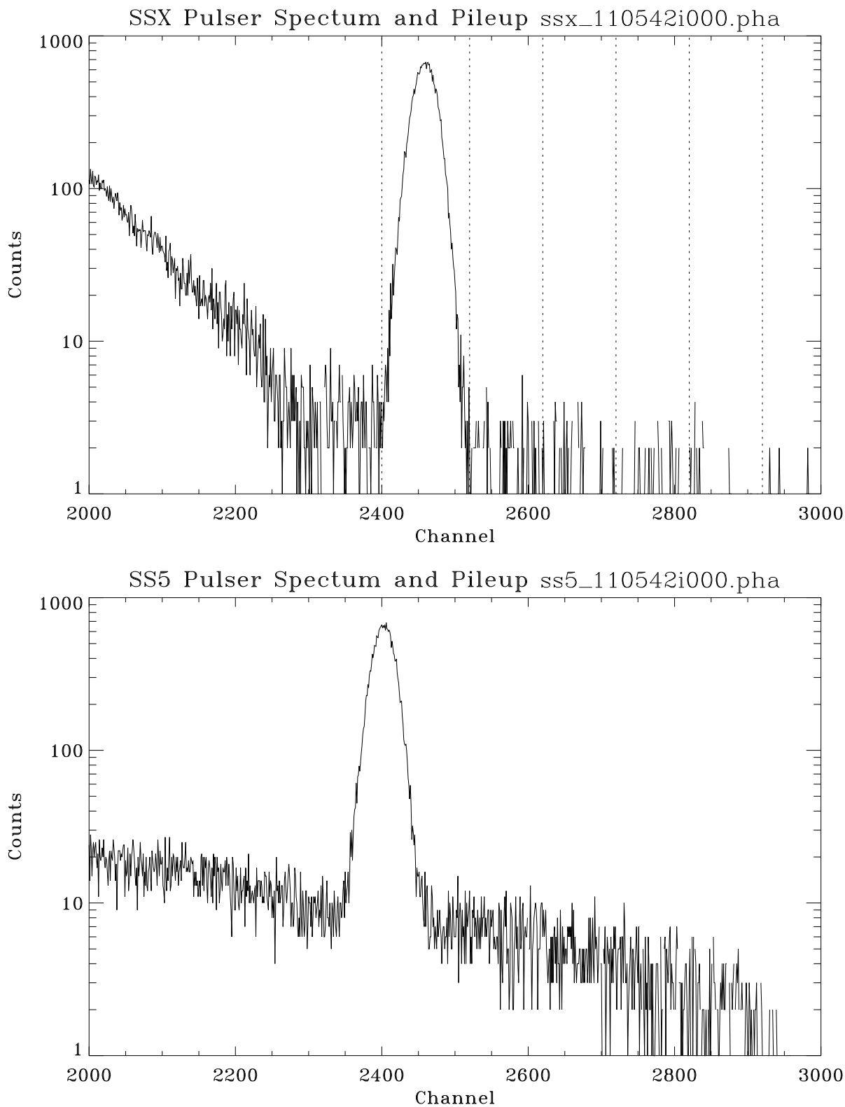
Figure 11.8: SSX and SS5 pulser spectra: Shell 6; Run ID: 110542. Counts to the right of the SSX pulser peak are mixtures of the pulser pileups and the continuum pileups.
