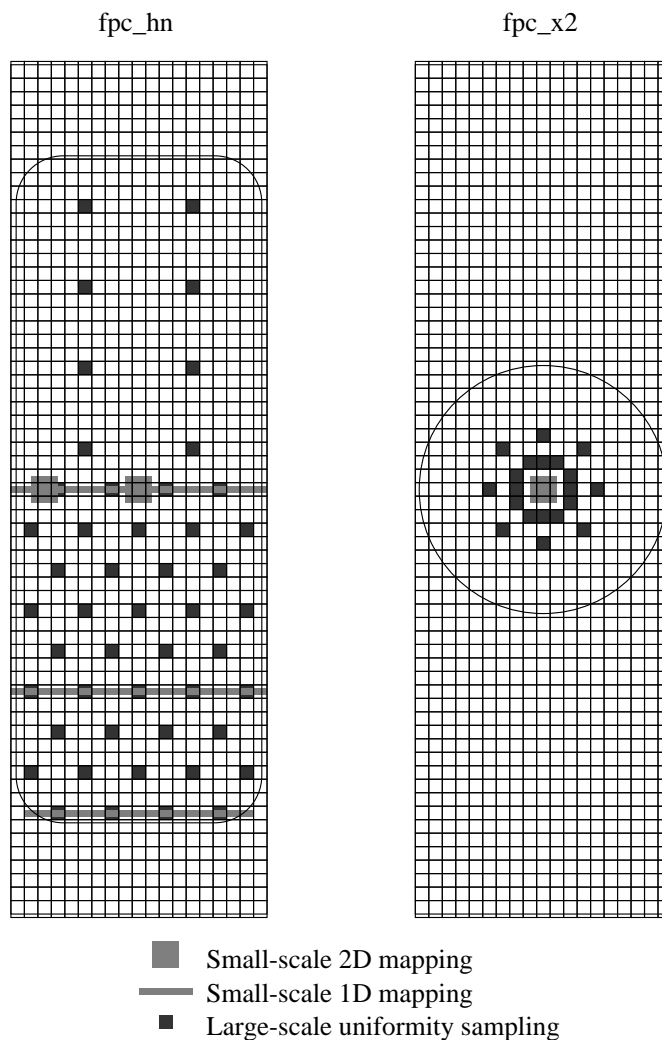
Figure 3.14: QE mapping of fpc_hn and fpc_x2 . Drawings show full window assembly (1.5" by 5.0" with 2-mm wire spacing), with blocking plate apertures for fpc_hn and fpc_x2 . Small-scale scans used five points per windowlet, in 350- \mu\text{m} steps. Most QE mapping was conducted at 330 eV; some scans were repeated at 500 and 930 eV. Mapping pattern for the two-dimensional small-scale scans is shown in Figure 3.16. SRF/absolute QE measurements were made in the center windowlets (or 2 mm to the side when using the higher-energy KMC beam, so that penetrating x-rays would not hit the anode wire running down the middle).
