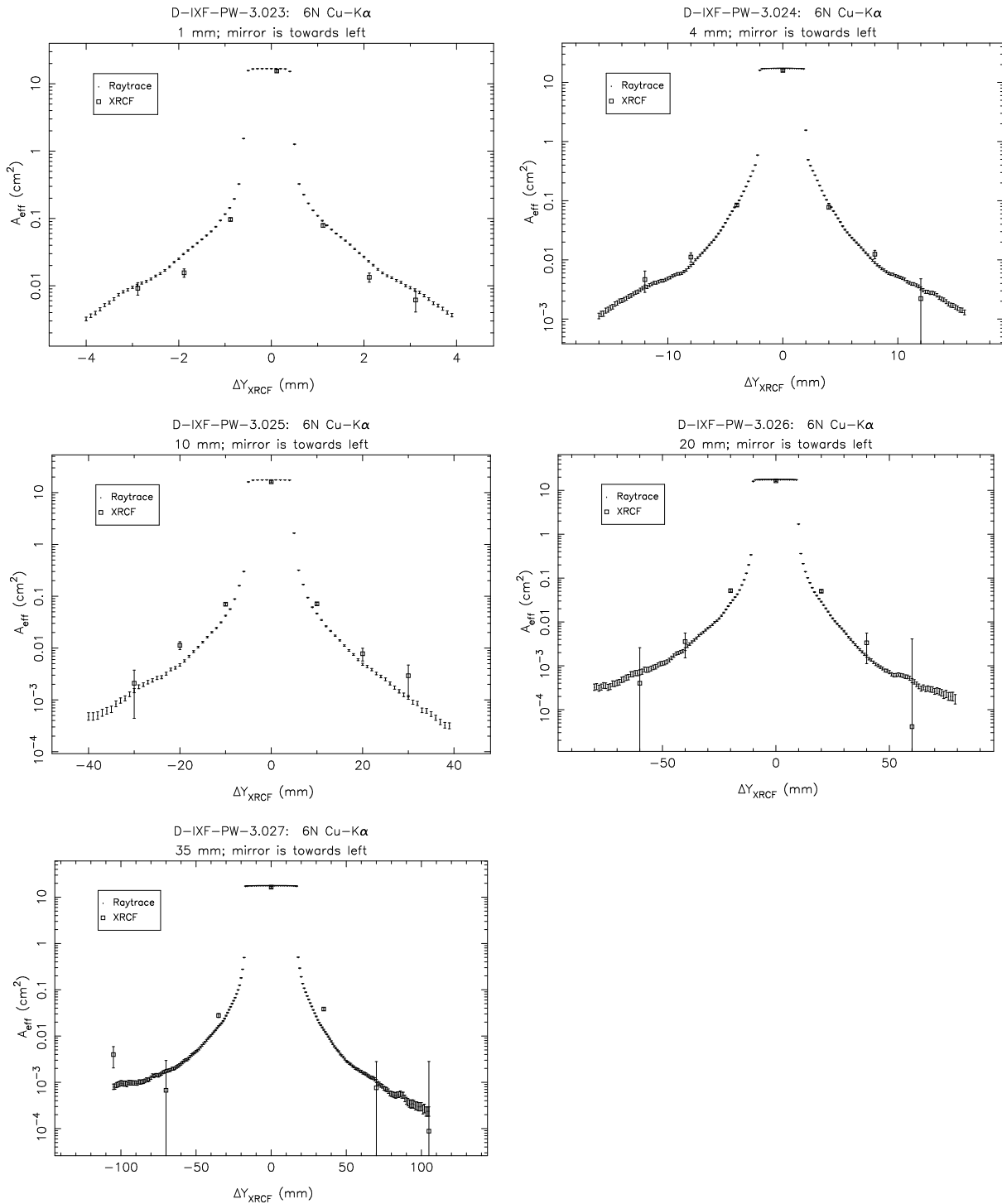
Figure 14.44: Pinhole effective areas; Shell 6N at Cu-K \alpha .
