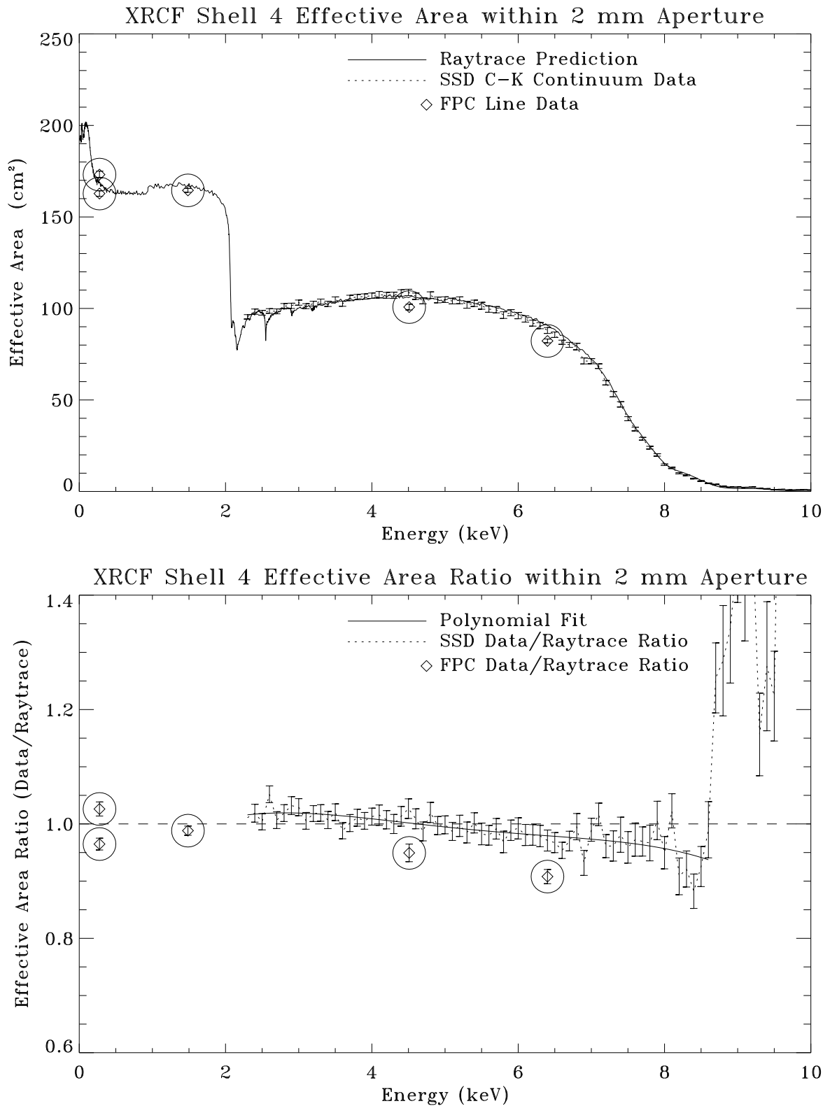
Figure 11.38: Calibration data vs. raytrace prediction. Top panel shows the XRCF Shell 4 effective area within 2 mm aperture. Bottom panel shows the effective area ratio of data/raytrace.
