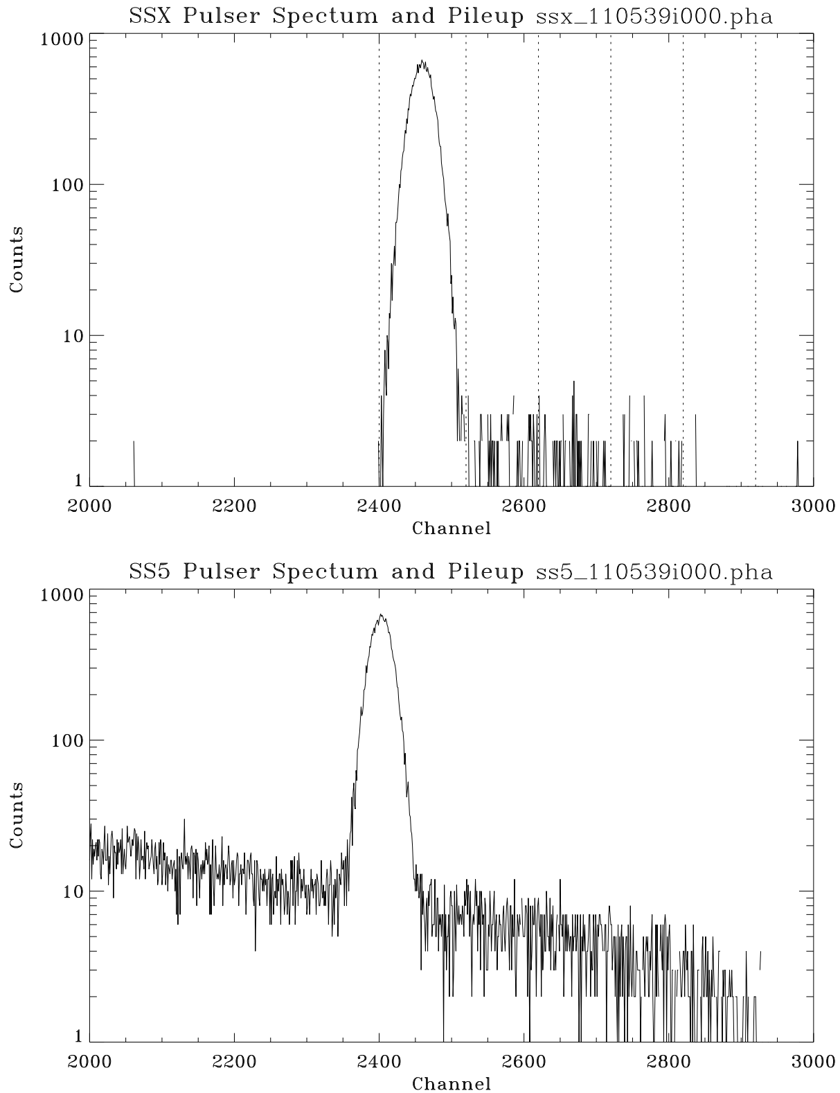
Figure 11.5: SSX and SS5 pulsar spectra: Shell 1; Run ID: 110539. Counts to the right of the SSX pulsar peak are the pileups from the pulsar and low energy photons. Dotted vertical lines in the upper panel indicate the pulsar region and four pileup bands.
