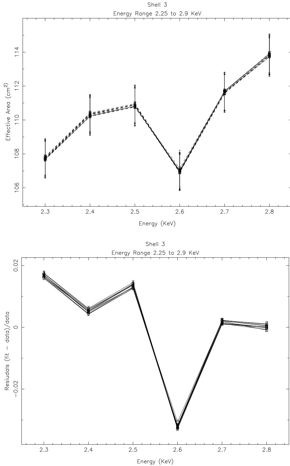
Figure 13.13: SSD continuum data and model effective area and residuals through 2mm pinhole for shell 3 between 2.25 and 2.9 keV.
