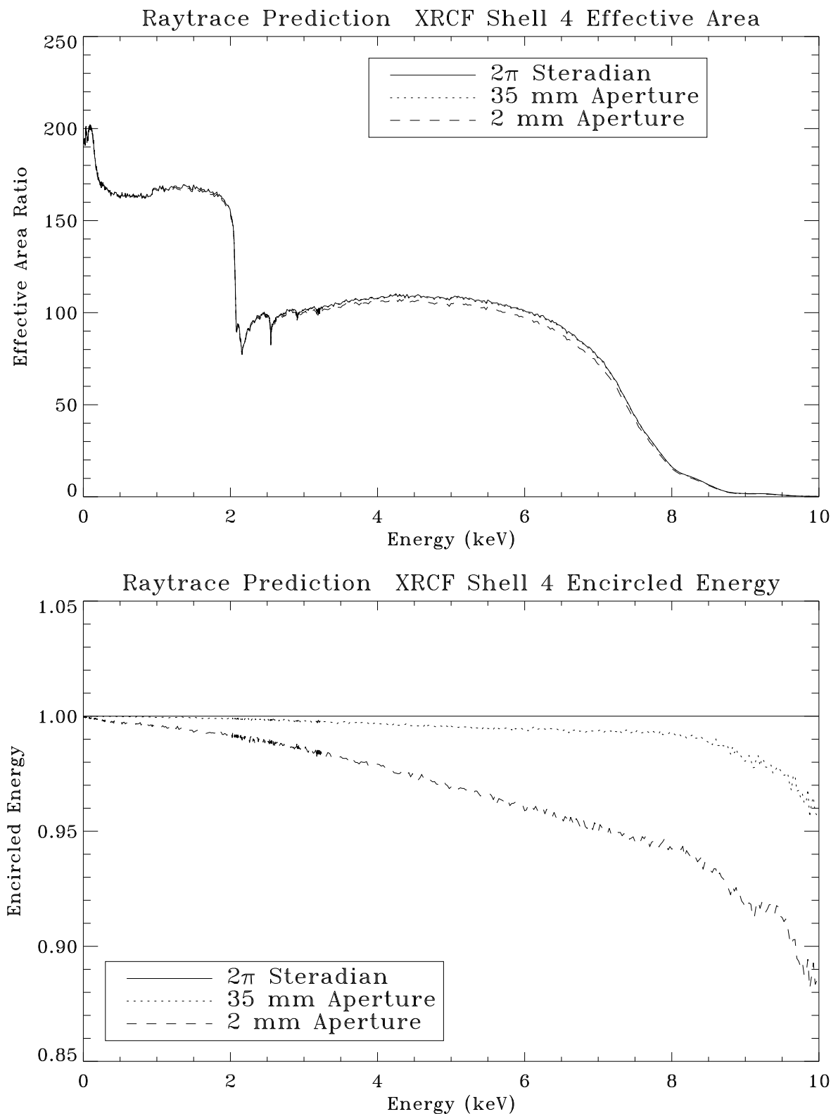
Figure 11.43: Raytrace prediction of XRCF Shell 4 effective area and encircled energy. Top panel shows the effective area curves within 2 mm, 35 mm apertures, and 2\pi steradian. Bottom panel shows the encircled energies of 2 mm and 35 mm apertures as fractions of that within 2\pi steradian.
