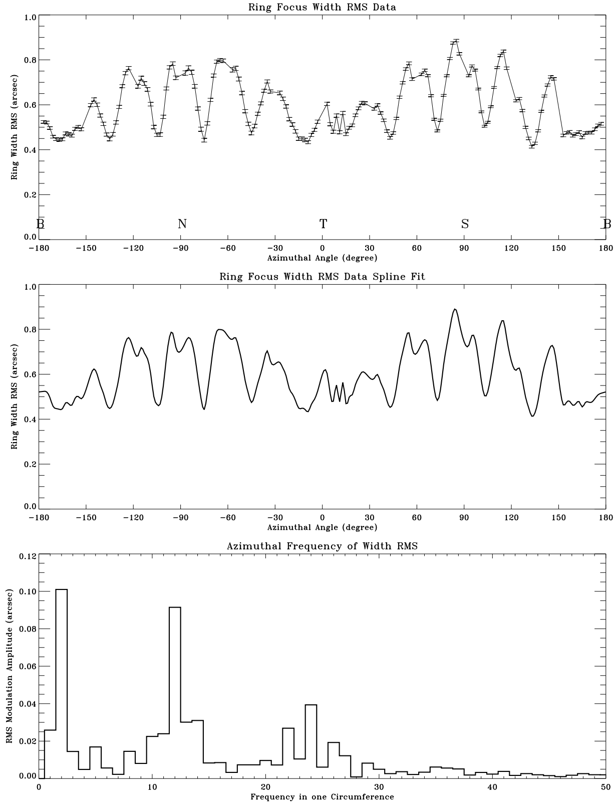
Figure 18.11: The Ring width RMS for ring 1. Date: 1997/01/24; TRW ID: D-IXH-RF-1.005; Run ID: 110004; Source: A1-K; Defocus: 65.2 mm.
