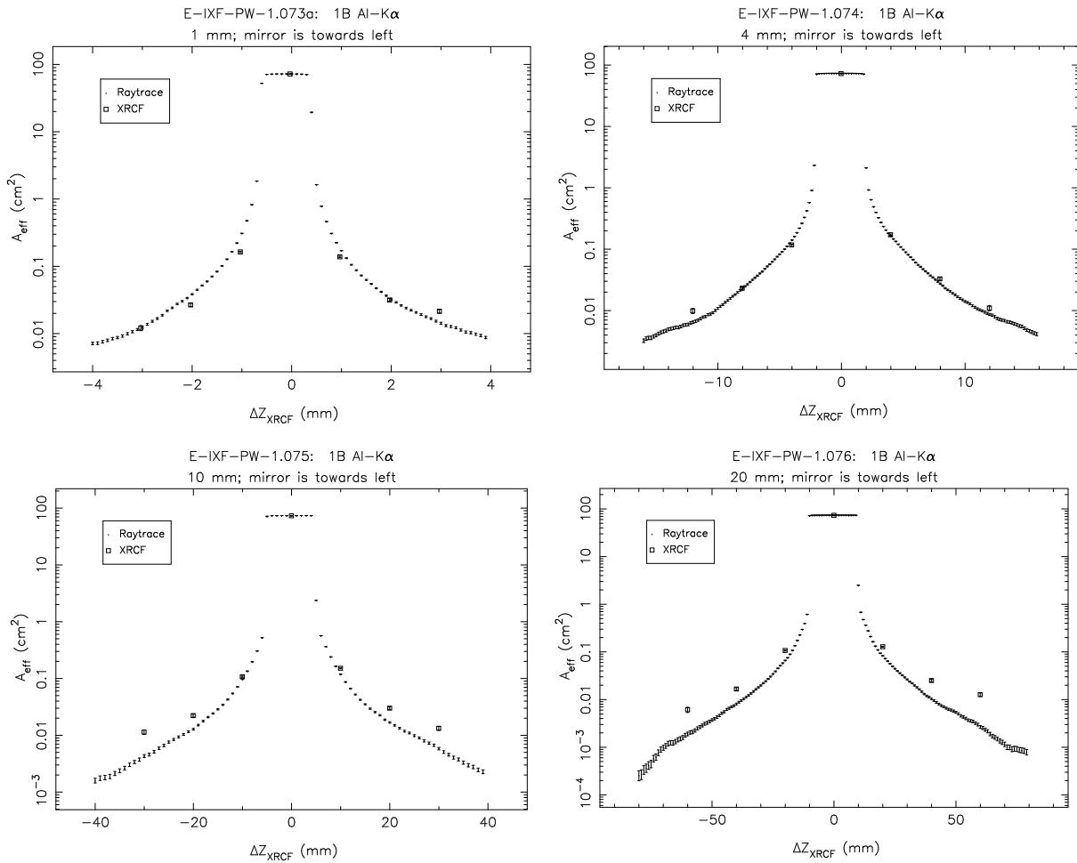
Figure 14.6: Pinhole effective areas; Shell 1B at Al-K \alpha .
