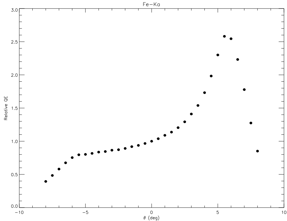
Figure 7.1: (continued) Fe-K.
