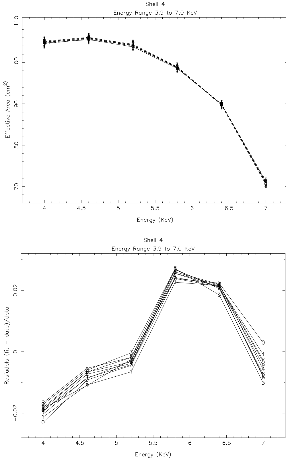
Figure 13.21: SSD continuum data and model effective area and residuals through 2mm pinhole for shell 4 between 3.9 and 7.0 keV.
