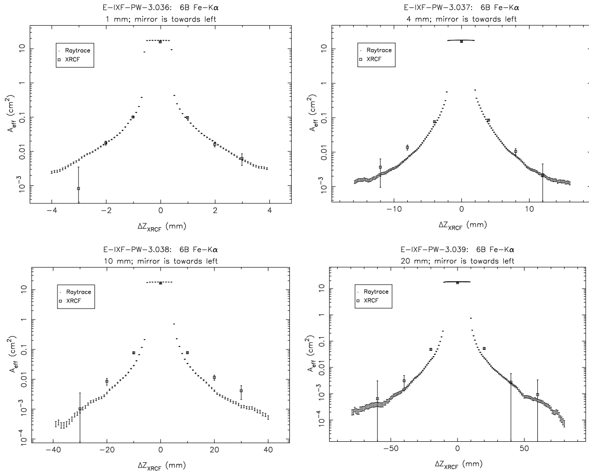
Figure 14.41: Pinhole effective areas; Shell 6B at Fe- \text{K}\alpha .
