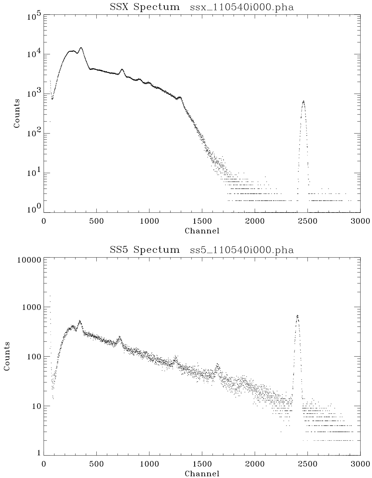
Figure 11.2: C-continuum SSX and SS5 spectra: Shell 3; Date: 970130; TRW ID: E-IXS-MC-15.002; Run ID: 110540; Aperture: 2 mm; Integration time: 1000 seconds.
