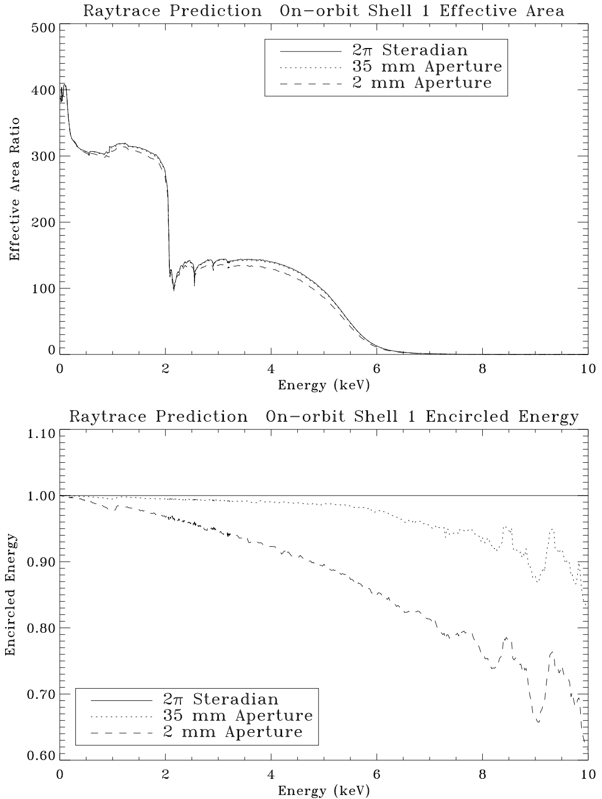
Figure 11.46: Raytrace prediction of on-orbit Shell 1 effective area and encircled energy. Top panel shows the effective area curves within 2 mm, 35 mm apertures, and 2\pi steradian. Bottom panel shows the encircled energies of 2 mm and 35 mm apertures as fractions of that within 2\pi steradian.
