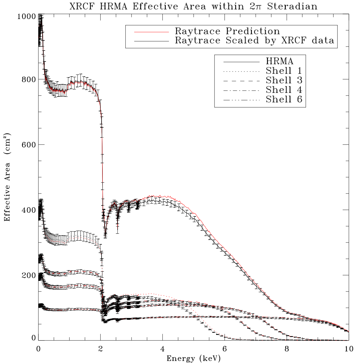
Figure 11.53: The XRCF HRMA and four shells effective areas within 2\pi steradian. The original raytrace predictions and the calibration data scaled raytrace predictions.
