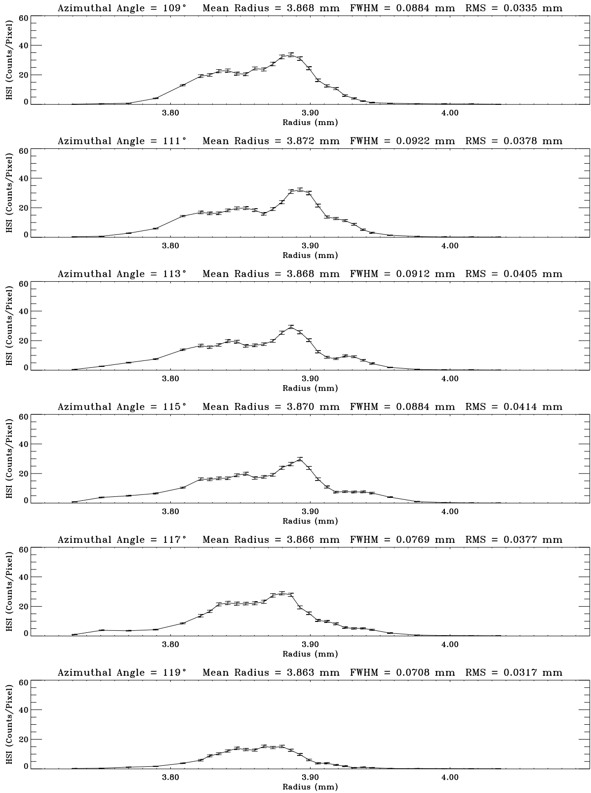
Figure 18.10: Radial profiles for ring 1. Date: 1997/01/24; TRW ID: D-IXH-RF-1.005; Run ID: 110004; Source: Al-K; Defocus: 65.2 mm.
