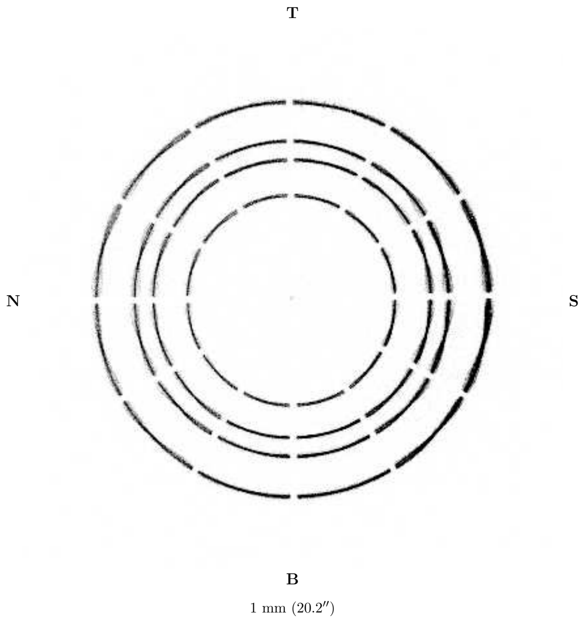
Figure 18.1: The HRMA ring focus HSI image. Date: 1996/12/23; TRW ID: C-IXH-RF-1.005; Run ID: 106856; Source: A1-K; Defocus: 65.2 mm; Integration time: 1800 seconds.
