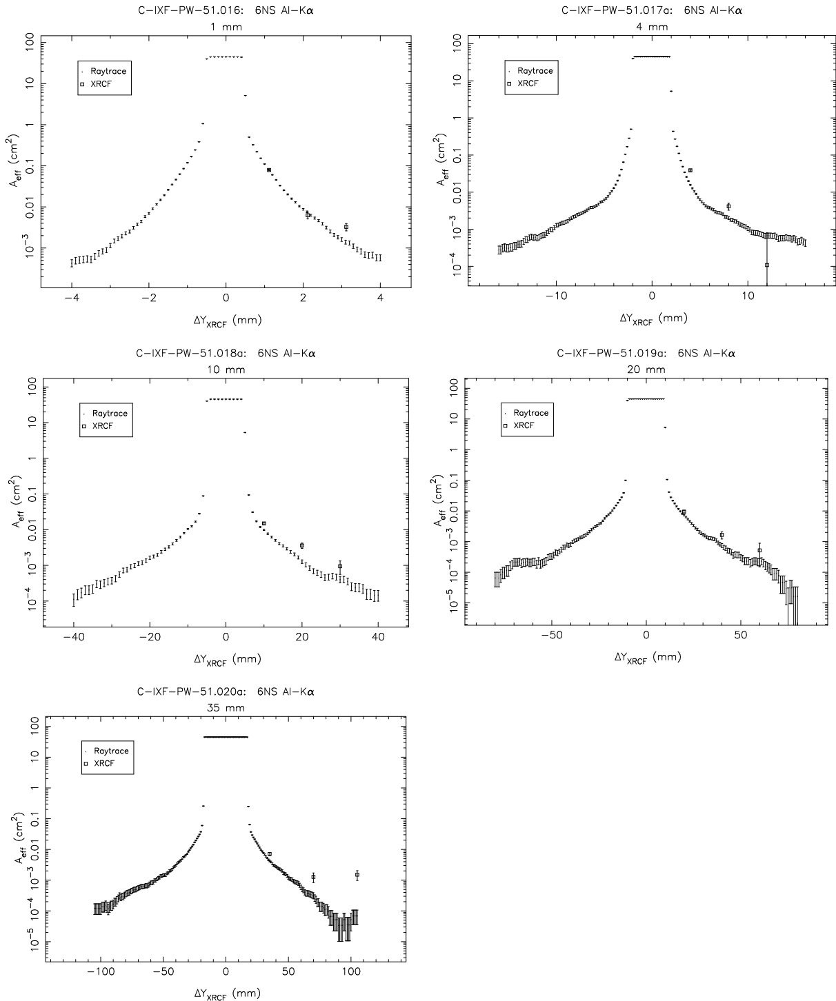
Figure 14.50: Pinhole effective areas; Shell 6NS at \text{Al-K}\alpha .
