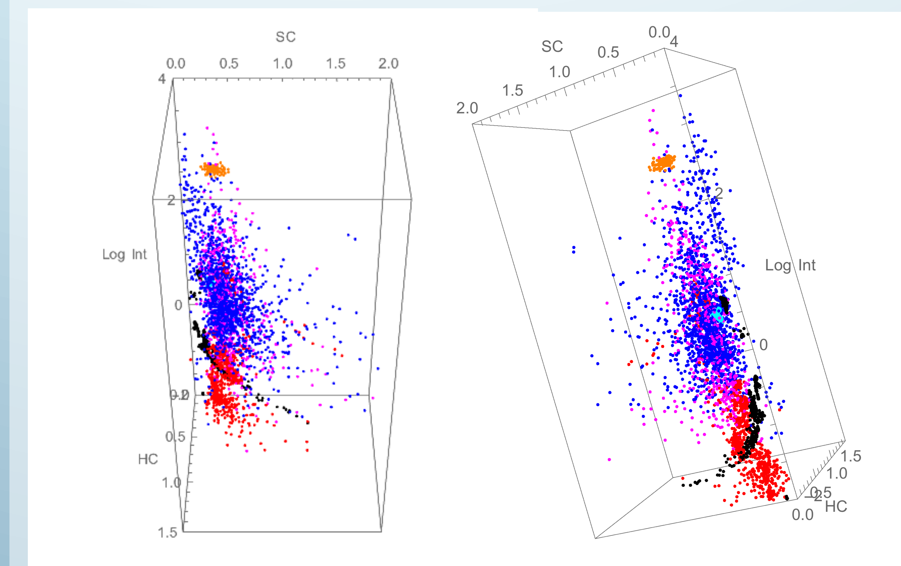
Figure 3. Two views of a CCI plot of Chandra point sources from 62 early (blue) and 13 late (magenta) galaxies together with Chandra observations of 20 X-ray binaries (black holes in black, non-pulsing neutron stars in cyan, and X-ray pulsars in red). Plotted are cts/sec at a standardized distance of 1 Mpc. Also (in orange) are Chandra data of the ULX M82 X-1.
