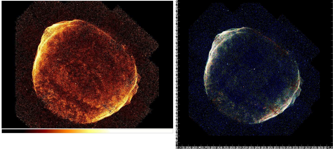
Figure 1. An exposure-corrected composite mosaic image from 11 separate Chandra ACIS observations of the supernova remnant SN1006. In the right panel the image is displayed in “true” colors (where color correlates with energy) obtained from the ACIS energy bands. Blue represents non-thermal emission above 2.5 keV while red represents thermal emission below 1.5 keV. Several CIAO tools were used to create these images and in particular the tools reproject_image_grid and reproject_image which allow a user to project images to common coordinate systems and aconvolve and dmimg2jpg used to create the smoothed three-color image.
