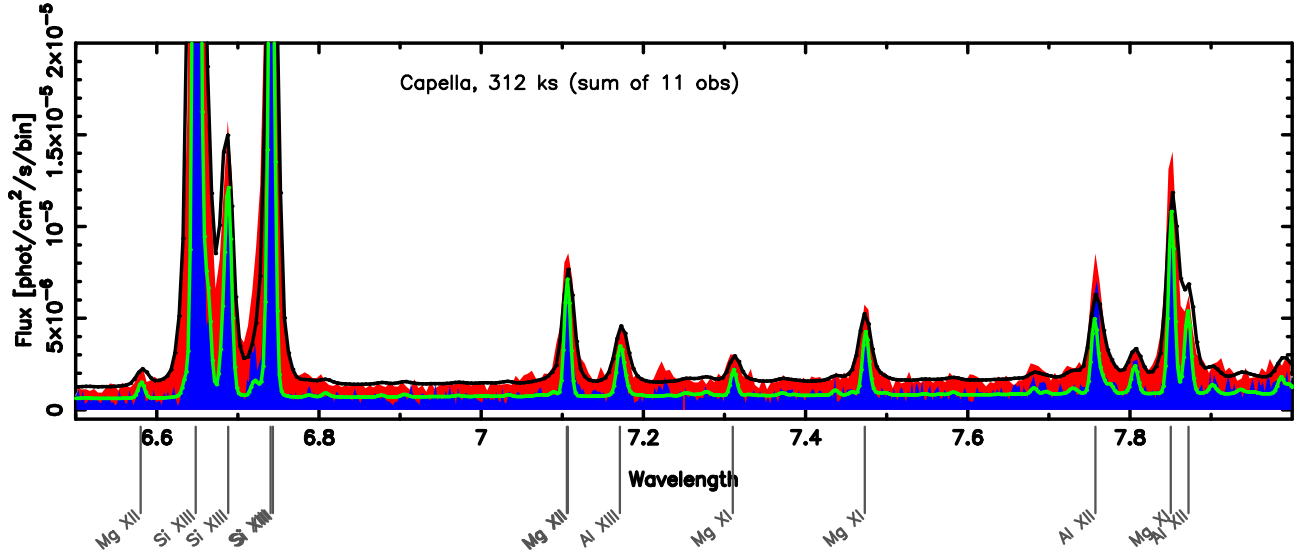
Figure 2. This shows a small portion of the High Energy Transmission Grating Spectrometer (HETGS) flux-calibrated spectrum of the star Capella, from the sum of 11 observations. The upper filled region (red) is from the Medium Energy Grating (MEG), and the lower (blue) is from the High Energy Grating (HEG) (HEG and MEG have different spectral resolutions and sensitivities). The solid lines outlining each region (black and green) are models derived from the atomic database (APED) convolved with the instrument responses. Line identifications are shown below the spectrum. Each individual observation and calibration were computed with standard CIAO tools, velocities and wavelength shifts computed with custom S-Lang programs, and spectra were combined and displayed with ISIS.
