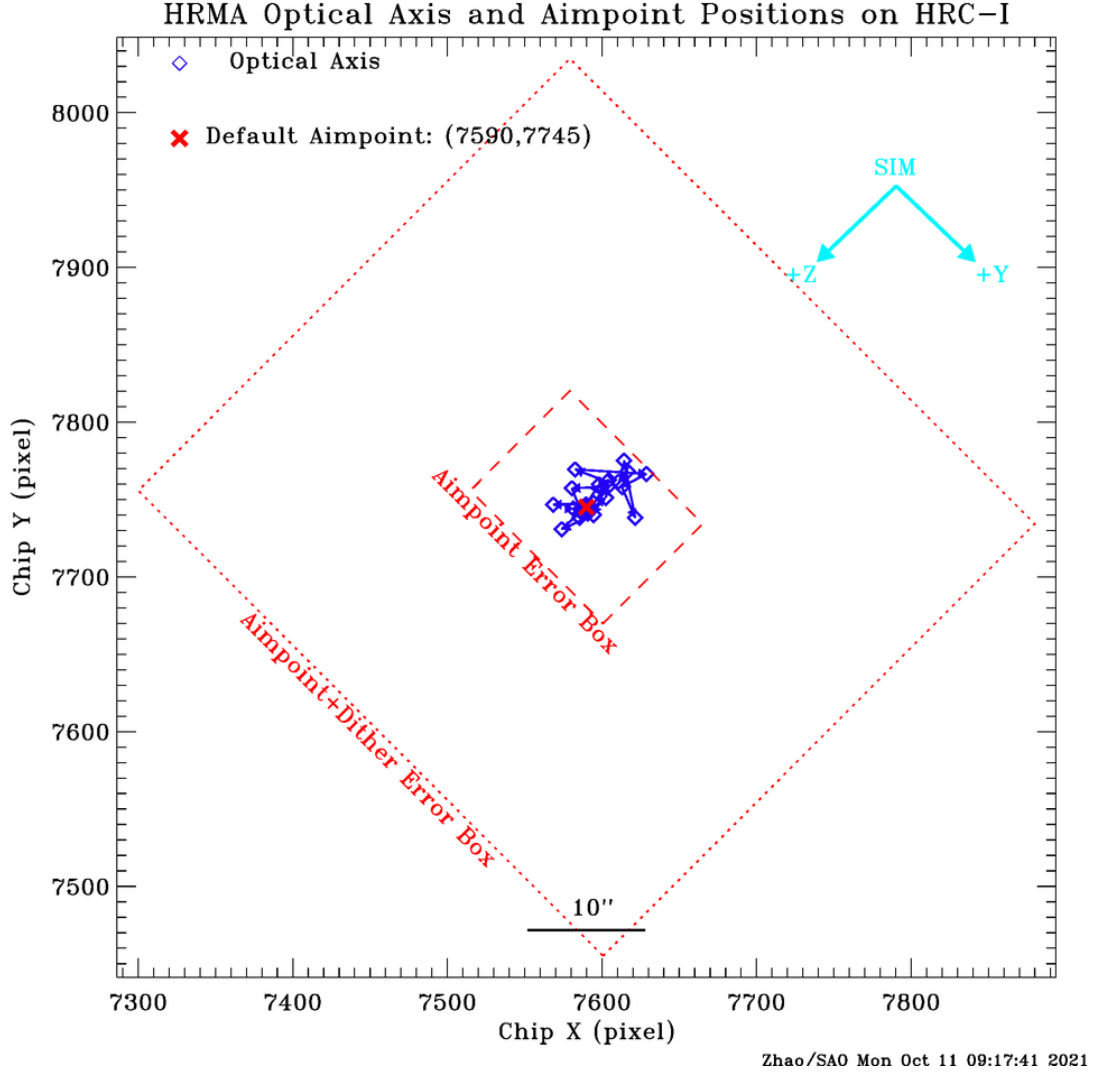
Figure 4.32: Chandra optical axis (blue diamonds) positions for each year and permanent default aimpoint (red cross) on HRC-I at [7590,7745]. The small box (red dashed line, 16 arcsec \times 12 arcsec, or 121.4 \times 91.1 pixels in SIM [Y, Z]) centered at the permanent default aimpoint is the error box of the effective aimpoint center, i.e. an on-axis target can be anywhere inside this box. The large box (red dotted line, 56 arcsec \times 52 arcsec, or 425.0 \times 394.7 pixels in SIM [Y, Z]) is the error box of effective aimpoint with dither.
