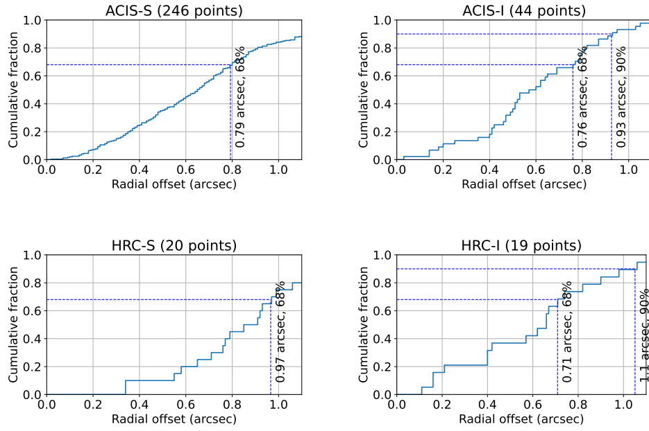
Figure 5.4: Cumulative histogram of celestial accuracy for Chandra X-ray source locations for each SI using observations since 2019-Oct. Radial offset is the distance in arcsec between the optical coordinate, typically from the Tycho-2 catalog, and the Chandra position.
