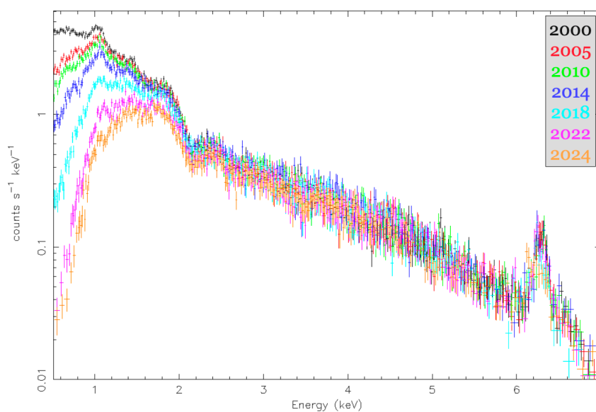
Figure 6.8: ACIS-S spectrum of the galaxy cluster Abell 1795 at seven different epochs ranging from 2000 to 2024. The decreasing count rates in the spectrum of a stable calibration source demonstrate the loss of effective area due to the build-up of the contaminant on the ACIS OBF.
