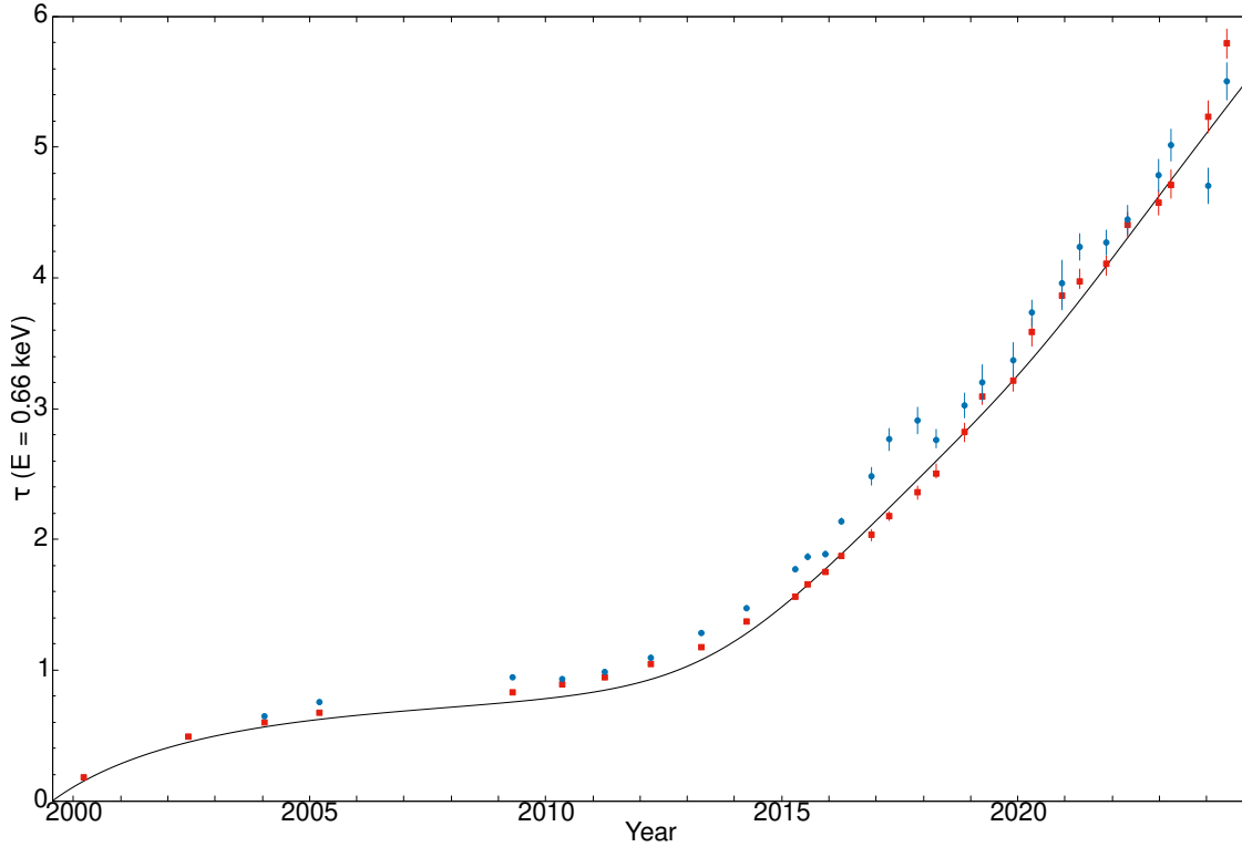
Figure 6.7: Optical depth of the contaminant measured at 0.66 keV from observations of the galaxy cluster Abell 1795. Red squares denote observations with the target on ACIS-S and blue disks denote observations with the target on ACIS-I. The solid curve shows the optical depth of the contaminant as modeled in the most recent contamination model.
