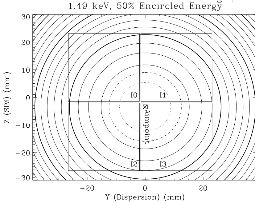
Figure 6.17: Approximate contours of constant 50% encircled energy at 1.49 keV when the ACIS-I aimpoint is selected. The dotted circle is 1 arcsec. That is, the 50% encircled energy at 1.49 keV at any point on the dotted circle is 1 arcsec. Similarly, the dashed circle is 1.5 arcsec. The remainder are at 1 arcsec intervals. The thicker solid circles highlight the 5, 10, and 15 arcsec contours.
