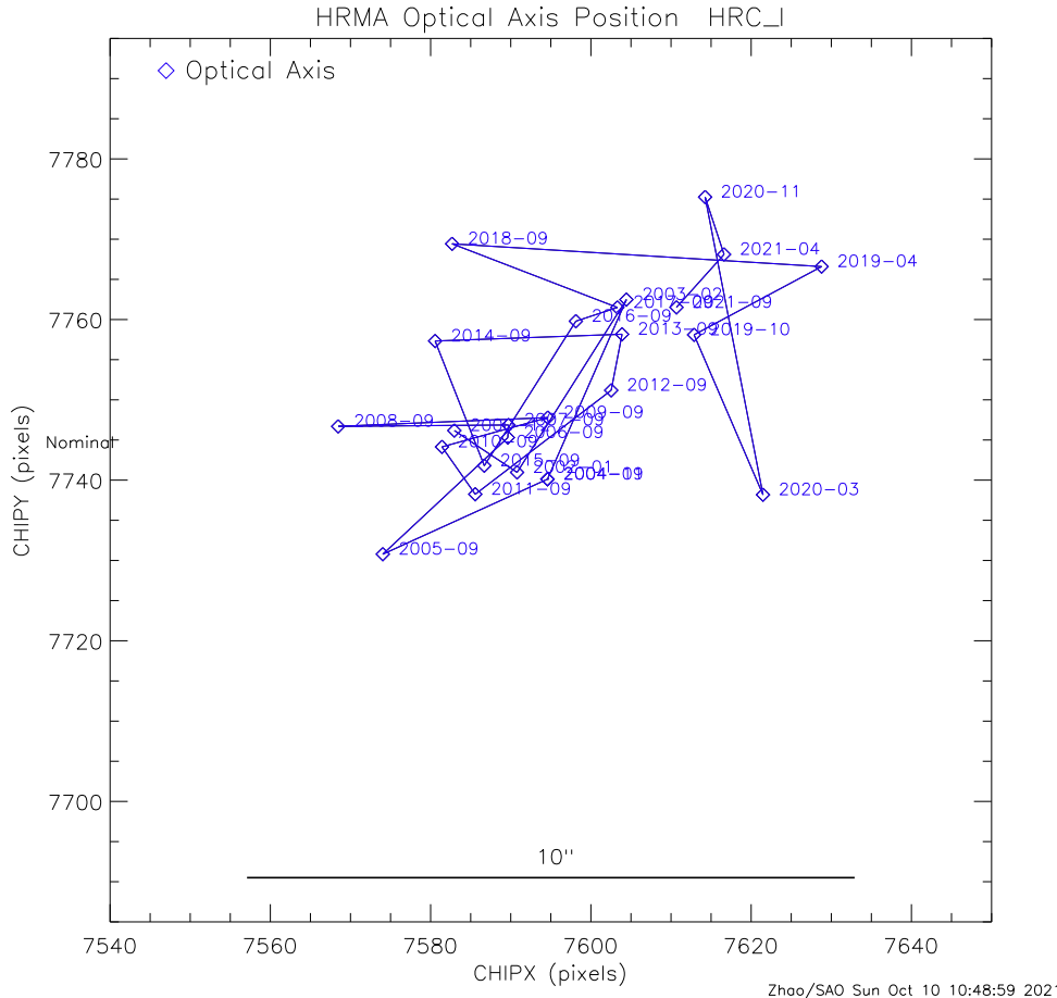
Figure 4.26: Chandra optical axis positions on HRC-I since launch. Each position is labeled by the year-month. The optical axis position is very stable and well within a 10 arcsec region.
