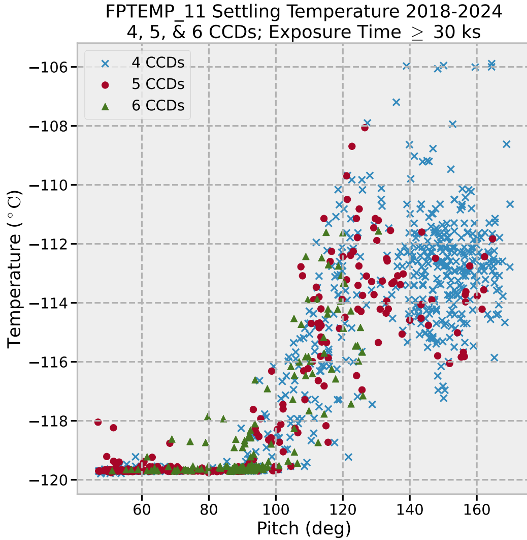
Figure 6.38: ACIS FP temperature as a function of spacecraft pitch angle. 6 CCD observations are indicated by green-filled triangles, 5 CCD observations by red-filled circles and 4 CCD observations are indicated by blue \times s.
