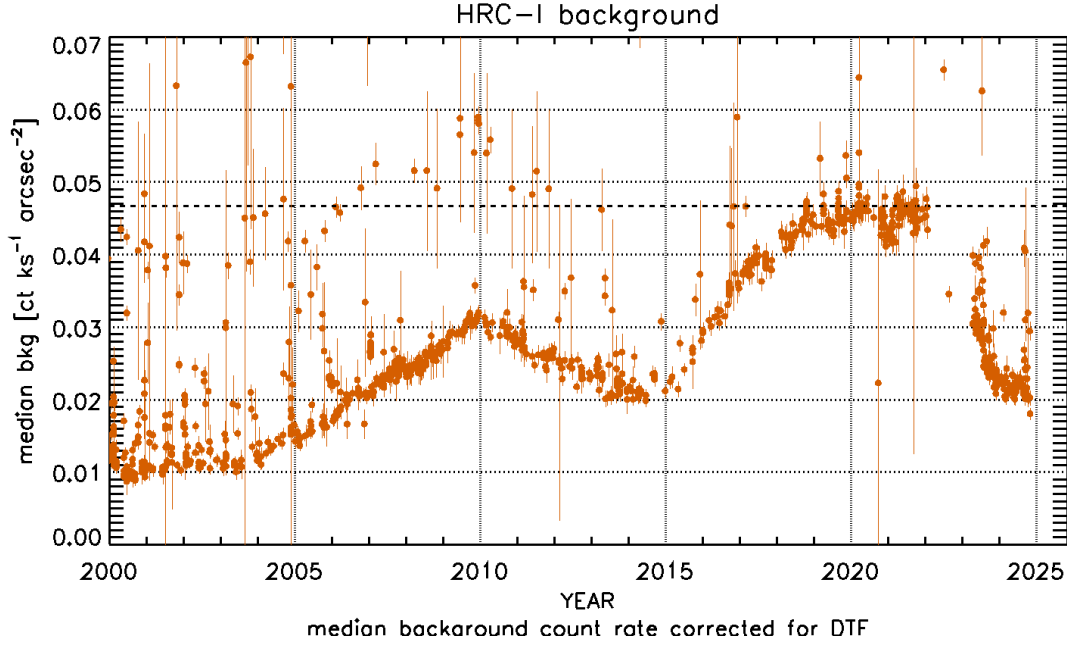
Figure 7.13: The change in HRC-I background rate with time. The deadtime corrected detector averaged counts per ksec per square arcsec is shown with error bars for each HRC-I observation. The lower envelope represents the quiescent rate, and the fluctuations are due to the occasional background flaring. The HRC-S data show a similar trend.
