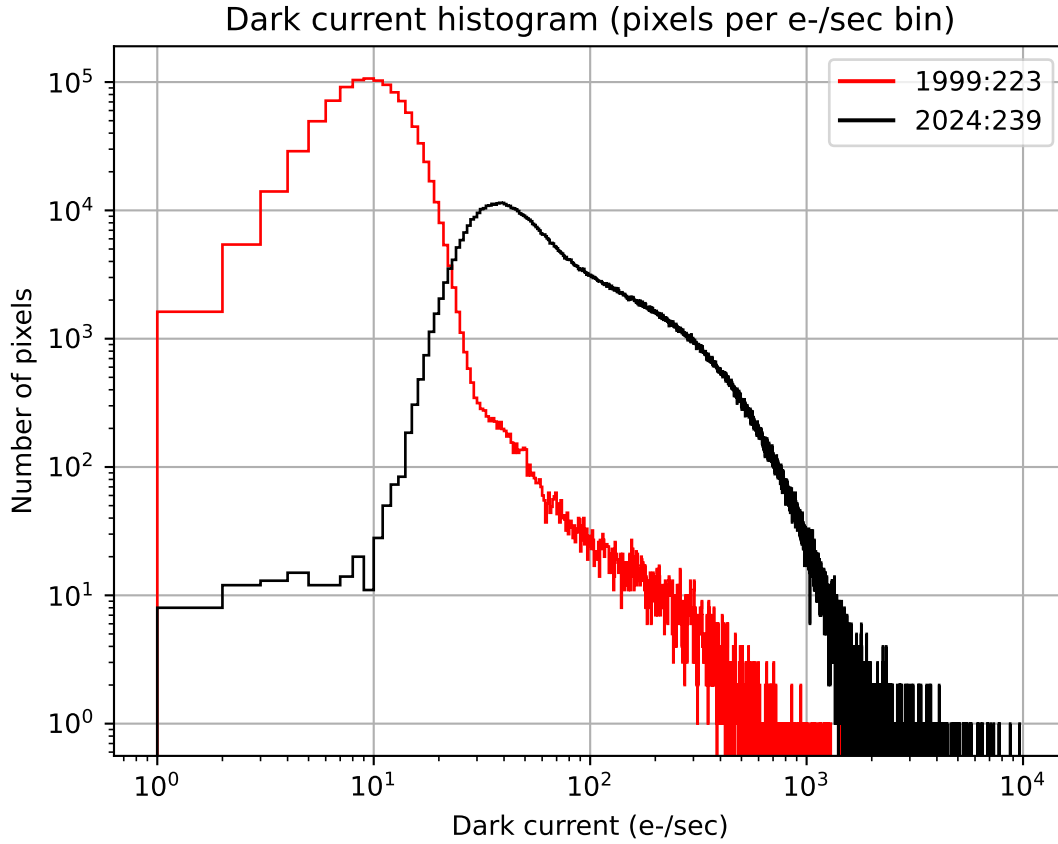
Figure 5.8: Differential histogram of dark current distribution for the ACA CCD on 1999-Aug-11 and 2024-Aug-26.
