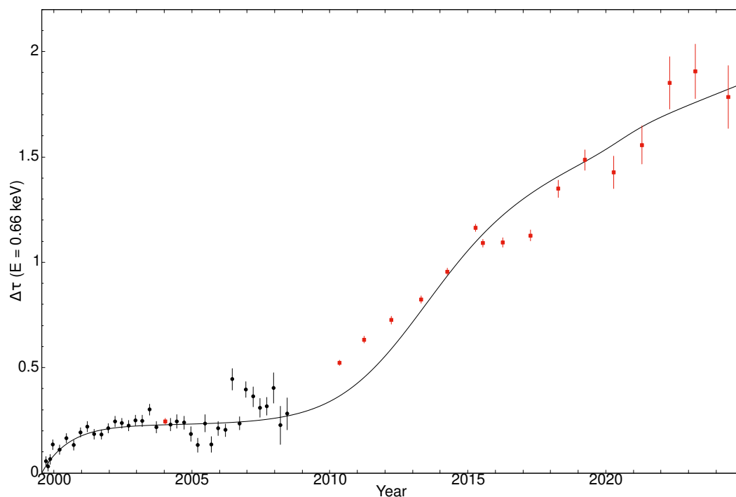
Figure 6.9: The difference between the optical depth at 0.66 keV measured near the center of the ACIS-S chip S3 and that measured near the readout at the edge of the same chip is shown against time. Black circles are measurements made using the ECS data and red squares are made from observations of the galaxy cluster Abell 1795. The solid curve shows the optical depth of the contaminant as modeled in the most recent contamination model.
