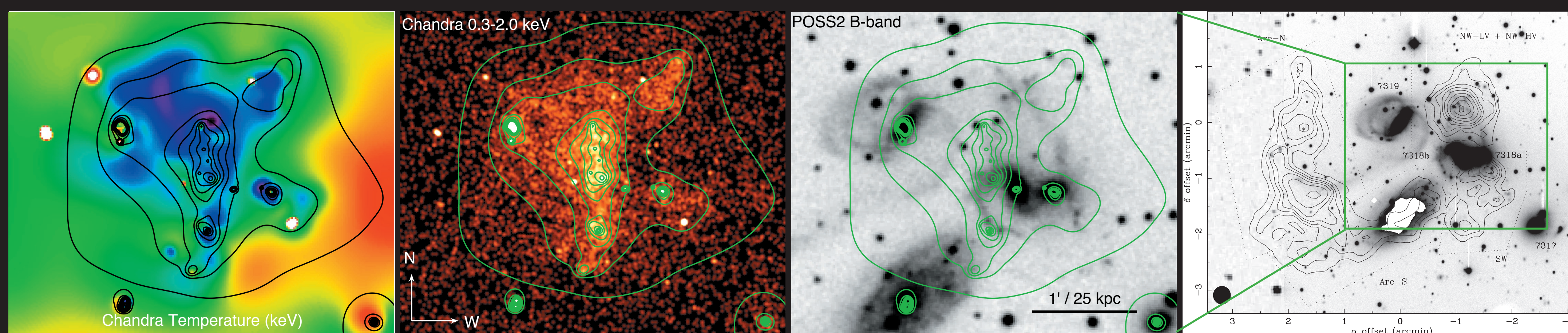
Exposure corrected 0.3-2.0 keV ACIS-S3 image, smoothed with a 3 pixel Gaussian. Adaptively smoothed contours overlaid.
