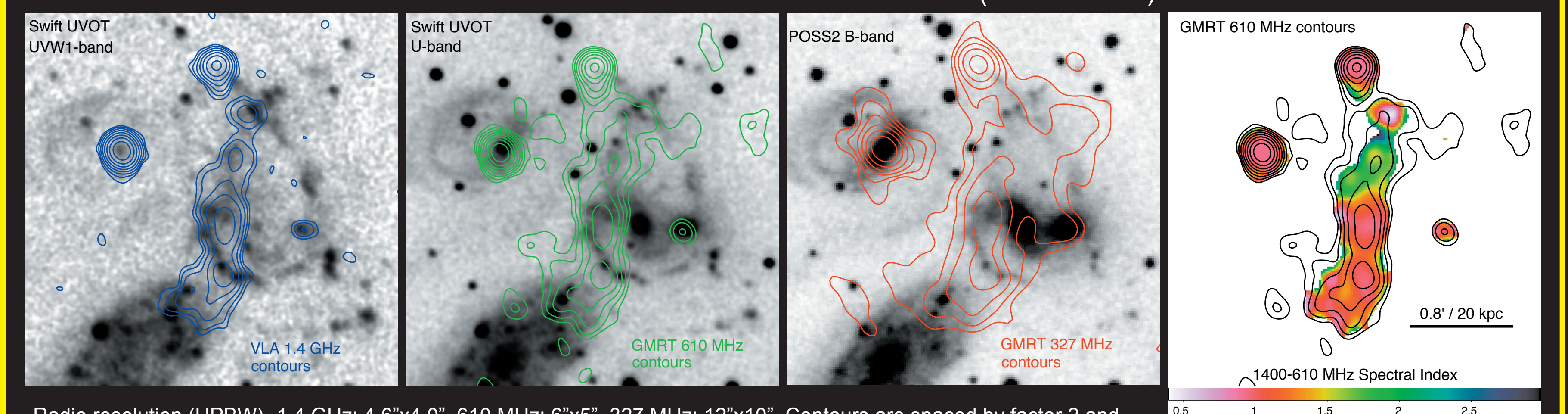
Radio resolution (HPBW)- 1.4 GHz: 4.6'' \times 4.0'' , 610 MHz: 6'' \times 5'' , 327 MHz: 12'' \times 10'' . Contours are spaced by factor 2 and start at 3\sigma above the r.m.s. noise level - 0.09 mJy/b for 1.4 GHz, 0.36 mJy/b for 610 MHz and 0.9 mJy/b for 327 MHz.
